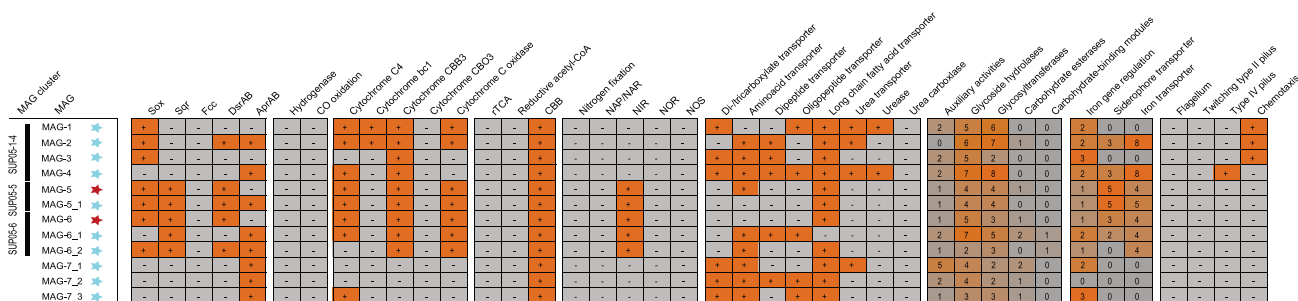
Fig. 4 Metabolic potential of SUP05-related MAGs. Bacterial genomes were manually screened for genes for: sulfur metabolism (Sox sulfur oxidizing enzyme, Sqr sulfide:quinone oxidoreductase, Fcc flavocytochrome c, Dsr dissimilatory sulfite reductase, Apr dissimilatory adenylylsulfate reductase), hydrogen oxidation and carbon monoxide oxidation, carbon fixation pathways (rTCA reverse tricarboxylic acid cycle, reductive acetyl-CoA, CBB Calvin Benson Bassham cycle), nitrogen fixation and nitrogen reduction (NAP nitrate reductase NIR nitrite reductase, NOR nitric oxide reductase, NOS nitrous oxide reductase), transporters, carbohydrate-active enzymes and lastly motility genes. MAGs with more than 95% ANI between each other are clustered together: SUP05-1-4 (MAG-1 to -4); SUP05-5 (MAG-5 and MAG 5_1); SUP05-6 (MAG-6, MAG-6_1 and MAG-6_2). MAGs retrieved from single assemblies are marked with a blue star and those resulting from a cross-assembly with a red star. The presence of genes is marked with a plus in an orange table cell, whereas the absence is marked with a minus in a gray cell. The presence of the carbohydrate-active enzymes and iron-related genes is given as a heatmap based on the number of these genes.
