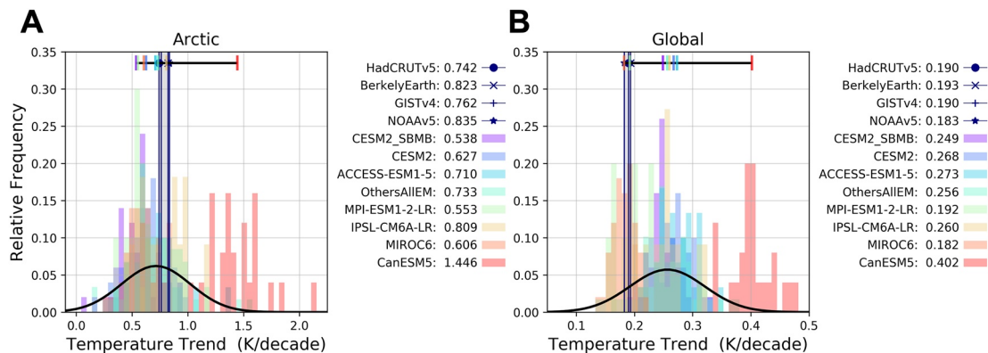
Figure 2. Surface air temperature trends over 1980–2022 for the (a) Arctic and (b) global mean. The histograms show the distributions from model simulations, and the vertical lines represent the observations where gray shading shows their range. The black curve shows a normal distribution fitted to all the simulated temperature trends. The horizontal black line shows the range of externally forced trends with ticks showing individual models' forced trends. The trend values from individual observational data sets and forced trend values from individual models are provided in the legend.
