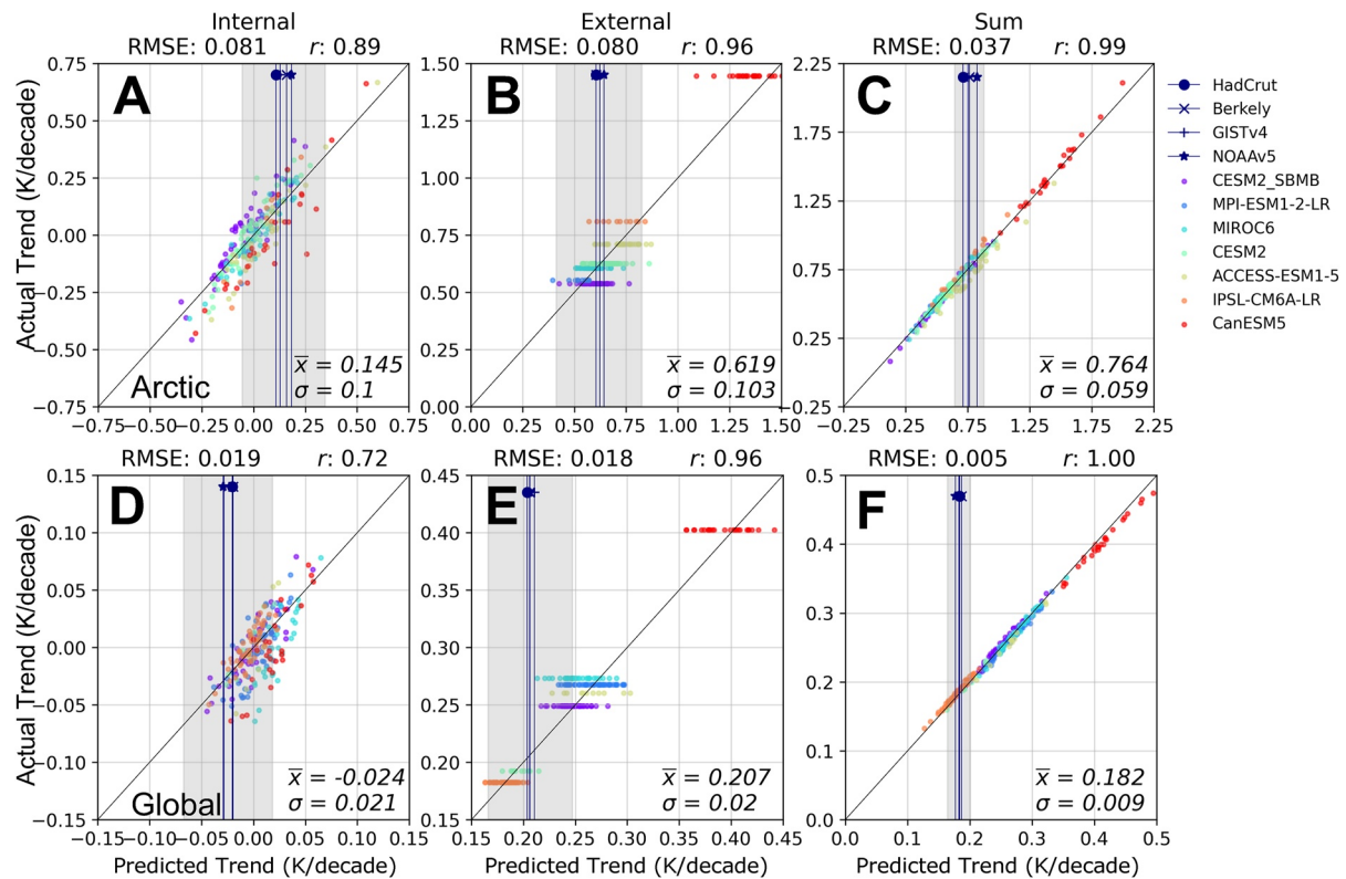
Figure 3. (a)–(c) Arctic and (d)–(f) global surface air temperature trends predicted from the CNN ( x -axis) versus corresponding actual trends ( y -axis) over 1980–2022. The root mean squared error (RMSE) and correlation coefficient ( r ) are shown at the top of each plot. Panels (a), (d) shows results for internally generated trends, (b), (e) shows the externally forced trends, and (c), (f) shows the sum of the internally generated and externally forced trends. The vertical lines show the mean observational estimate for each temperature record, and the gray shading shows the \pm 2\sigma uncertainty of mean prediction. The mean ( \bar{x} ) and its standard deviation ( \sigma ) based on observations are provided in the bottom right of each plot. The black diagonal line in (a)–(f) is the 1:1 line.
