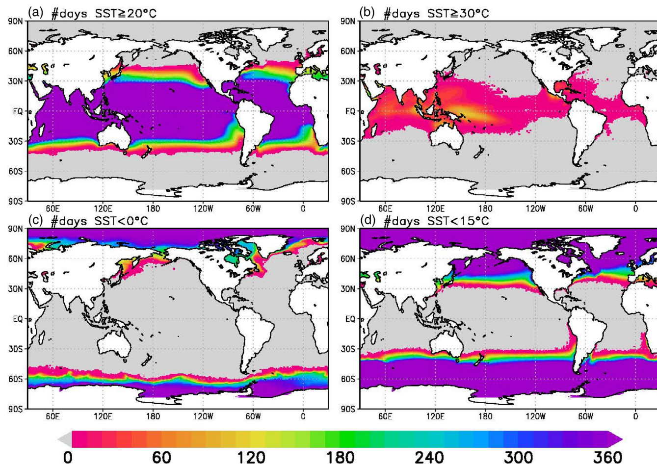
FIGURE 5 Annual normal SST count (units: days) for the number of days with SST (a) \geq 20^{\circ}\text{C} , (b) \geq 30^{\circ}\text{C} , (c) < 0^{\circ}\text{C} and (d) < 15^{\circ}\text{C} . [Colour figure can be viewed at wileyonlinelibrary.com ]
