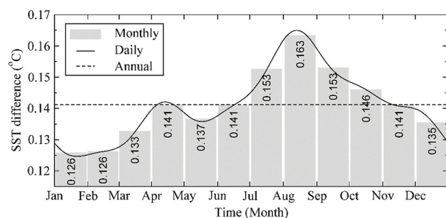
FIGURE 12 Global mean SST difference between the two climatologies (1991–2020 minus 1982–2011) at annual, monthly and daily scales. [Colour figure can be viewed at wileyonlinelibrary.com ]
