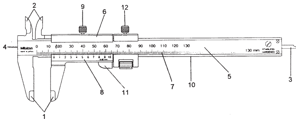
Figure 27. Vernier calipers.
