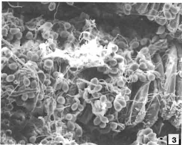
Figure 3.—Scanning electron micrograph of a secondary gill rachis of a blue shrimp, P. stylirostris , that is heavily infested with colonies of the colonial peritrich Zoothamnium sp. Also present are filaments of Leucothrix mucor and a few diatoms. x 199.
