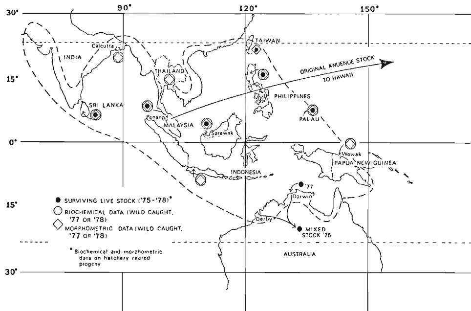
Figure 13.—Native distribution of Macrobrachium rosenbergii showing geographic origin of the Anjuene stock and areas visited in a field survey. Small closed circles refer to areas from which imported founders have been used to develop parental and hybrid progeny. Large open circles represent populations which were analyzed electrophoretically (i.e., biochemically). Diamond symbols represent areas visited from which morphometric data was obtained.
