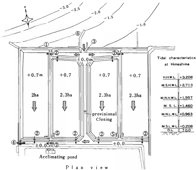
Figure 9.—Plan view of Himeshima shrimp culture pond.
