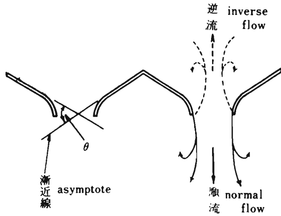
Figure 8.—Configuration of a training dyke.
