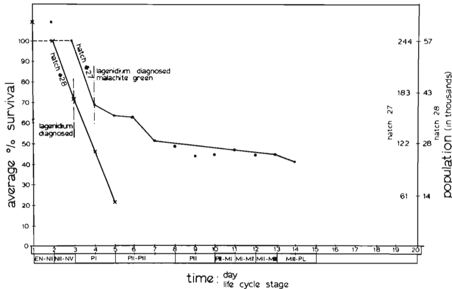
Figure 6.—Survival plots of larval blue shrimp, Penaeus stylirostris , populations in which disease due to Lagenidium callinectes was epizootic. The population designated as ‘‘hatch 27’’ was treated with malachite green upon detection of the presence of Lagenidium , while the population labeled ‘‘hatch 28’’ was not. The epizootic in hatch 27 was arrested with nearly a 50% survival rate, while the untreated hatch 28 had nearly 100% mortality.
