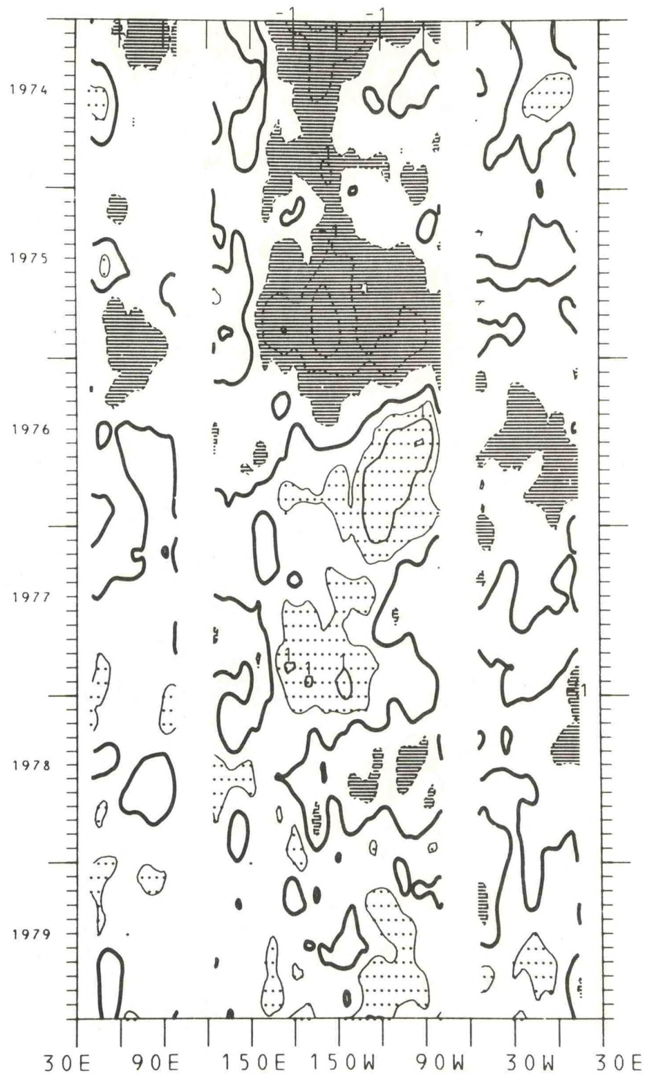
Figure 97. Time-longitude cross-section of equatorial SST anomalies for the years 1974-1979. The contour interval is .5^{\circ}\text{C} . The zero isotherm is emphasized. Negative values are dashed. Light shading is greater than 0.5^{\circ}\text{C} ; dark shading is less than -0.5^{\circ}\text{C} .
