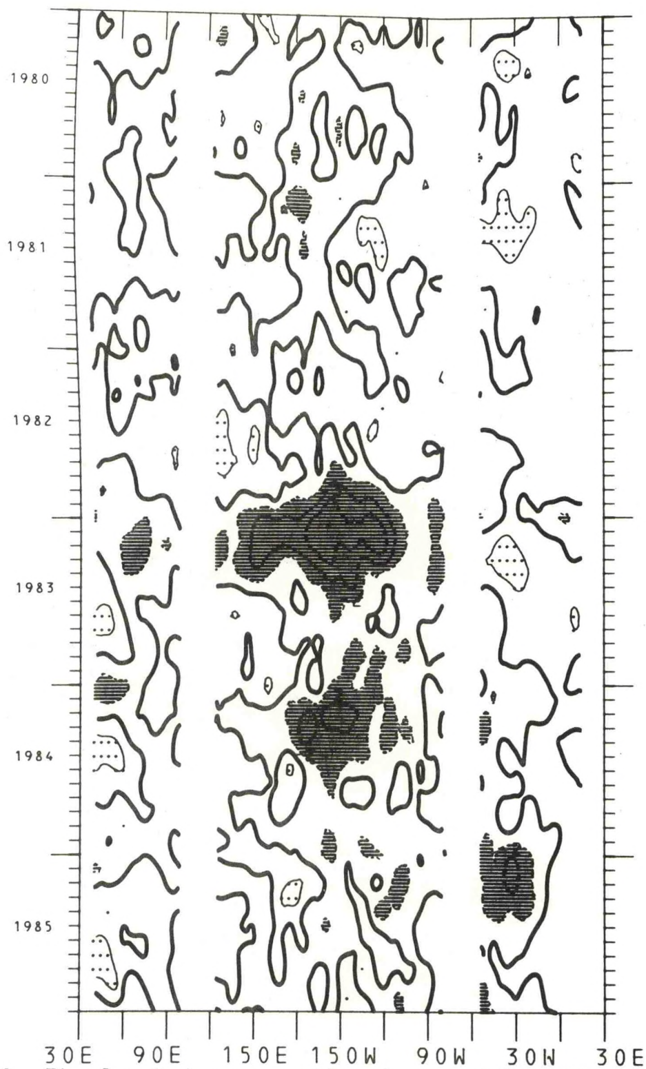
Figure 142. Time-longitude cross-section of equatorial meridional wind component anomalies for the years 1980-1985. The contour interval is 1.0 m/s. The zero isotherm is emphasized. Light shading is greater than 1.0 m/s; dark shading is less than -1.0 m/s.
