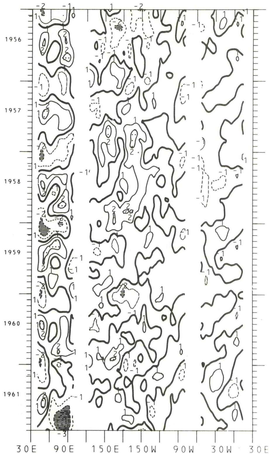
Figure 123. Time-longitude cross-section of equatorial zonal wind component expressed as the difference from the annual mean for the years 1956-1961. The contour interval is 1.0 m/s. The zero isotherm is emphasized. Light shading is greater than 2.0 m/s; dark shading is less than -2.0 m/s.
