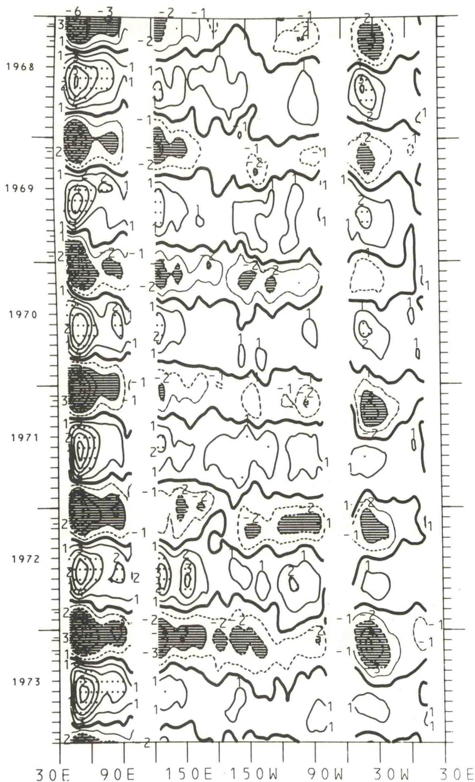
Figure 147. Time-longitude cross-section of equatorial meridional wind component expressed as the difference from the annual mean for the years 1968-1973. The contour interval is 1.0 m/s. The zero isotherm is emphasized. Light shading is greater than 2.0 m/s; dark shading is less than -2.0 m/s.
