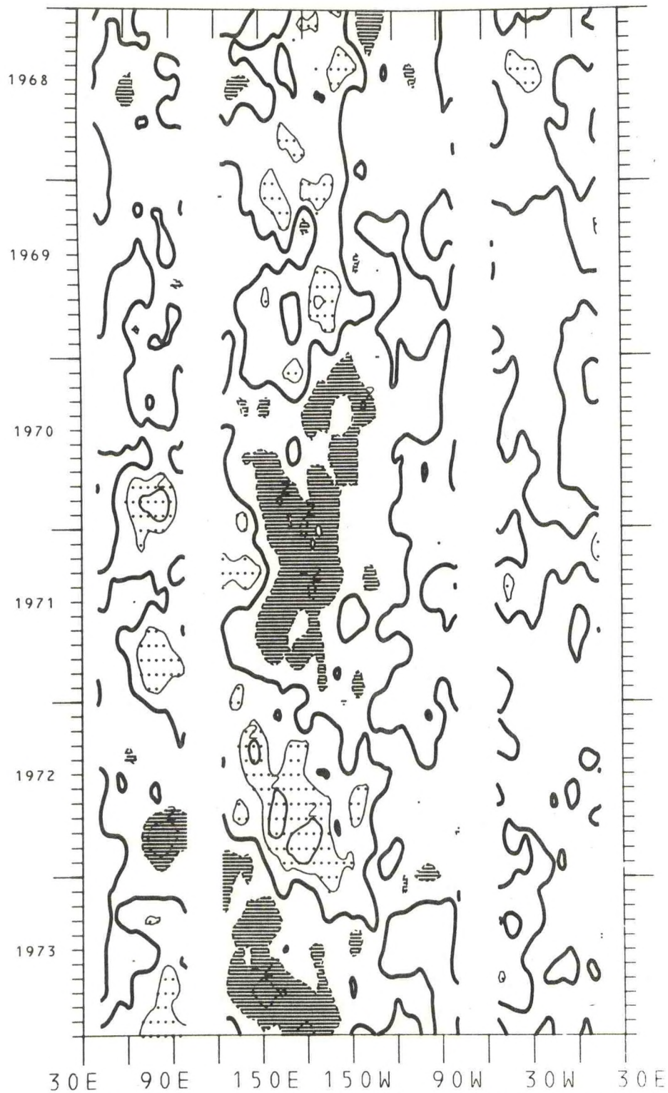
Figure 118. Time-longitude cross-section of equatorial zonal wind component anomalies for the years 1968-1973. The contour interval is 1.0 m/s. The zero isotherm is emphasized. Light shading is greater than 1.0 m/s; dark shading is less than -1.0 m/s.
