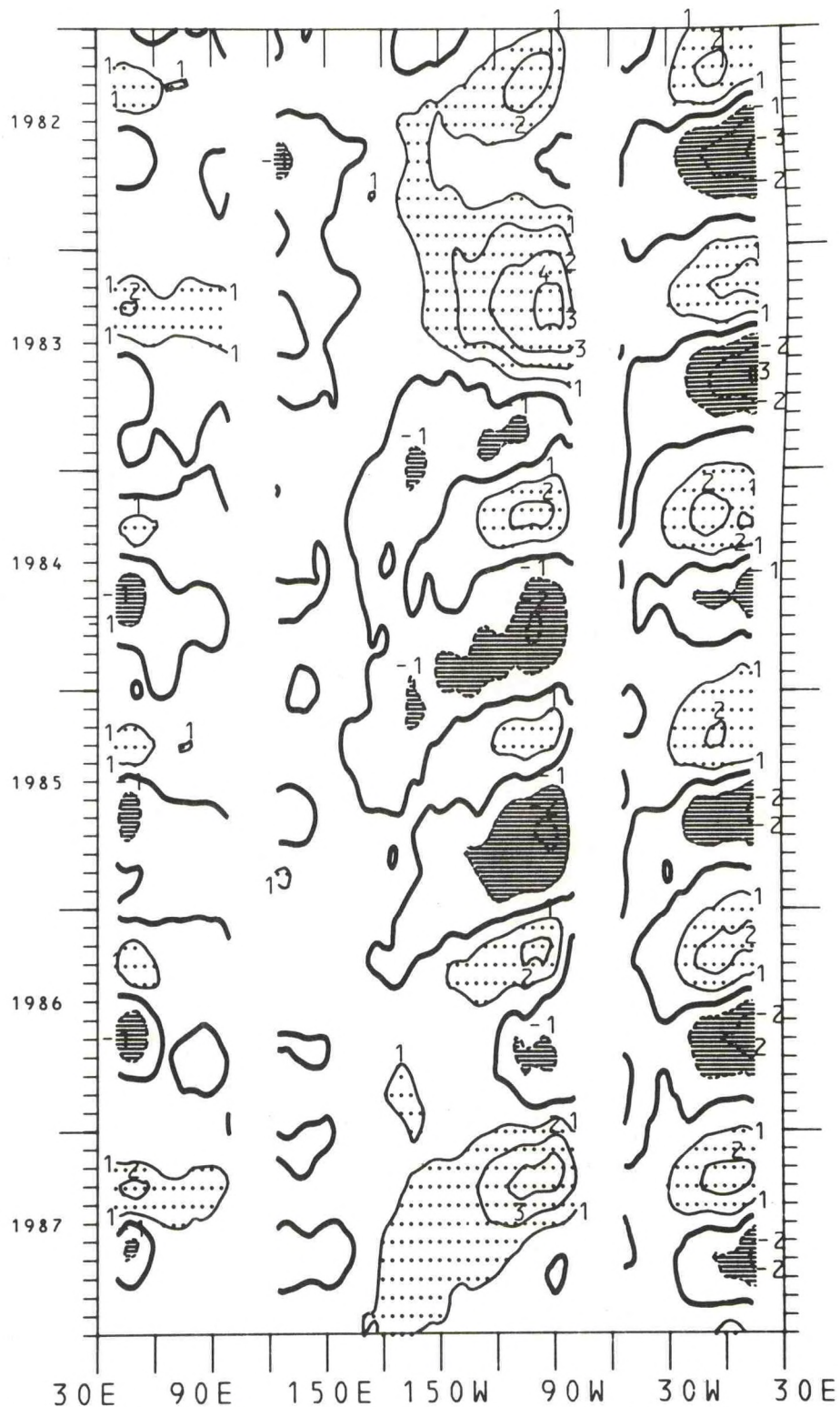
Figure 106. Time-longitude cross-section of equatorial SST expressed as the difference from the annual mean for the years 1982-1987. The contour interval is 1.0^{\circ}\text{C} . The zero isotherm is emphasized. Negative values are dashed. Light shading is greater than 1.0^{\circ}\text{C} ; dark shading is less than -1.0^{\circ}\text{C} .
