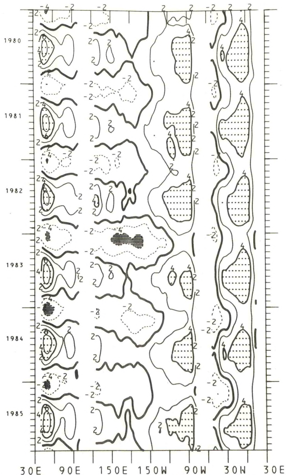
Figure 135. Time-longitude cross-section of the mean monthly equatorial meridional wind component for the years 1980-1985. The contour interval is 2.0 m/s. The zero isotherm is emphasized. Negative values (northerlies) are dashed. Light shading is greater than 4.0 m/s; dark shading is less than -4.0 m/s.
