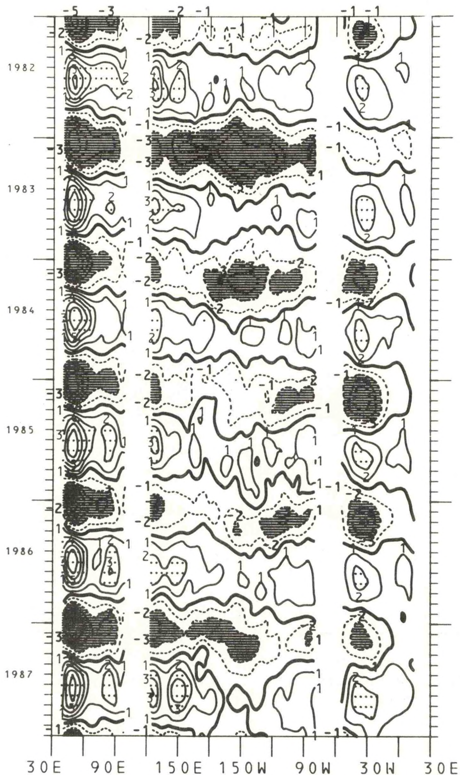
Figure 150. Time-longitude cross-section of equatorial meridional wind component expressed as the difference from the annual mean for the years 1982-1987. The contour interval is 1.0 m/s. The zero isotherm is emphasized. Light shading is greater than 2.0 m/s; dark shading is less than -2.0 m/s.
