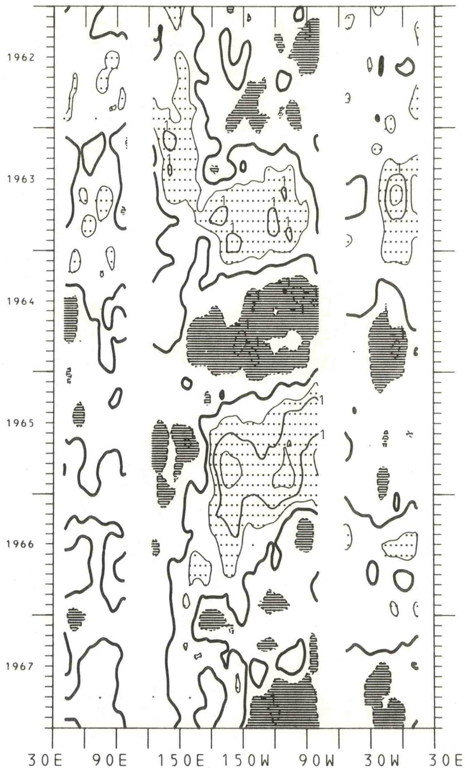
Figure 95. Time-longitude cross-section of equatorial SST anomalies for the years 1962-1967. The contour interval is .5^{\circ}\text{C} . The zero isotherm is emphasized. Negative values are dashed. Light shading is greater than 0.5^{\circ}\text{C} ; dark shading is less than -0.5^{\circ}\text{C} .
