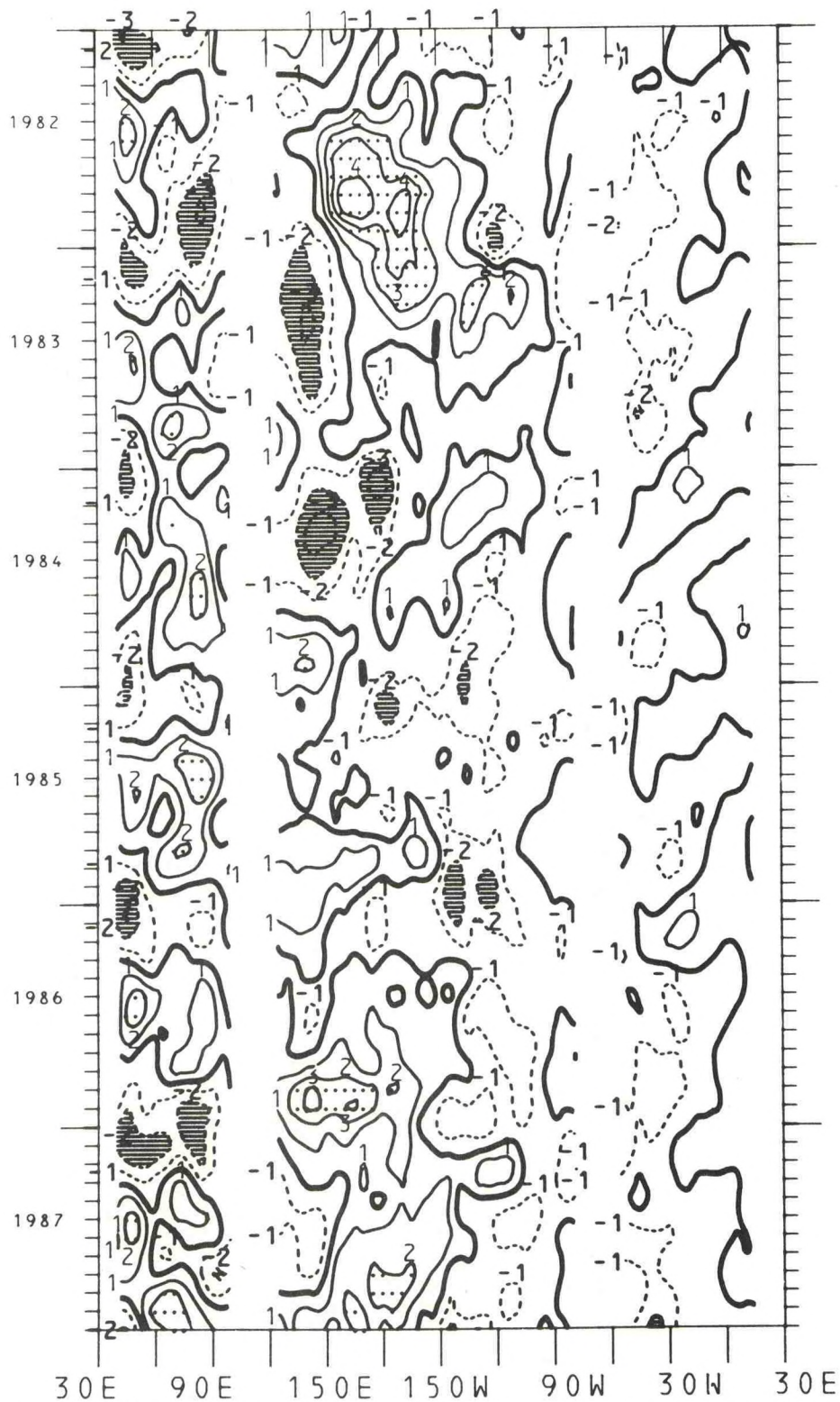
Figure 128. Time-longitude cross-section of equatorial zonal wind component expressed as the difference from the annual mean for the years 1982-1987. The contour interval is 1.0 m/s. The zero isotherm is emphasized. Light shading is greater than 2.0 m/s; dark shading is less than -2.0 m/s.
