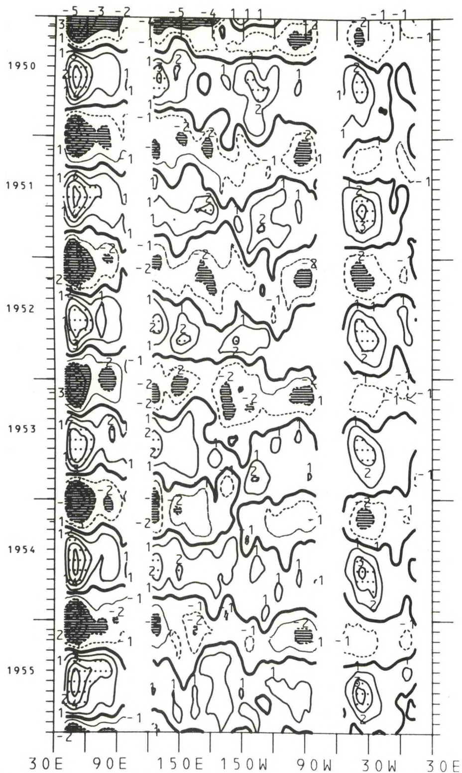
Figure 144. Time-longitude cross-section of equatorial meridional wind component expressed as the difference from the annual mean for the years 1950-1955. The contour interval is 1.0 m/s. The zero isotherm is emphasized. Light shading is greater than 2.0 m/s; dark shading is less than -2.0 m/s.
