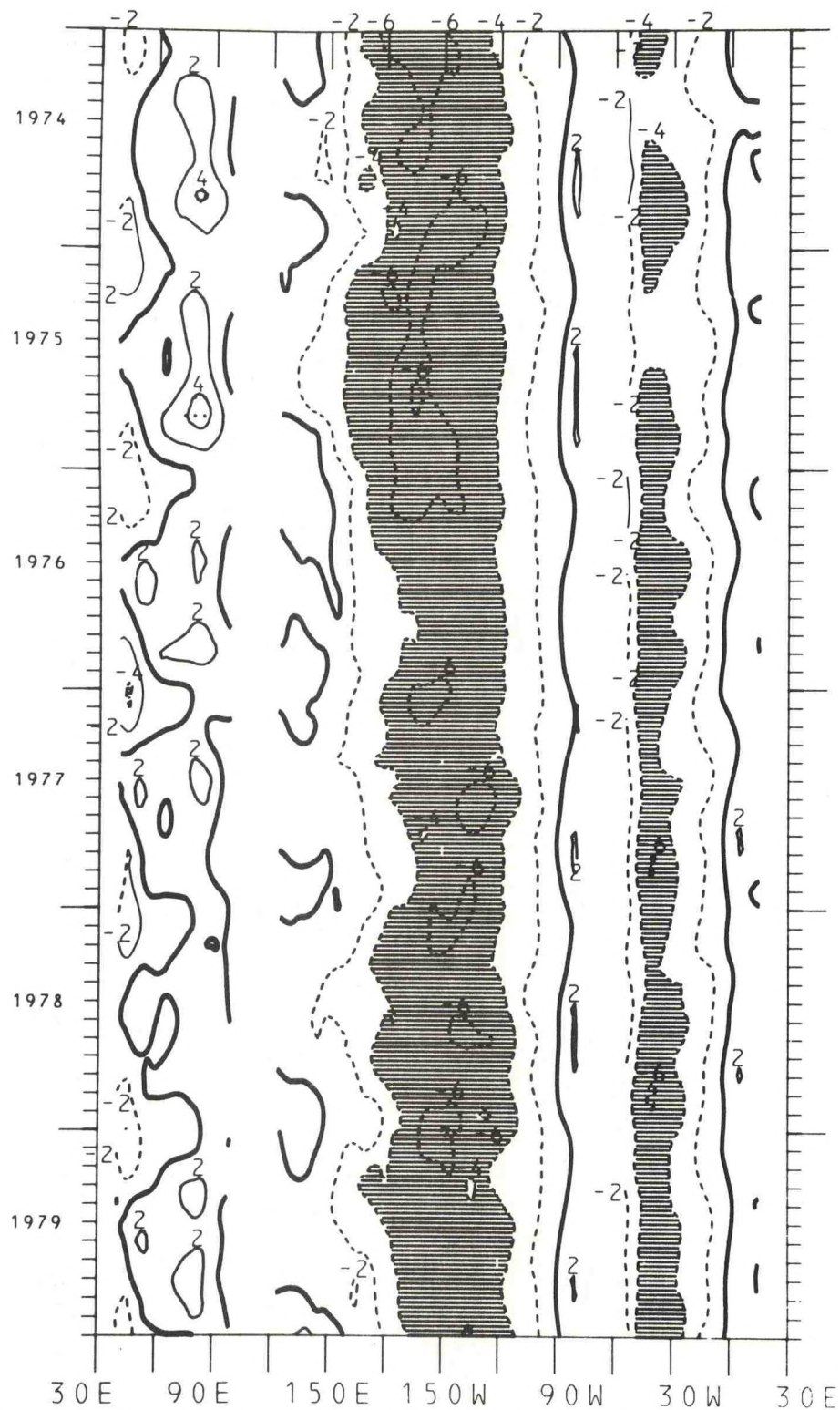
Figure 112. Time-longitude cross-section of the mean monthly equatorial zonal wind component for the years 1974-1979. The contour interval is 2.0 m/s. The zero isotherm is emphasized. Negative values (easterlies) are dashed. Light shading is greater than 4.0 m/s; dark shading is less than -4.0 m/s.
