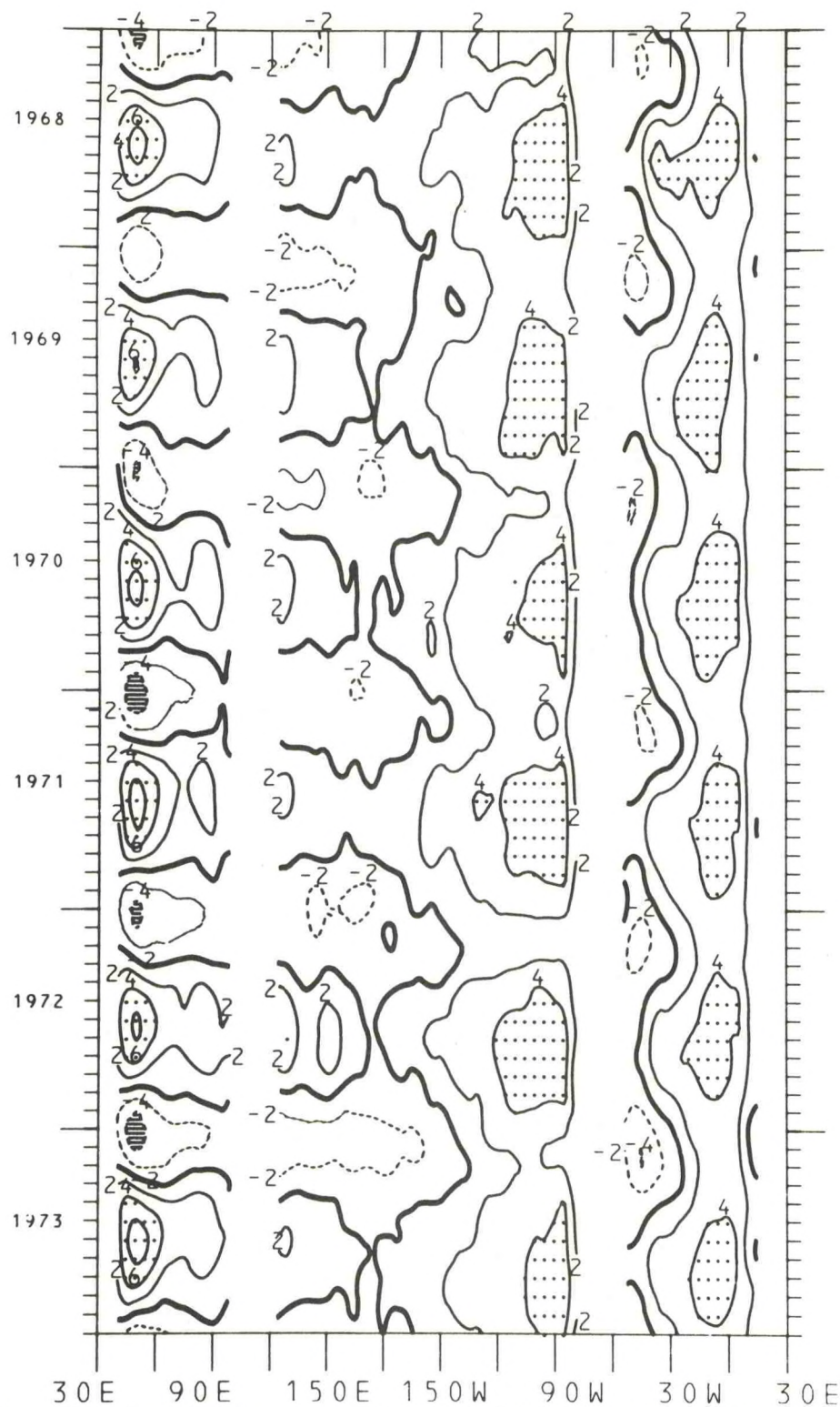
Figure 133. Time-longitude cross-section of the mean monthly equatorial meridional wind component for the years 1968-1973. The contour interval is 2.0 m/s. The zero isotherm is emphasized. Negative values (northerlies) are dashed. Light shading is greater than 4.0 m/s; dark shading is less than -4.0 m/s.
