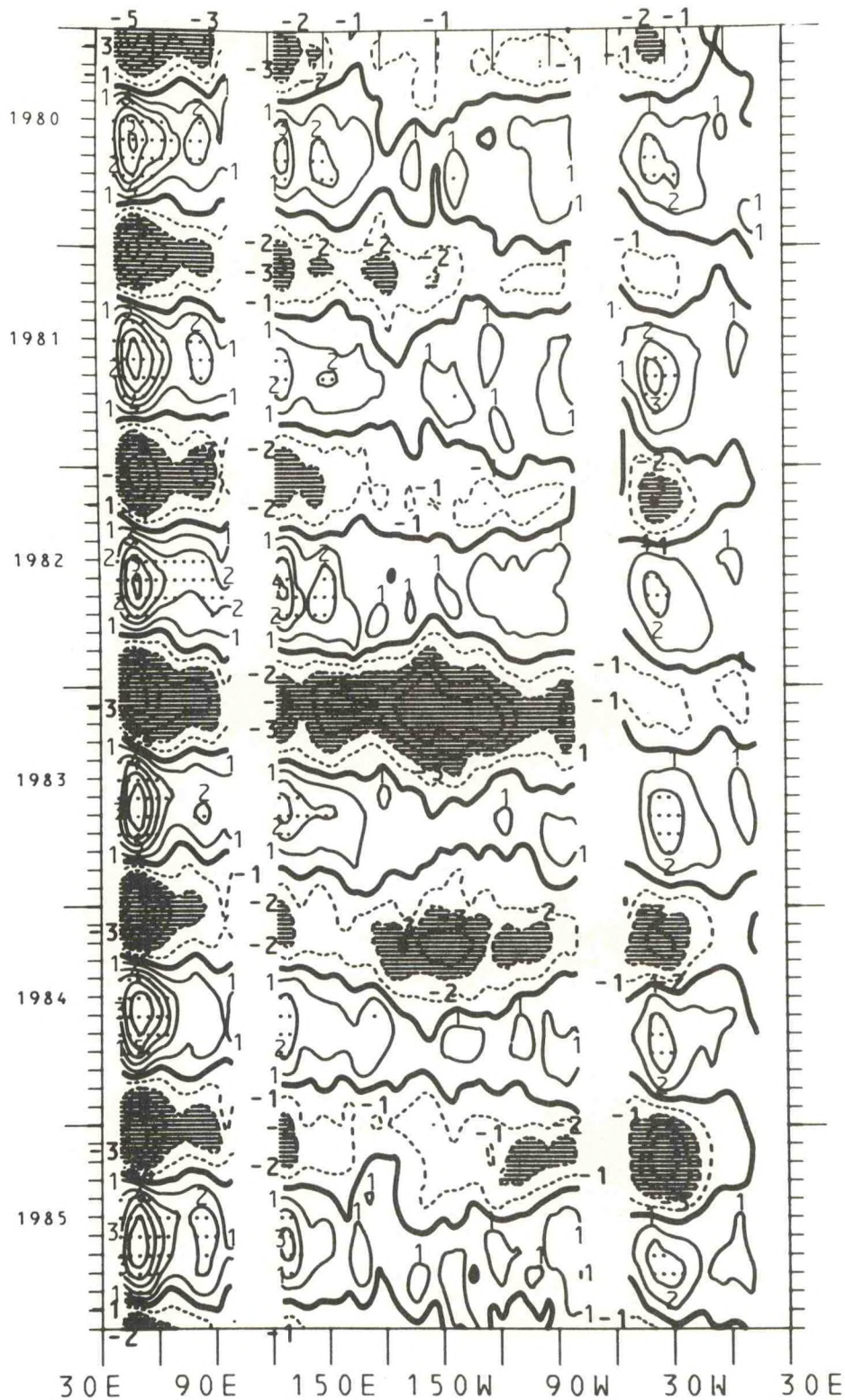
Figure 149. Time-longitude cross-section of equatorial meridional wind component expressed as the difference from the annual mean for the years 1980-1985. The contour interval is 1.0 m/s. The zero isotherm is emphasized. Light shading is greater than 2.0 m/s; dark shading is less than -2.0 m/s.
