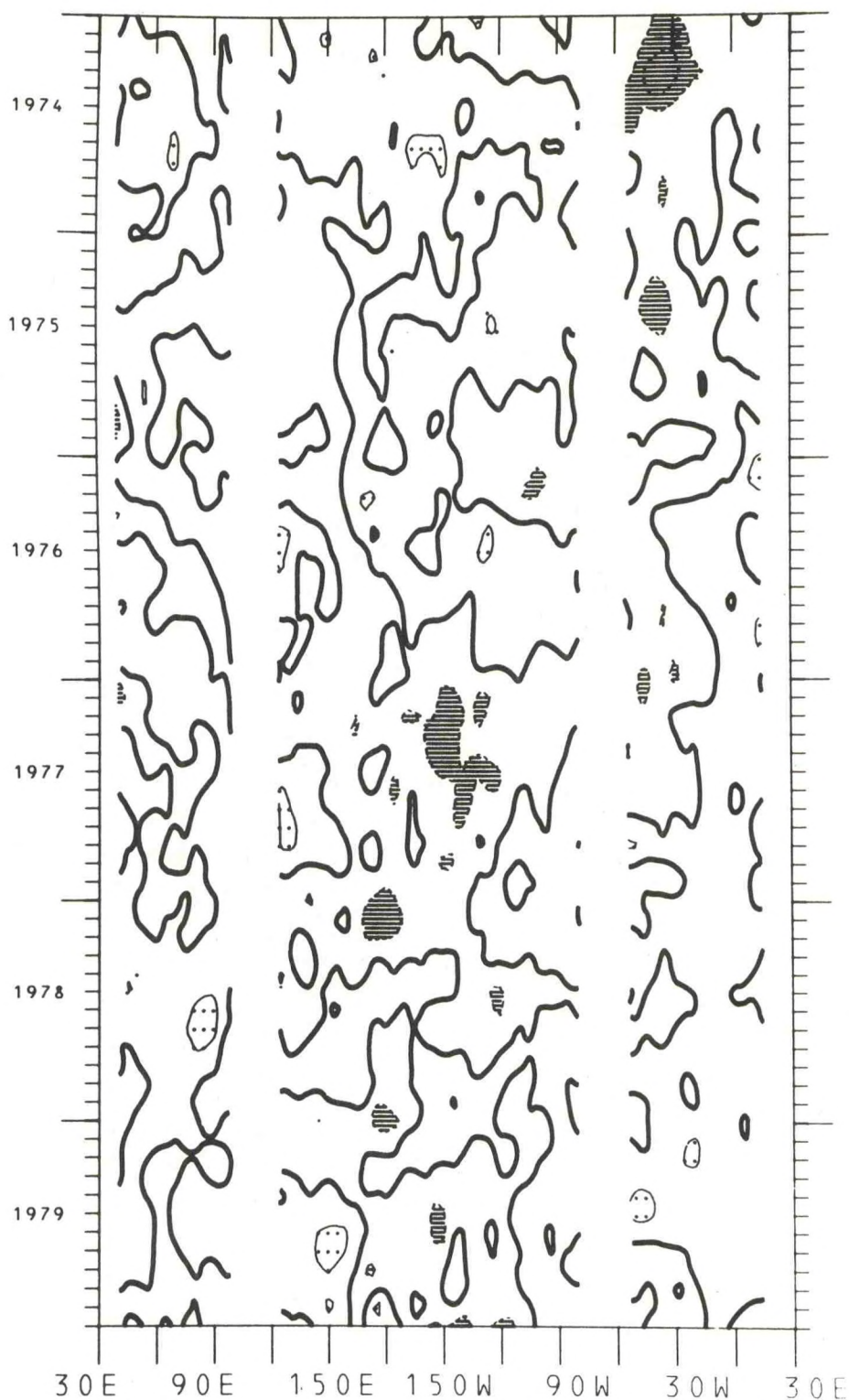
Figure 141. Time-longitude cross-section of equatorial meridional wind component anomalies for the years 1974-1979. The contour interval is 1.0 m/s. The zero isotherm is emphasized. Light shading is greater than 1.0 m/s; dark shading is less than -1.0 m/s.
