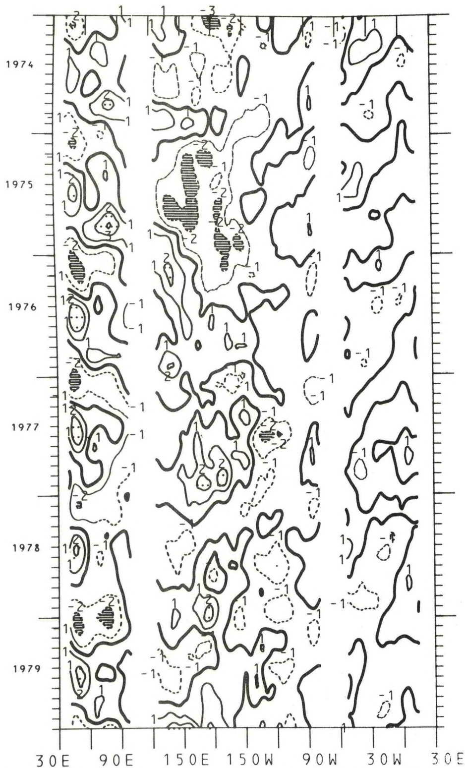
Figure 126. Time-longitude cross-section of equatorial zonal wind component expressed as the difference from the annual mean for the years 1974-1979. The contour interval is 1.0 m/s. The zero isotherm is emphasized. Light shading is greater than 2.0 m/s; dark shading is less than -2.0 m/s.
