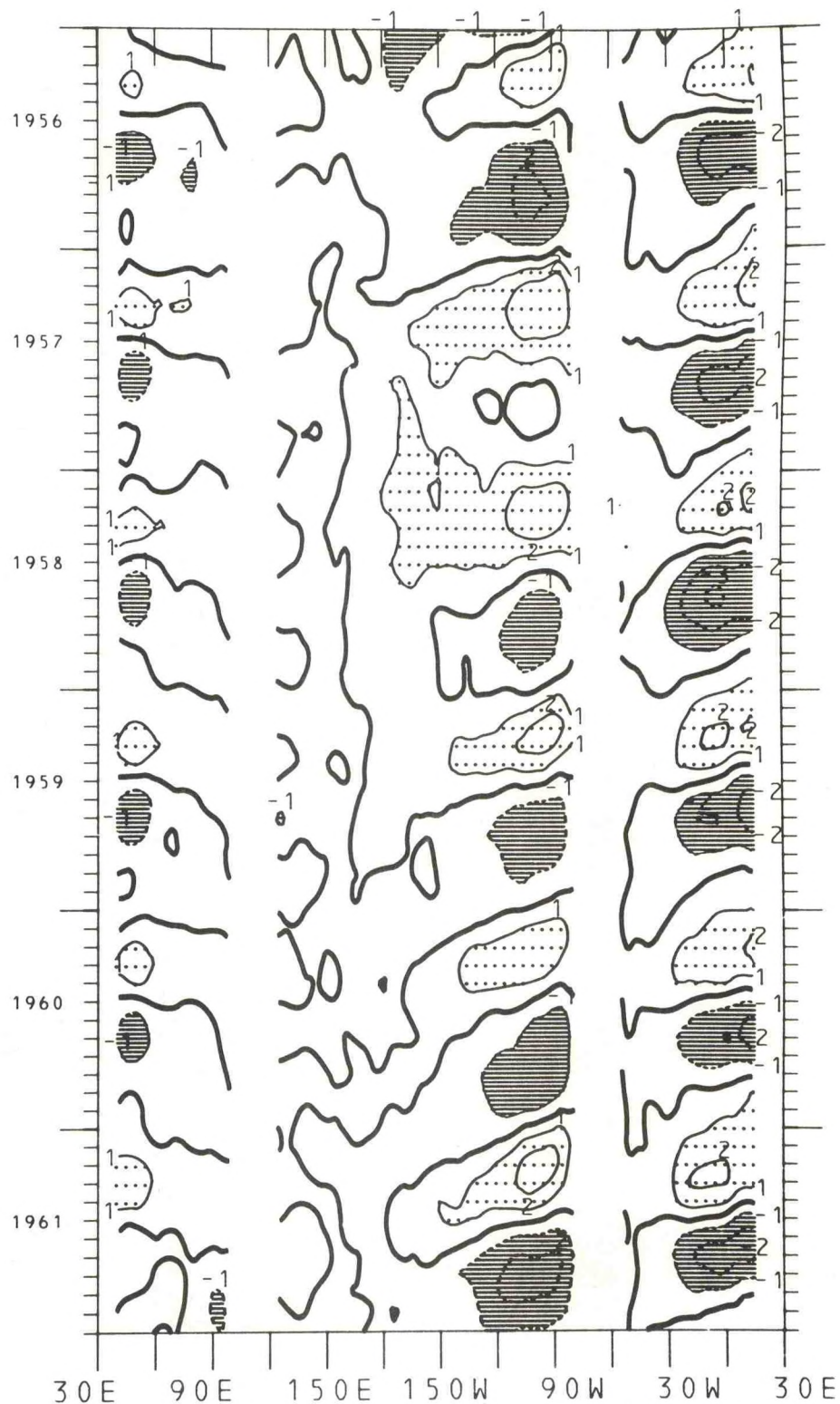
Figure 101. Time-longitude cross-section of equatorial SST expressed as the difference from the annual mean for the years 1956-1961. The contour interval is 1.0^{\circ}\text{C} . The zero isotherm is emphasized. Negative values are dashed. Light shading is greater than 1.0^{\circ}\text{C} ; dark shading is less than -1.0^{\circ}\text{C} .
