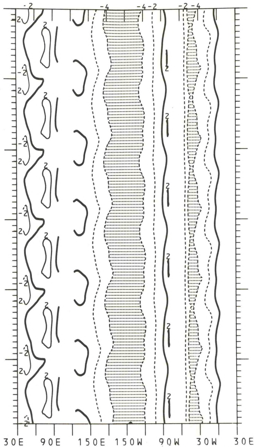
Figure 107. Time-longitude cross-section of the mean equatorial zonal wind component based on the period 1950-1979. The contour interval is 2.0 m/s. The zero isotherm is emphasized. Negative values (easterlies) are dashed. Values less than -4.0 m/s are shaded.
