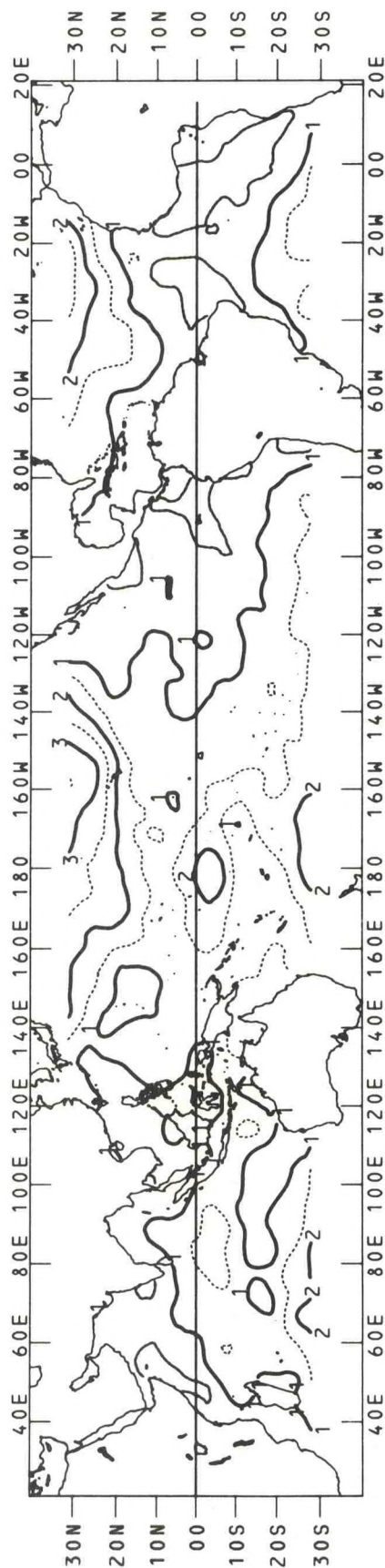
Figure 30b. December zonal wind component standard deviation for the period 1950-1979. The contour interval is .5 m/s.
