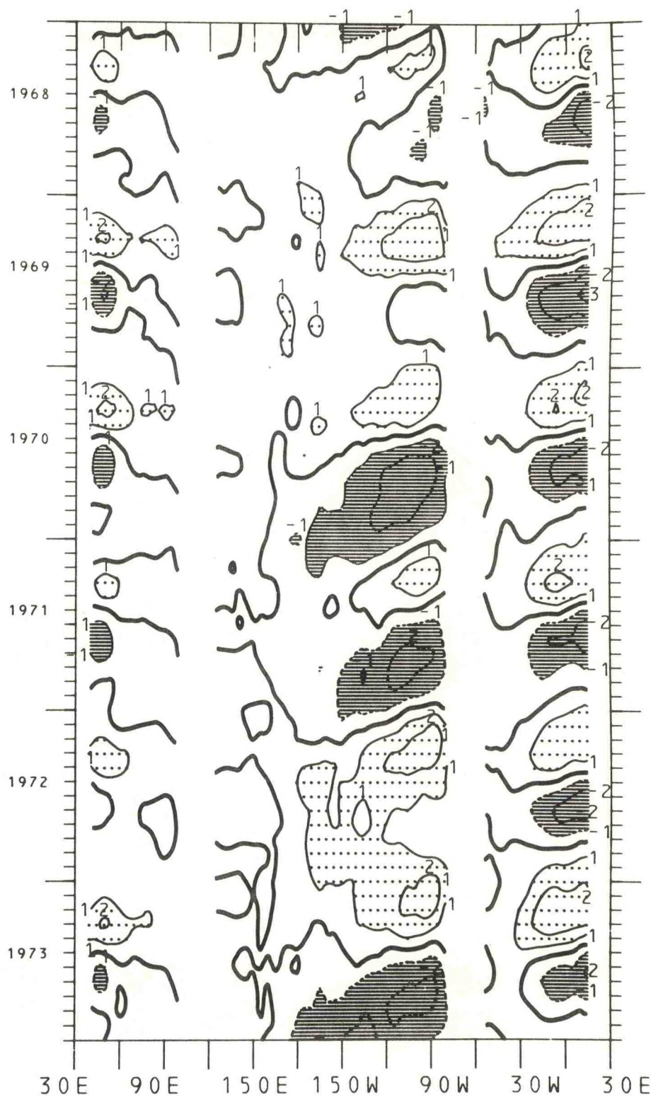
Figure 103. Time-longitude cross-section of equatorial SST expressed as the difference from the annual mean for the years 1968-1973. The contour interval is 1.0^{\circ}\text{C} . The zero isotherm is emphasized. Negative values are dashed. Light shading is greater than 1.0^{\circ}\text{C} ; dark shading is less than -1.0^{\circ}\text{C} .
