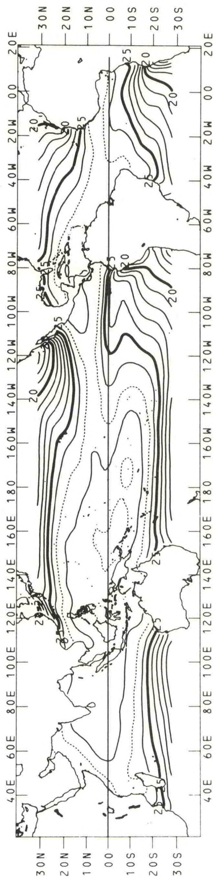
Figure 1. Annual SST mean for the period 1950-1979. The contour interval is 1.0°C. Dashed contours are 27°C and 29°C.
