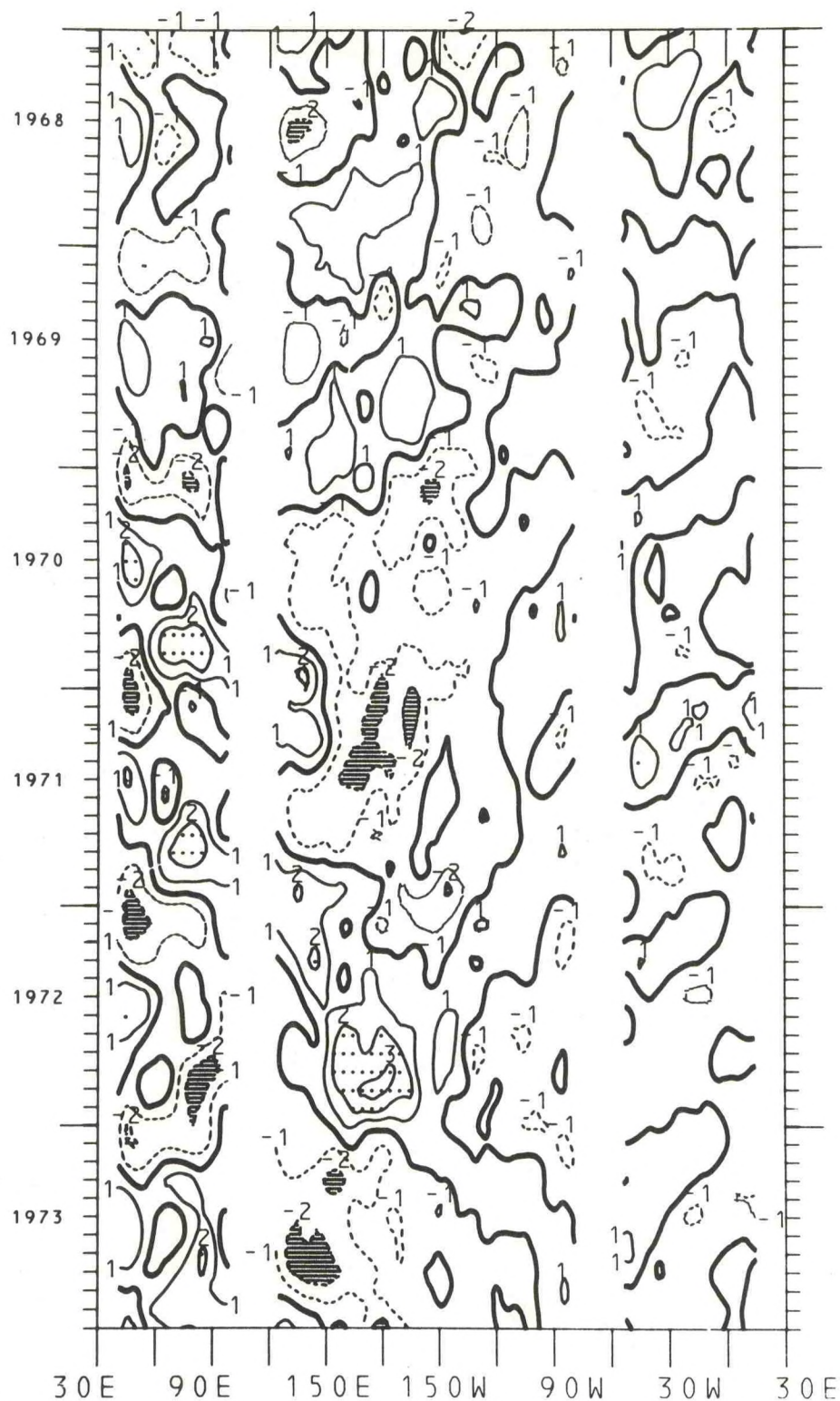
Figure 125. Time-longitude cross-section of equatorial zonal wind component expressed as the difference from the annual mean for the years 1968-1973. The contour interval is 1.0 m/s. The zero isotherm is emphasized. Light shading is greater than 2.0 m/s; dark shading is less than -2.0 m/s.
