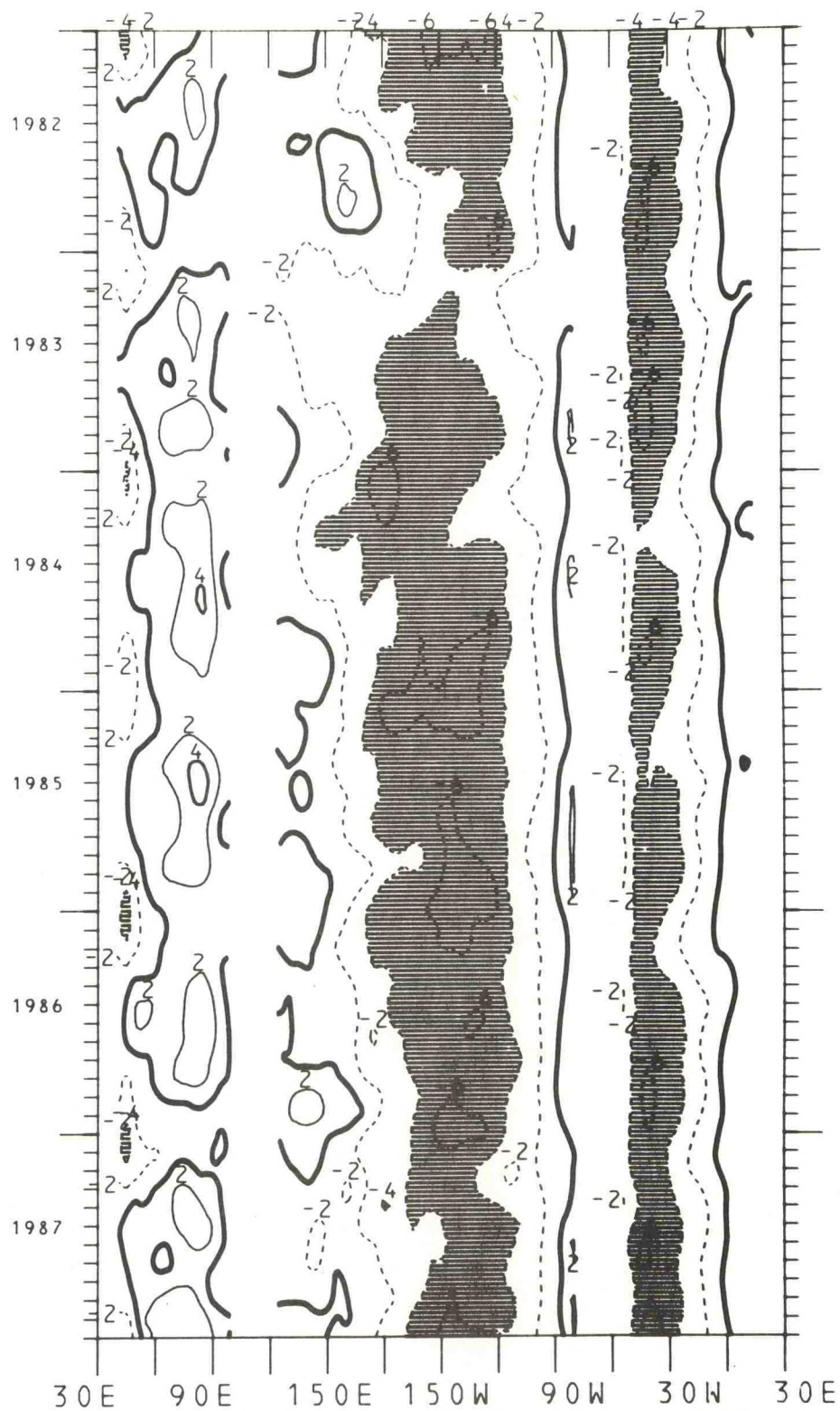
Figure 114. Time-longitude cross-section of the mean monthly equatorial zonal wind component for the years 1982-1987. The contour interval is 2.0 m/s. The zero isotherm is emphasized. Negative values (easterlies) are dashed. Light shading is greater than 4.0 m/s; dark shading is less than -4.0 m/s.
