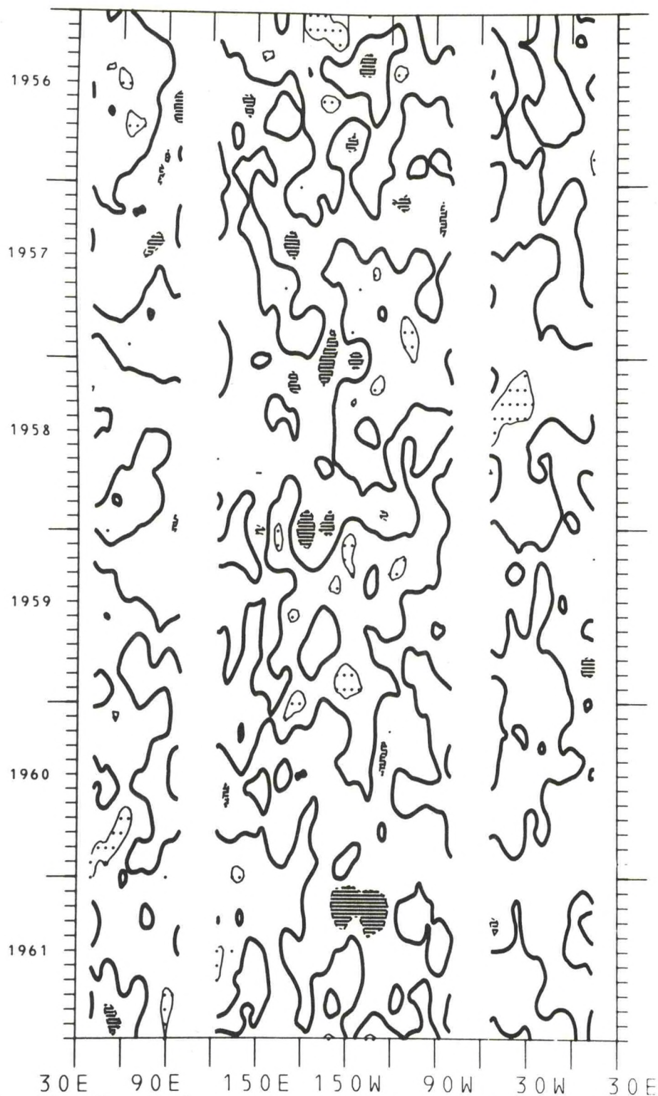
Figure 138. Time-longitude cross-section of equatorial meridional wind component anomalies for the years 1956-1961. The contour interval is 1.0 m/s. The zero isotherm is emphasized. Light shading is greater than 1.0 m/s; dark shading is less than -1.0 m/s.
