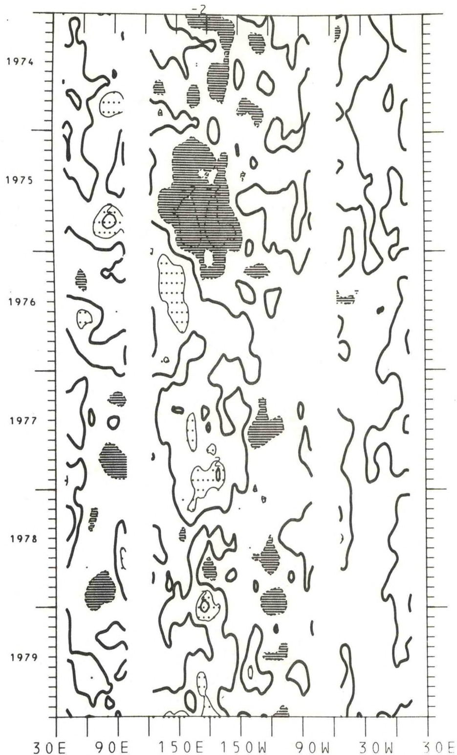
Figure 119. Time-longitude cross-section of equatorial zonal wind component anomalies for the years 1974-1979. The contour interval is 1.0 m/s. The zero isotherm is emphasized. Light shading is greater than 1.0 m/s; dark shading is less than -1.0 m/s.
