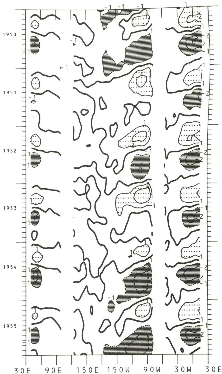
Figure 100. Time-longitude cross-section of equatorial SST expressed as the difference from the annual mean for the years 1950-1955. The contour interval is 1.0°C. The zero isotherm is emphasized. Negative values are dashed. Light shading is greater than 1.0°C; dark shading is less than -1.0°C.
