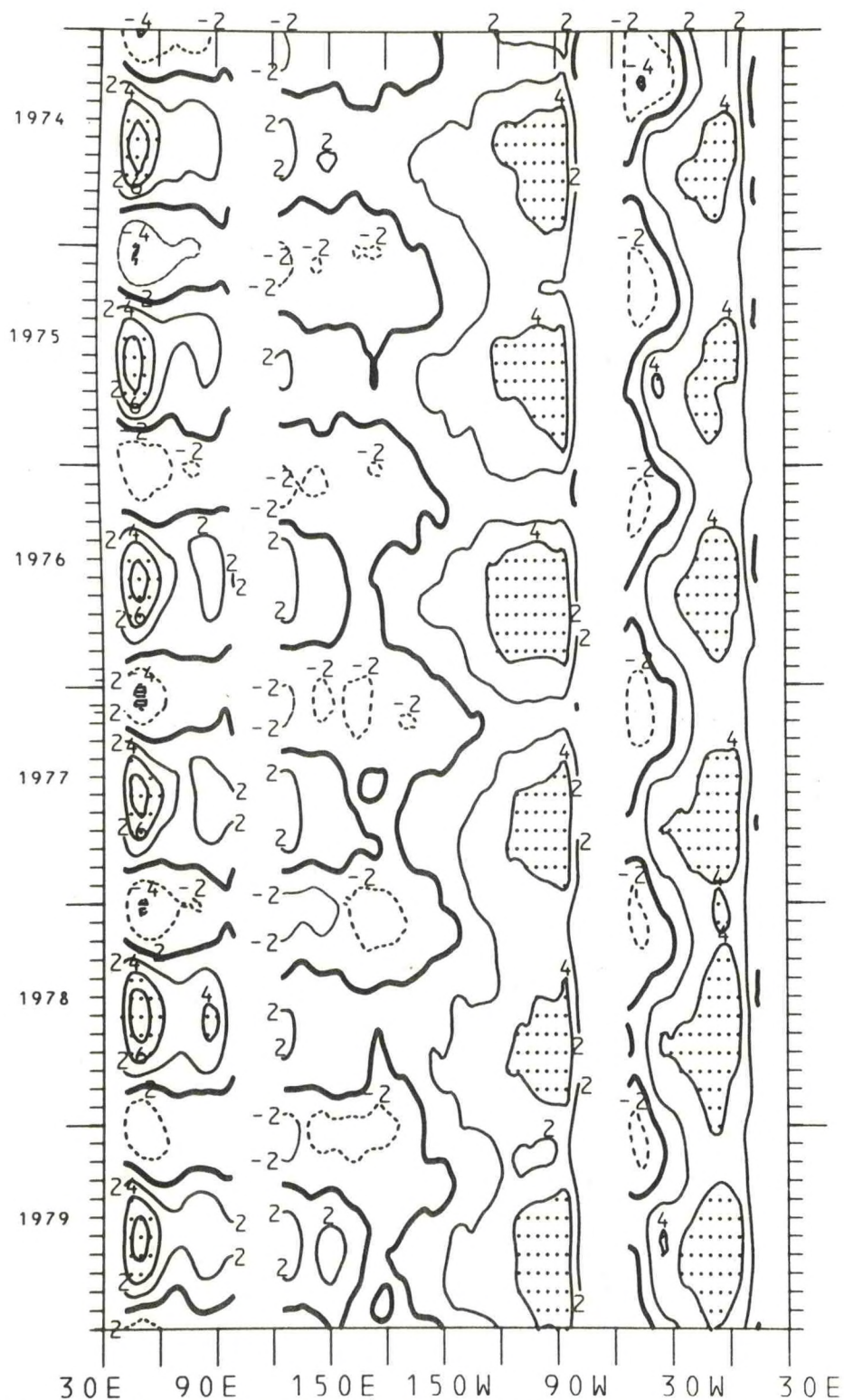
Figure 134. Time-longitude cross-section of the mean monthly equatorial meridional wind component for the years 1974-1979. The contour interval is 2.0 m/s. The zero isotherm is emphasized. Negative values (northerlies) are dashed. Light shading is greater than 4.0 m/s; dark shading is less than -4.0 m/s.
