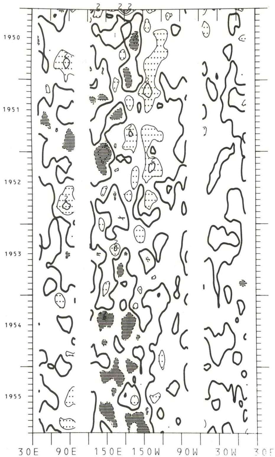
Figure 115. Time-longitude cross-section of equatorial zonal wind component anomalies for the years 1950-1955. The contour interval is 1.0 m/s. The zero isotherm is emphasized. Light shading is greater than 1.0 m/s; dark shading is less than -1.0 m/s.
