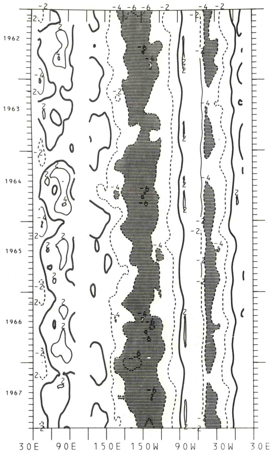
Figure 110. Time-longitude cross-section of the mean monthly equatorial zonal wind component for the years 1962-1967. The contour interval is 2.0 m/s. The zero isotherm is emphasized. Negative values (easterlies) are dashed. Light shading is greater than 4.0 m/s; dark shading is less than -4.0 m/s.
