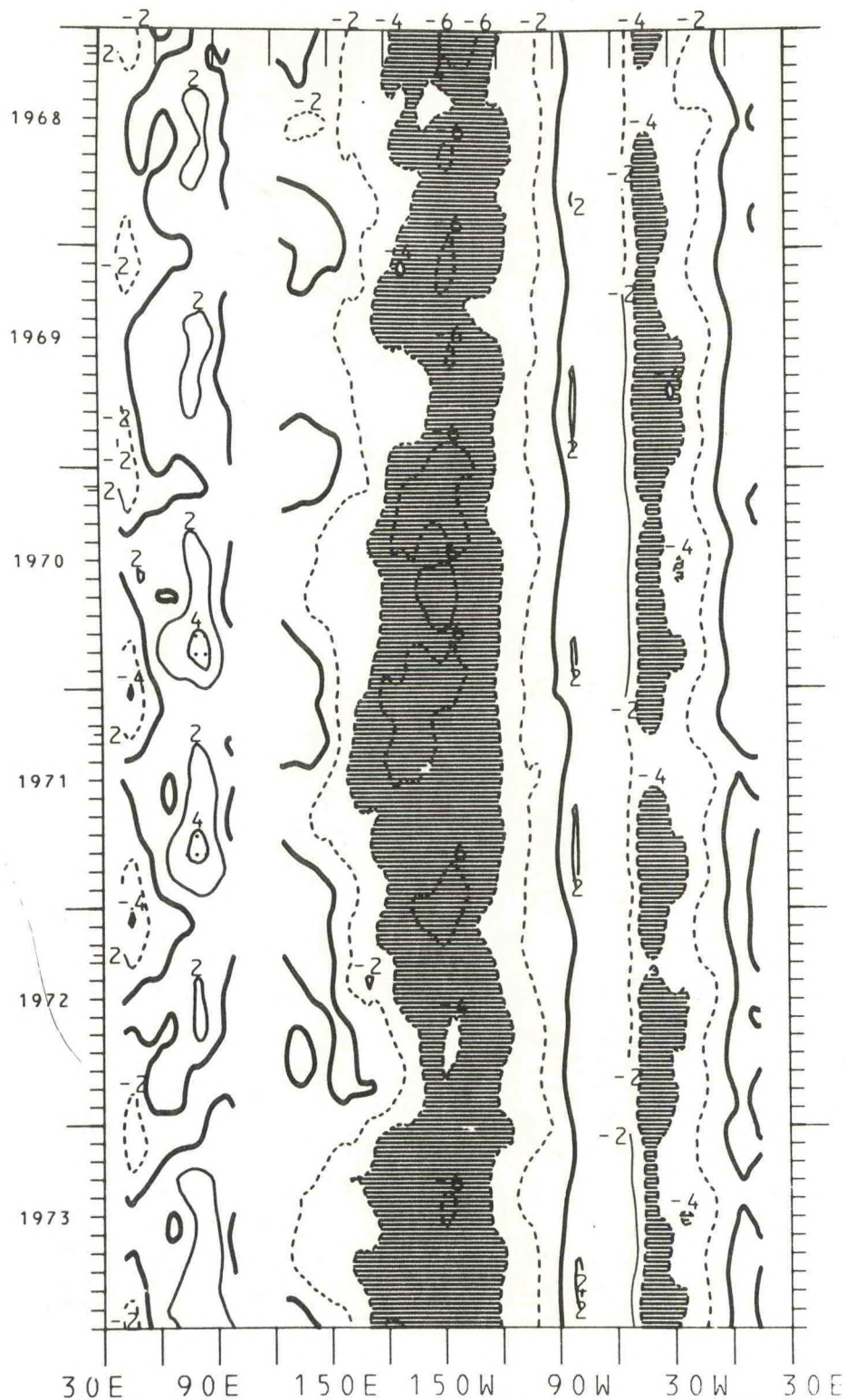
Figure 111. Time-longitude cross-section of the mean monthly equatorial zonal wind component for the years 1968-1973. The contour interval is 2.0 m/s. The zero isotherm is emphasized. Negative values (easterlies) are dashed. Light shading is greater than 4.0 m/s; dark shading is less than -4.0 m/s.
