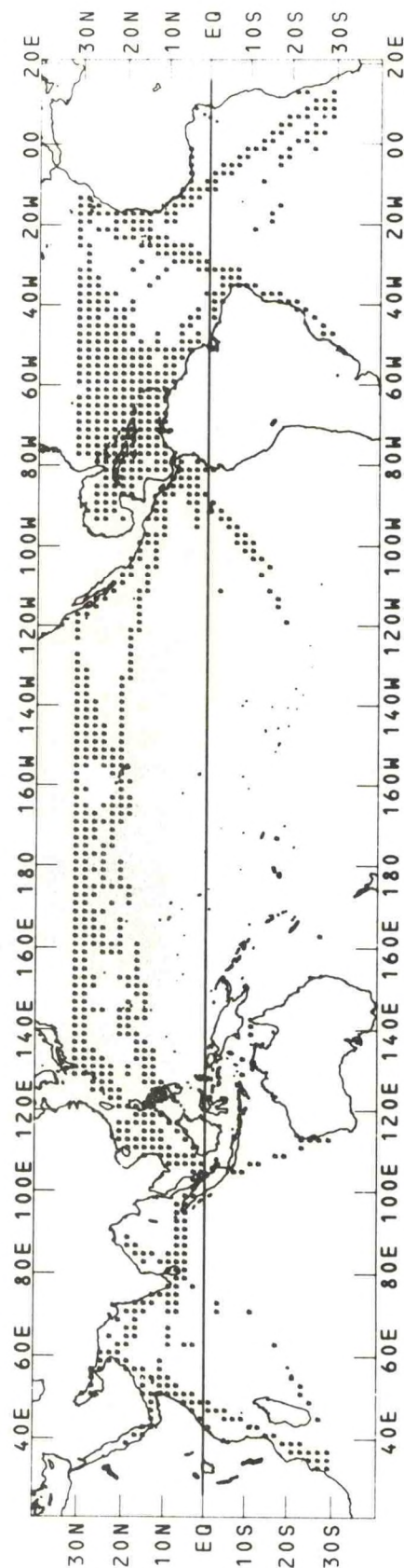
Figure A8. Locations which had data in a 2° latitude by 2° longitude grid box during all 30 years during the 1950-1979 period.
