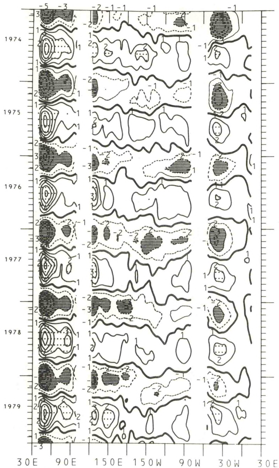
Figure 148. Time-longitude cross-section of equatorial meridional wind component expressed as the difference from the annual mean for the years 1974-1979. The contour interval is 1.0 m/s. The zero isotherm is emphasized. Light shading is greater than 2.0 m/s; dark shading is less than -2.0 m/s.
