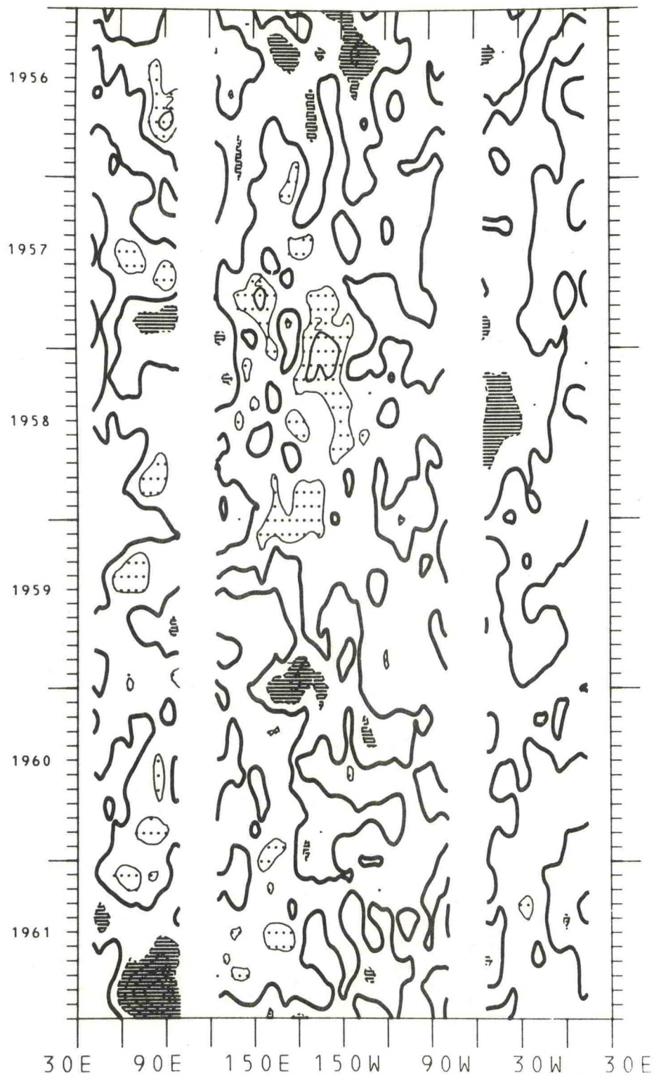
Figure 116. Time-longitude cross-section of equatorial zonal wind component anomalies for the years 1956-1961. The contour interval is 1.0 m/s. The zero isotherm is emphasized. Light shading is greater than 1.0 m/s; dark shading is less than -1.0 m/s.
