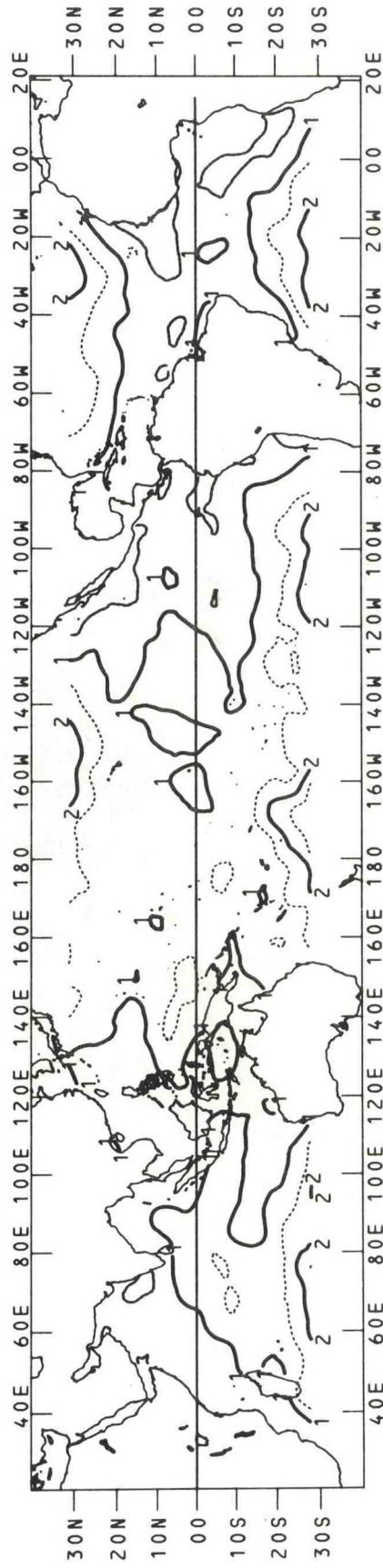
Figure 22b. April zonal wind component standard deviation for the period 1950-1979. The contour interval is .5 m/s.
