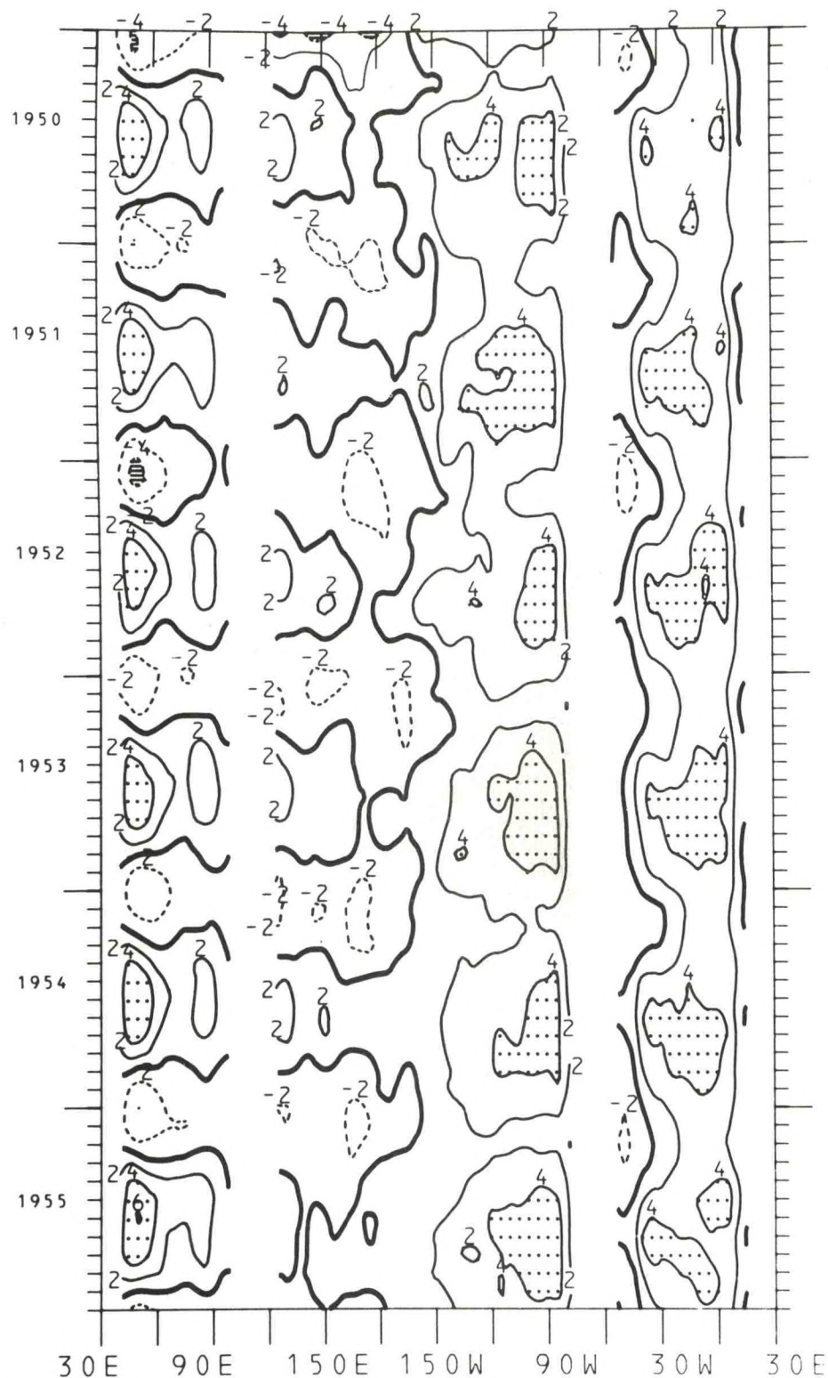
Figure 130. Time-longitude cross-section of the mean monthly equatorial meridional wind component for the years 1950-1955. The contour interval is 2.0 m/s. The zero isotherm is emphasized. Negative values (northerlies) are dashed. Light shading is greater than 4.0 m/s; dark shading is less than -4.0 m/s.
