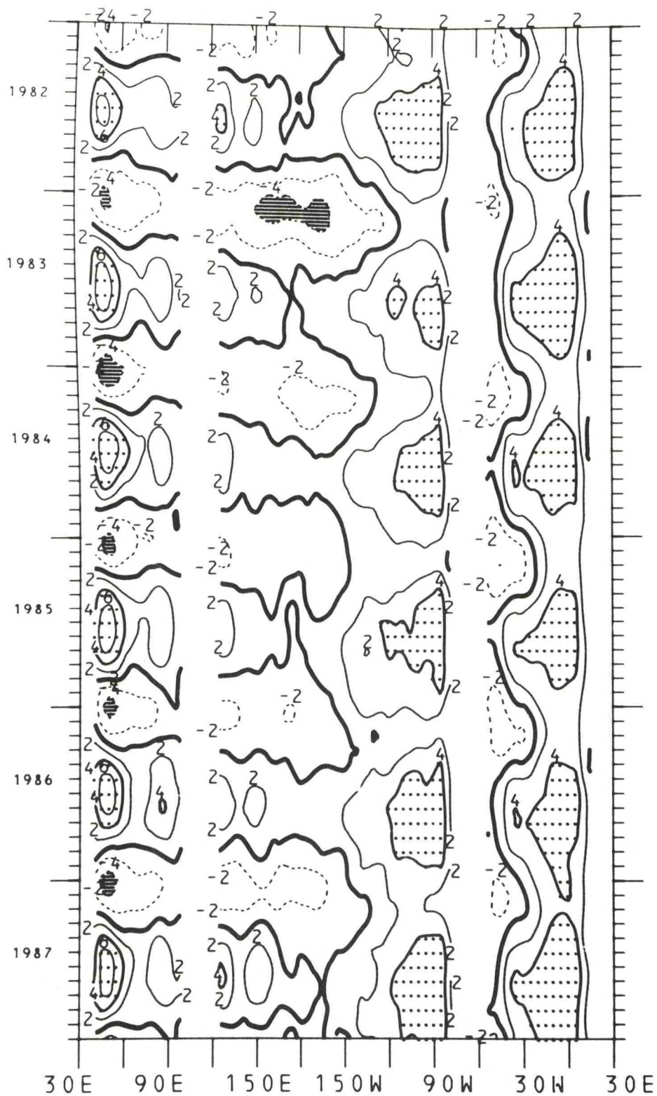
Figure 136. Time-longitude cross-section of the mean monthly equatorial meridional wind component for the years 1982-1987. The contour interval is 2.0 m/s. The zero isotherm is emphasized. Negative values (northerlies) are dashed. Light shading is greater than 4.0 m/s; dark shading is less than -4.0 m/s.
