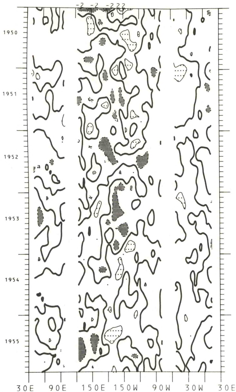
Figure 137. Time-longitude cross-section of equatorial meridional wind component anomalies for the years 1950-1955. The contour interval is 1.0 m/s. The zero isotherm is emphasized. Light shading is greater than 1.0 m/s; dark shading is less than -1.0 m/s.
