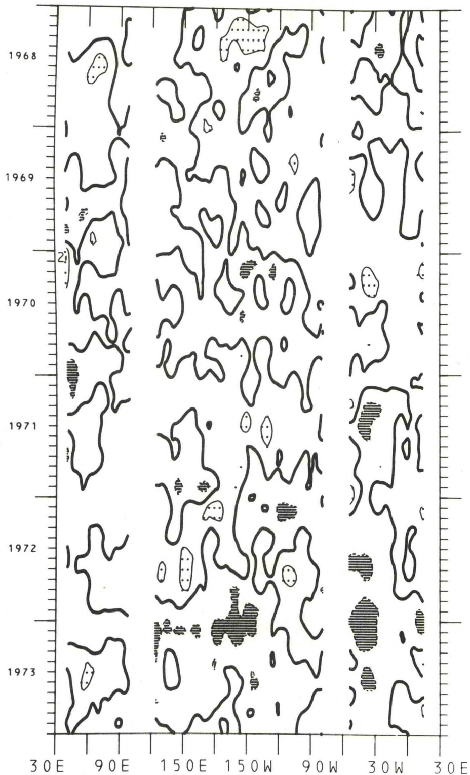
Figure 140. Time-longitude cross-section of equatorial meridional wind component anomalies for the years 1968-1973. The contour interval is 1.0 m/s. The zero isotherm is emphasized. Light shading is greater than 1.0 m/s; dark shading is less than -1.0 m/s.
