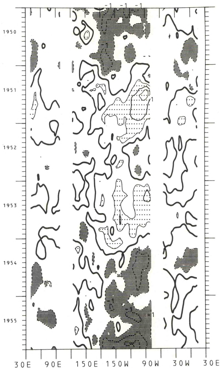
Figure 93. Time-longitude cross-section of equatorial SST anomalies for the years 1950-1955. The contour interval is .5^{\circ}\text{C} . The zero isotherm is emphasized. Negative values are dashed. Light shading is greater than 0.5^{\circ}\text{C} ; dark shading is less than -0.5^{\circ}\text{C} .
