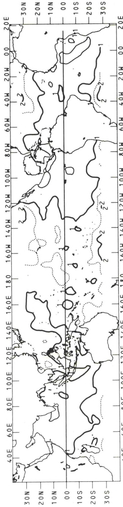
Figure 36b. January meridional wind component standard deviation for the period 1950-1979. The contour interval is .5 m/s.
