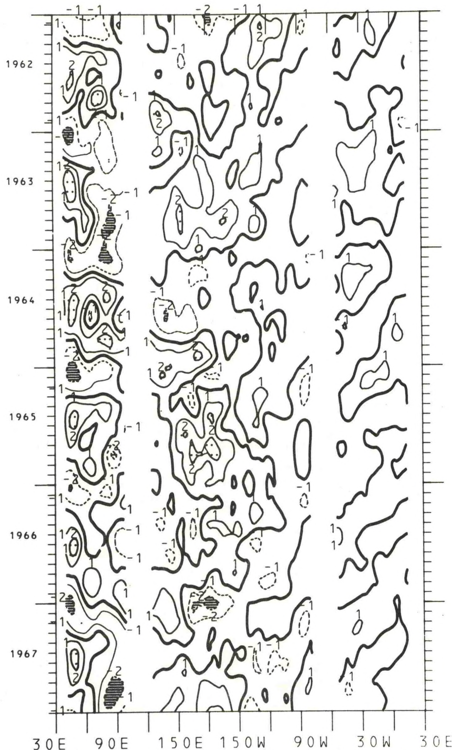
Figure 124. Time-longitude cross-section of equatorial zonal wind component expressed as the difference from the annual mean for the years 1962-1967. The contour interval is 1.0 m/s. The zero isotherm is emphasized. Light shading is greater than 2.0 m/s; dark shading is less than -2.0 m/s.
