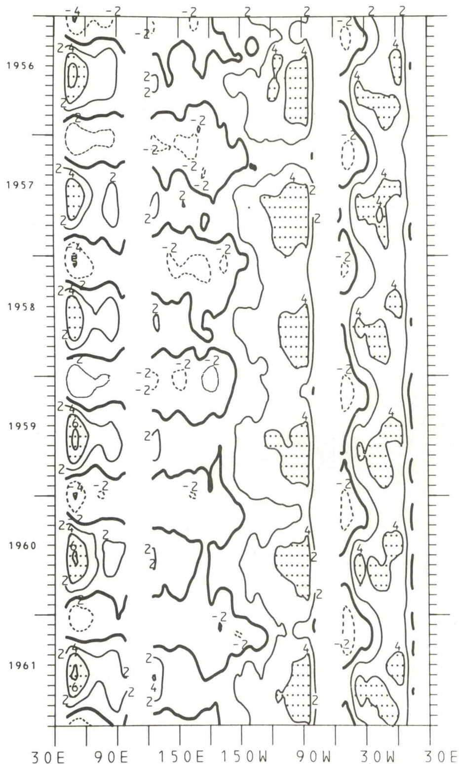
Figure 131. Time-longitude cross-section of the mean monthly equatorial meridional wind component for the years 1956-1961. The contour interval is 2.0 m/s. The zero isotherm is emphasized. Negative values (northerlies) are dashed. Light shading is greater than 4.0 m/s; dark shading is less than -4.0 m/s.
