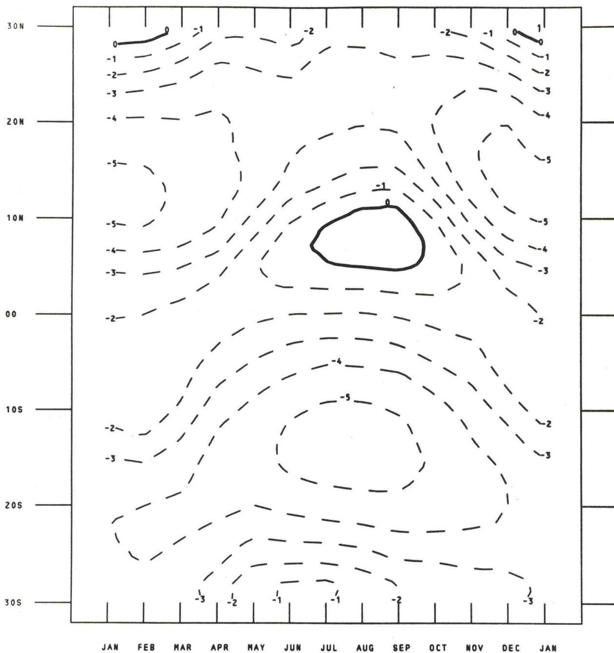
Figure 152. Time-latitude cross-section of the zonally averaged zonal wind. The contour interval is 1 m/s. Negative values (easterlies) are dashed.
