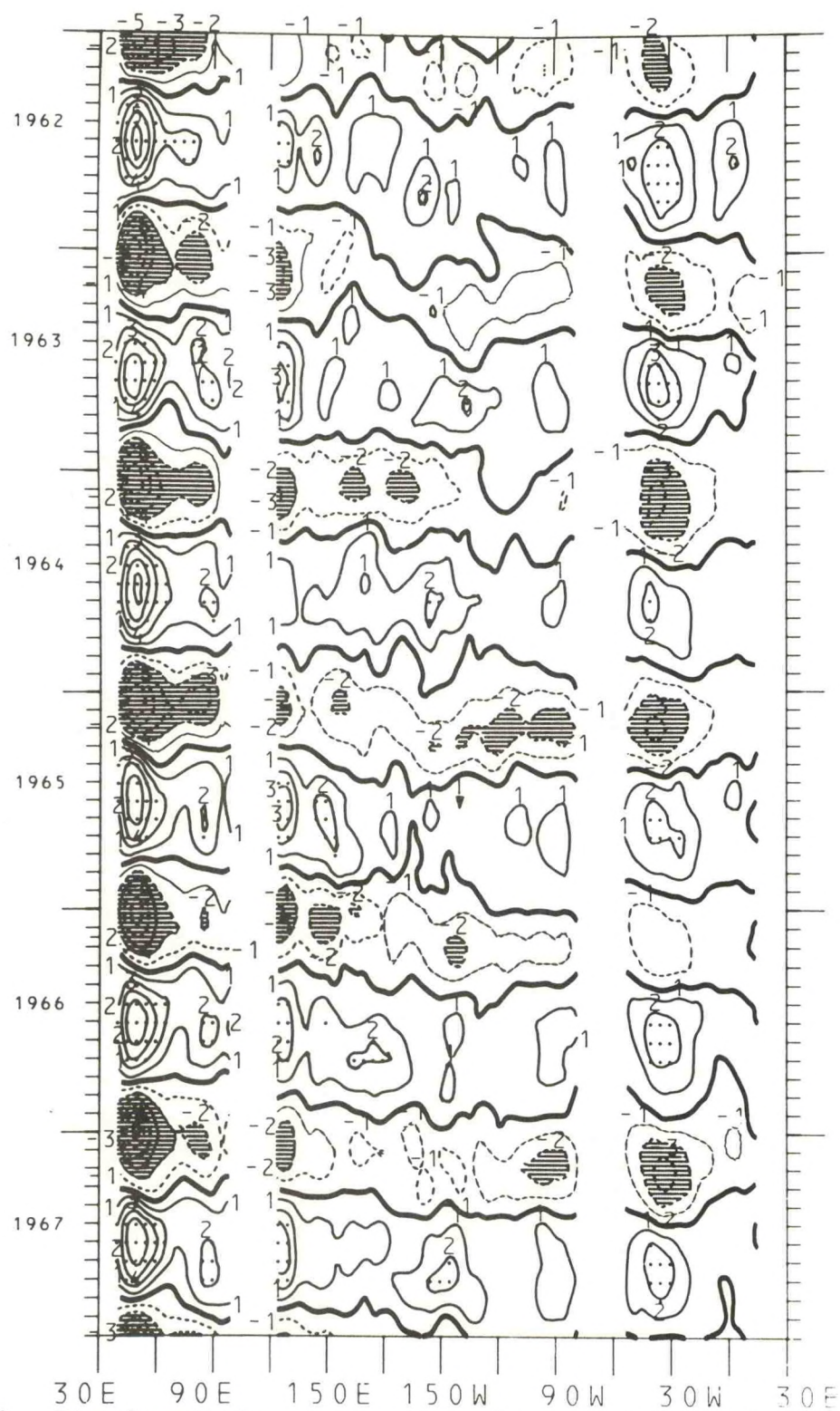
Figure 146. Time-longitude cross-section of equatorial meridional wind component expressed as the difference from the annual mean for the years 1962-1967. The contour interval is 1.0 m/s. The zero isotherm is emphasized. Light shading is greater than 2.0 m/s; dark shading is less than -2.0 m/s.
