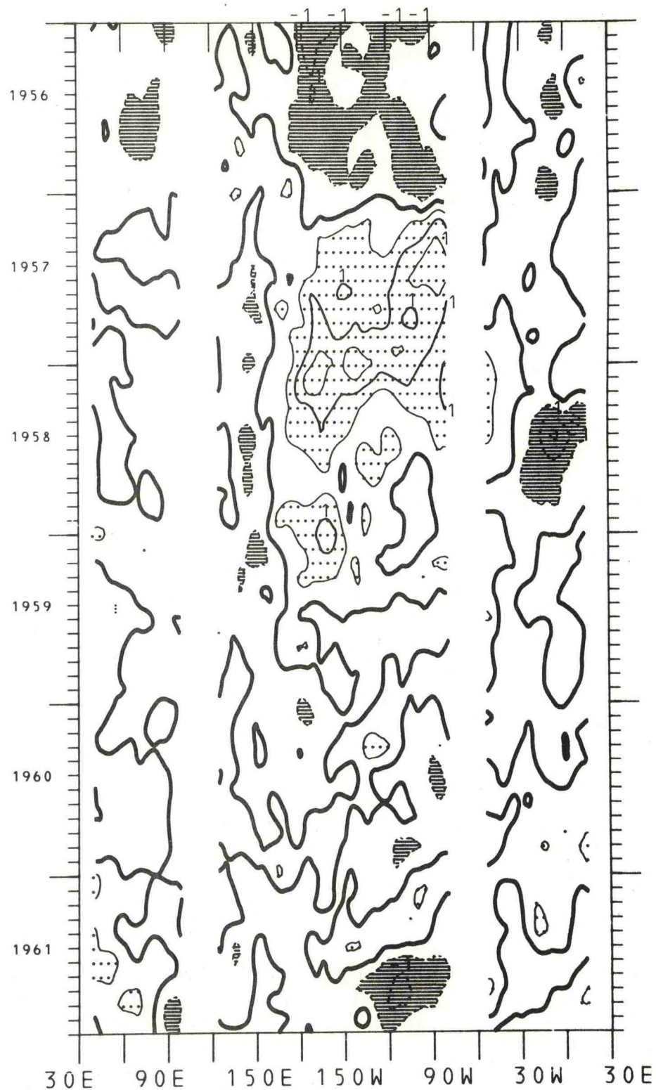
Figure 94. Time-longitude cross-section of equatorial SST anomalies for the years 1956-1961. The contour interval is .5^{\circ}\text{C} . The zero isotherm is emphasized. Negative values are dashed. Light shading is greater than 0.5^{\circ}\text{C} ; dark shading is less than -0.5^{\circ}\text{C} .
