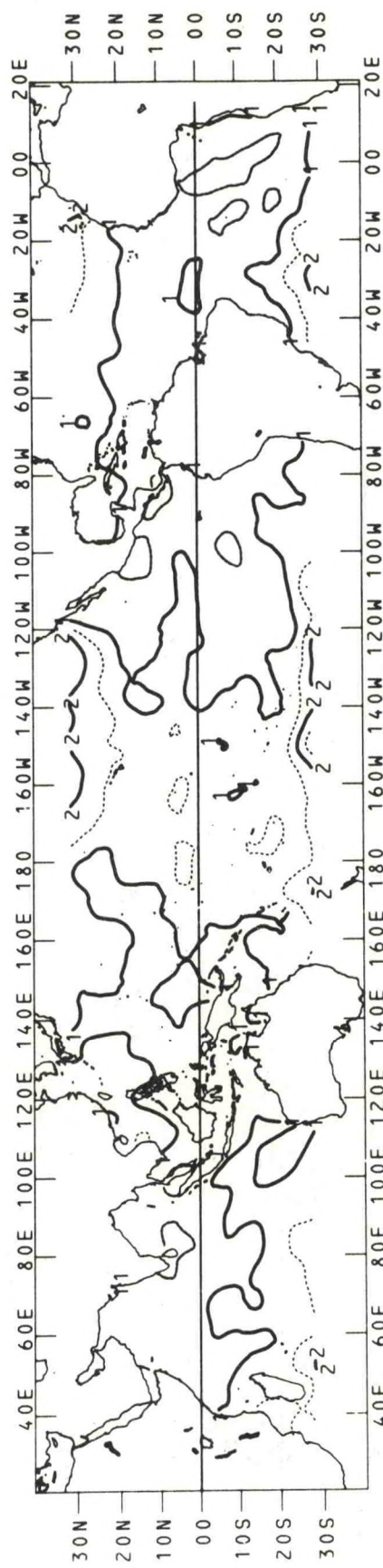
Figure 37b. February meridional wind component standard deviation for the period 1950-1979. The contour interval is .5 m/s.
