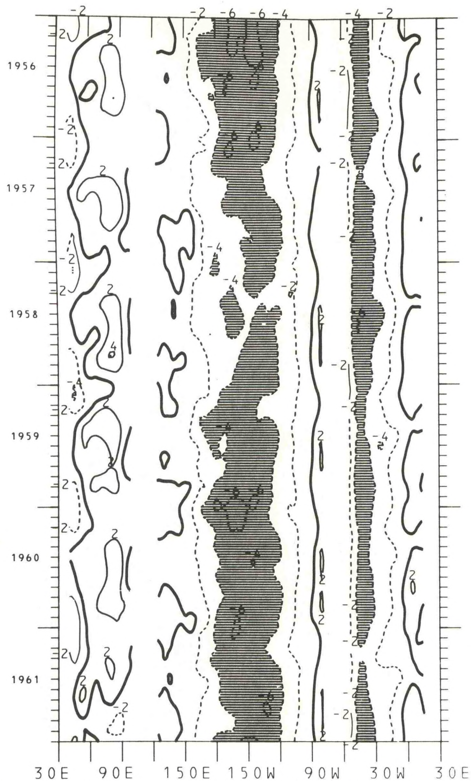
Figure 109. Time-longitude cross-section of the mean monthly equatorial zonal wind component for the years 1956-1961. The contour interval is 2.0 m/s. The zero isotherm is emphasized. Negative values (easterlies) are dashed. Light shading is greater than 4.0 m/s; dark shading is less than -4.0 m/s.
