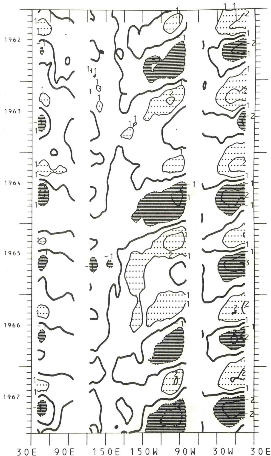
Figure 102. Time-longitude cross-section of equatorial SST expressed as the difference from the annual mean for the years 1962-1967. The contour interval is 1.0^{\circ}\text{C} . The zero isotherm is emphasized. Negative values are dashed. Light shading is greater than 1.0^{\circ}\text{C} ; dark shading is less than -1.0^{\circ}\text{C} .
