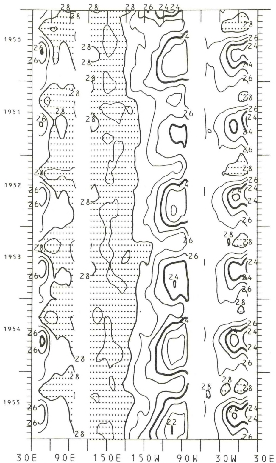
Figure 86. Time-longitude cross-section of the mean monthly equatorial SST for the years 1950-1955. The contour interval is 1°C. The 25°C isotherm is emphasized. Values greater than 28°C are shaded.
