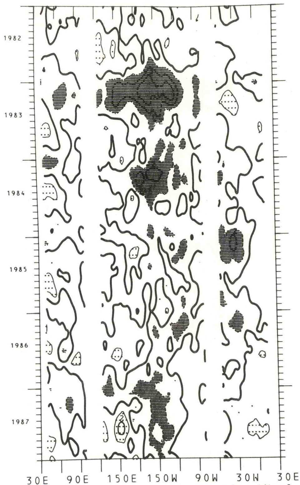
Figure 143. Time-longitude cross-section of equatorial meridional wind component anomalies for the years 1982-1987. The contour interval is 1.0 m/s. The zero isotherm is emphasized. Light shading is greater than 1.0 m/s; dark shading is less than -1.0 m/s.
