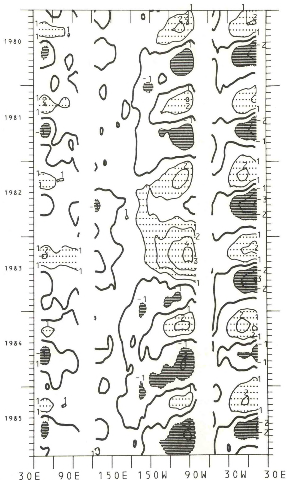
Figure 105. Time-longitude cross-section of equatorial SST expressed as the difference from the annual mean for the years 1980-1985. The contour interval is 1.0^{\circ}\text{C} . The zero isotherm is emphasized. Negative values are dashed. Light shading is greater than 1.0^{\circ}\text{C} ; dark shading is less than -1.0^{\circ}\text{C} .
