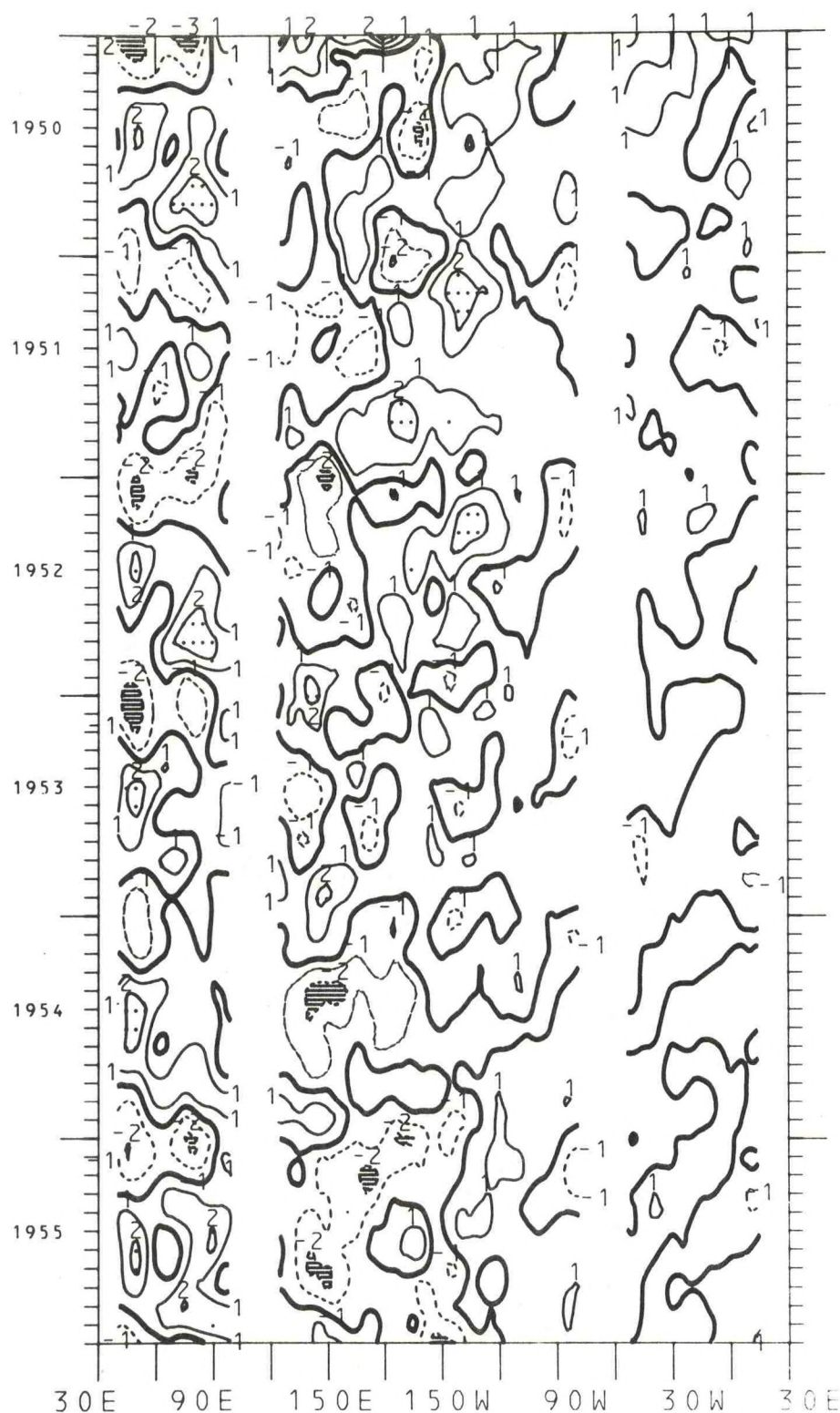
Figure 122. Time-longitude cross-section of equatorial zonal wind component expressed as the difference from the annual mean for the years 1950-1955. The contour interval is 1.0 m/s. The zero isotherm is emphasized. Light shading is greater than 2.0 m/s; dark shading is less than -2.0 m/s.
