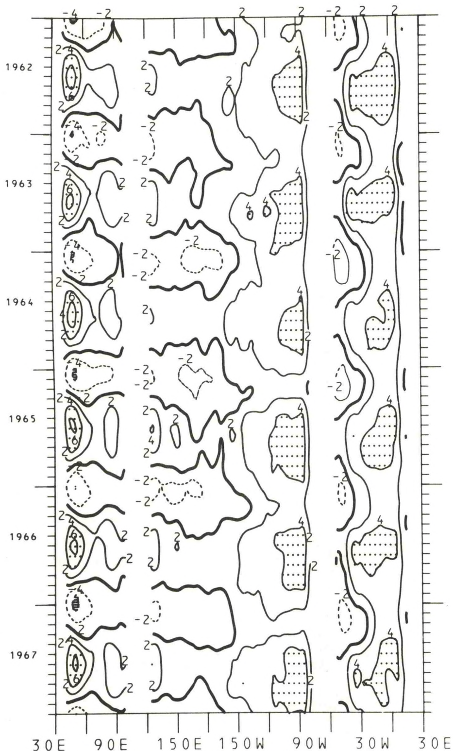
Figure 132. Time-longitude cross-section of the mean monthly equatorial meridional wind component for the years 1962-1967. The contour interval is 2.0 m/s. The zero isotherm is emphasized. Negative values (northerlies) are dashed. Light shading is greater than 4.0 m/s; dark shading is less than -4.0 m/s.
