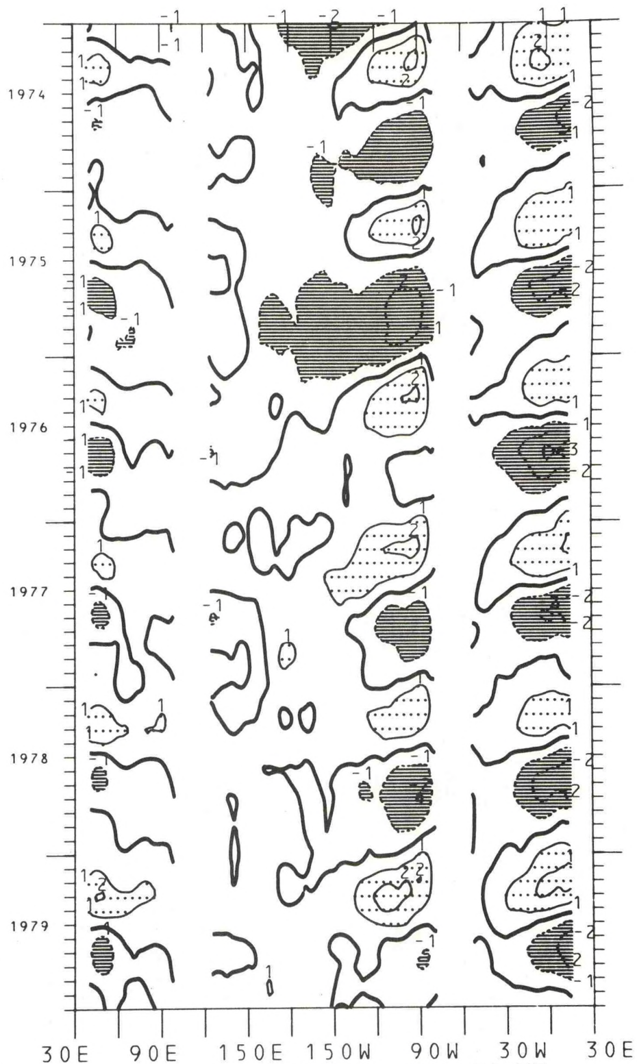
Figure 104. Time-longitude cross-section of equatorial SST expressed as the difference from the annual mean for the years 1974-1979. The contour interval is 1.0^{\circ}\text{C} . The zero isotherm is emphasized. Negative values are dashed. Light shading is greater than 1.0^{\circ}\text{C} ; dark shading is less than -1.0^{\circ}\text{C} .
