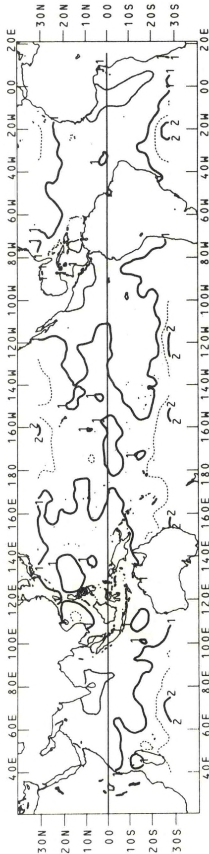
Figure 38b. March meridional wind component standard deviation for the period 1950-1979. The contour interval is .5 m/s.
