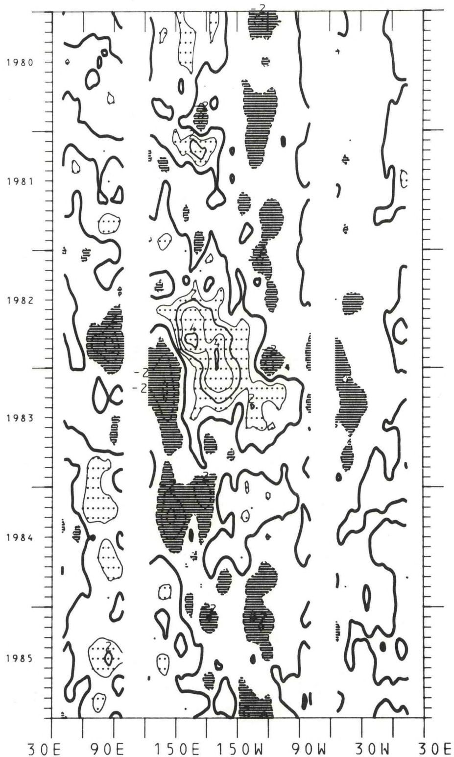
Figure 120. Time-longitude cross-section of equatorial zonal wind component anomalies for the years 1980-1985. The contour interval is 1.0 m/s. The zero isotherm is emphasized. Light shading is greater than 1.0 m/s; dark shading is less than -1.0 m/s.
