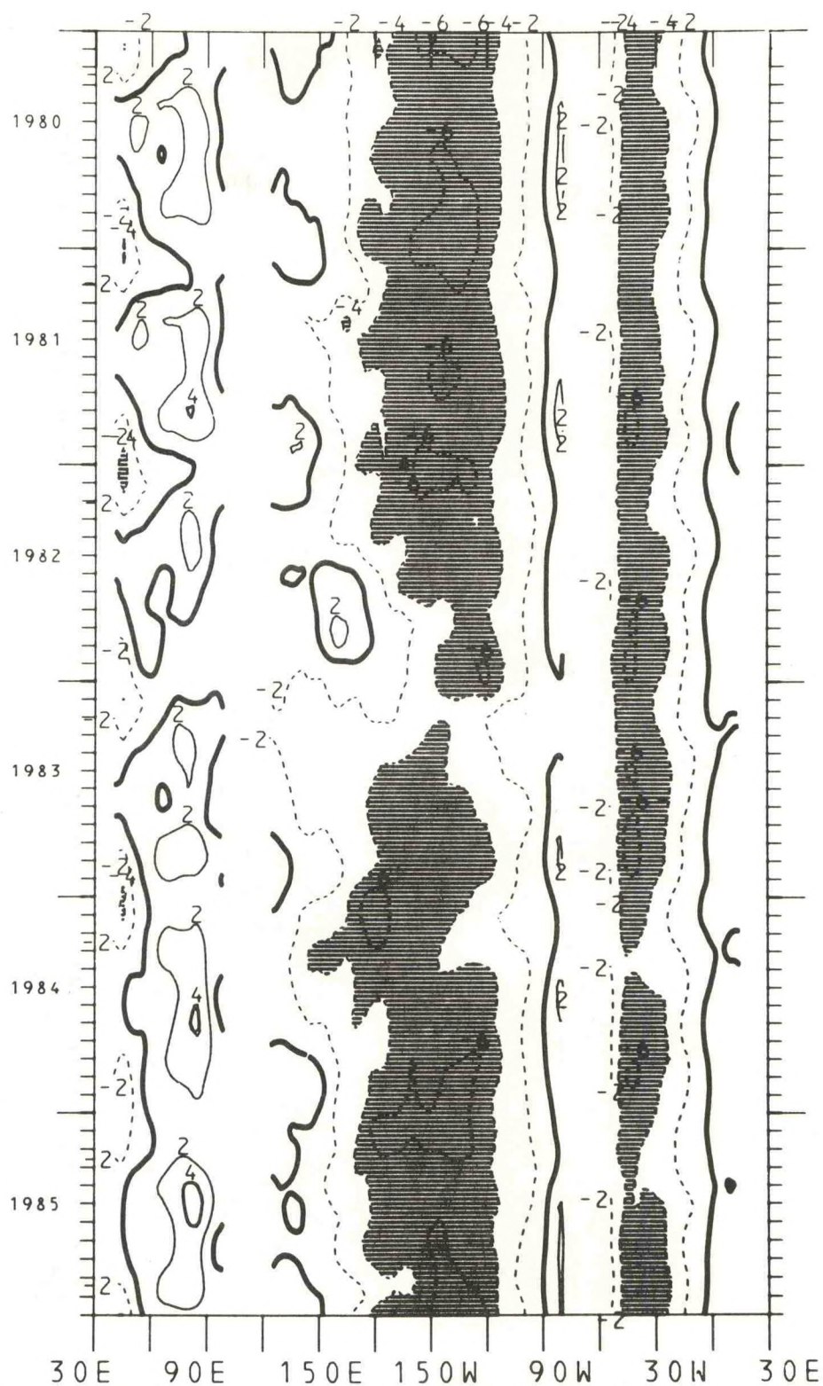
Figure 113. Time-longitude cross-section of the mean monthly equatorial zonal wind component for the years 1980-1985. The contour interval is 2.0 m/s. The zero isotherm is emphasized. Negative values (easterlies) are dashed. Light shading is greater than 4.0 m/s; dark shading is less than -4.0 m/s.
