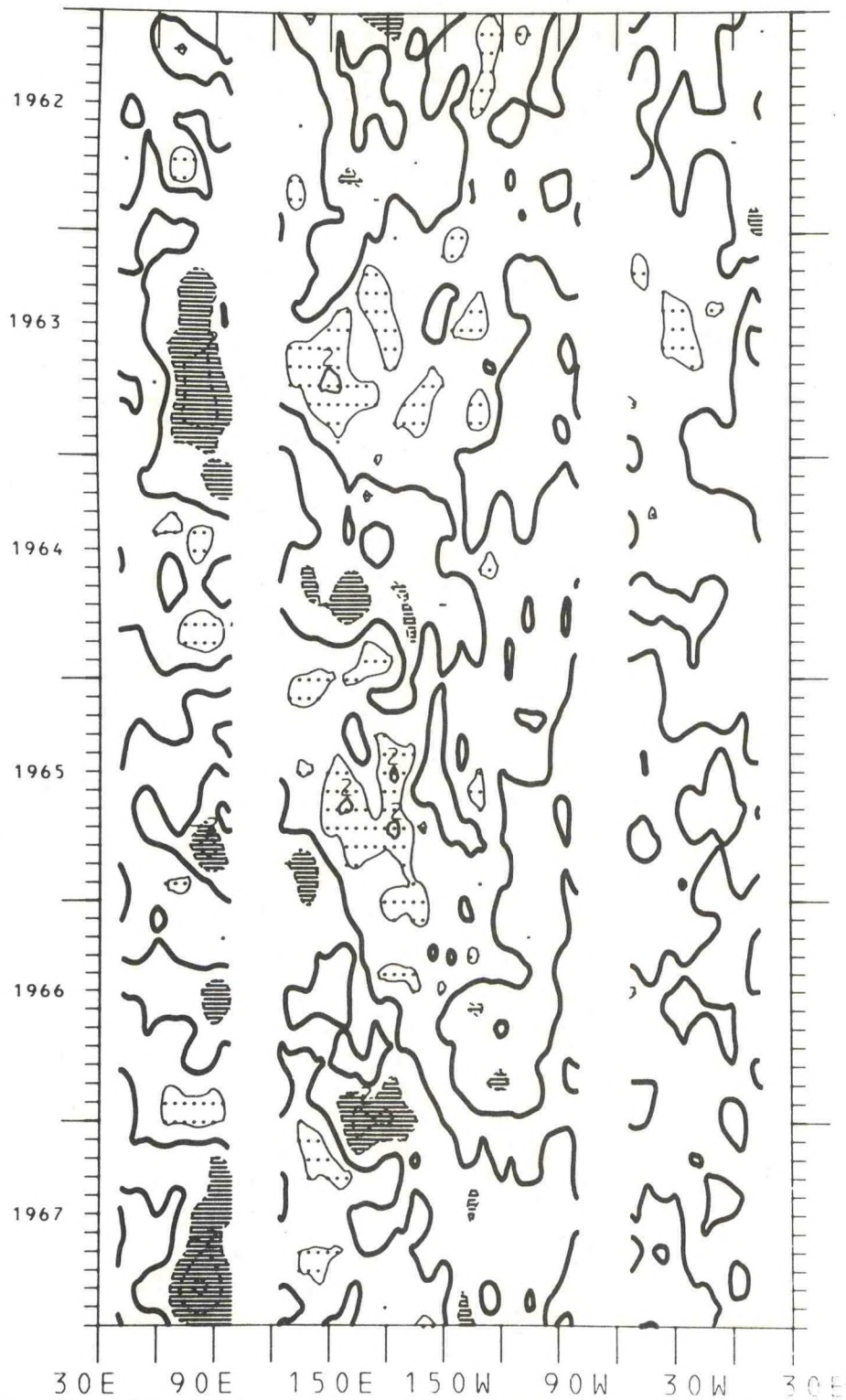
Figure 117. Time-longitude cross-section of equatorial zonal wind component anomalies for the years 1962-1967. The contour interval is 1.0 m/s. The zero isotherm is emphasized. Light shading is greater than 1.0 m/s; dark shading is less than -1.0 m/s.
