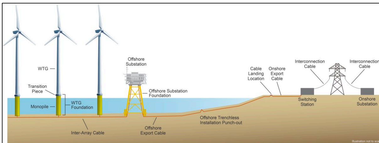
Figure 2. Conceptual Project Schematic
