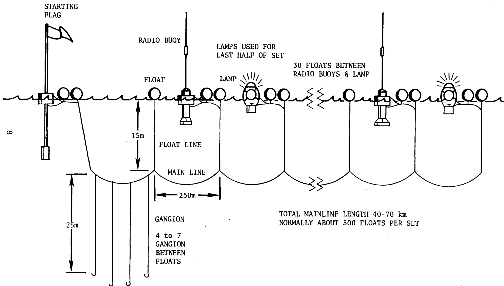
Figure 2. A typical Japanese longline set for tuna.
