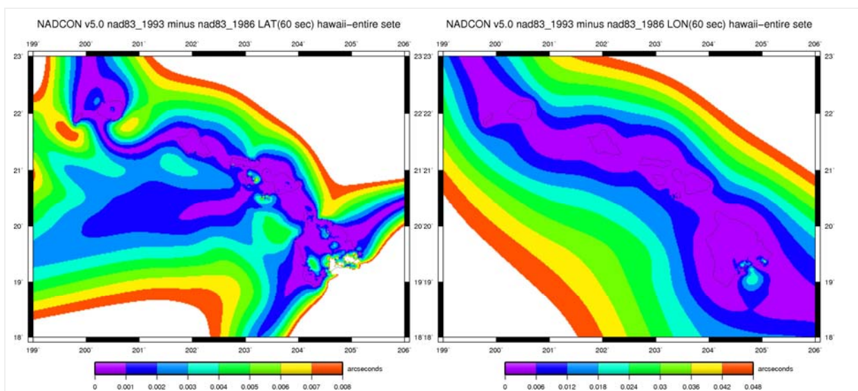
Figure 6-113: Errors for horizontal transformation, latitude (left) and longitude (right) components, in arcseconds for NAD 83(1986)/NAD 83(1993)/Hawaii.
