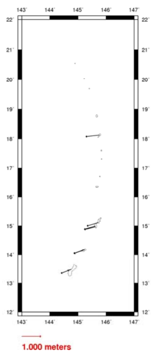
Figure 6-206: All horizontal vectors for NAD 83(1993)/NAD 83(2002)/Guam&CNMI.
