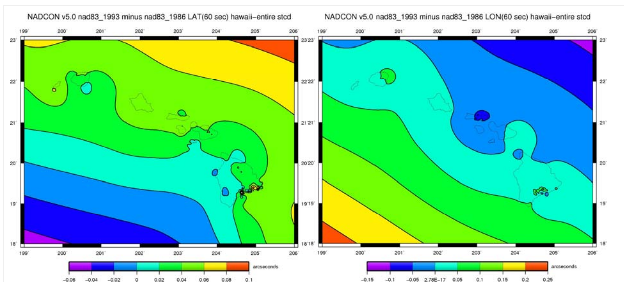
Figure 6-112: Horizontal transformation, latitude (left) and longitude (right) components, in arcseconds for NAD 83(1986)/NAD 83(1993)/Hawaii.
