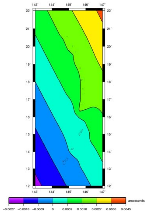
Figure 6-218: Horizontal transformation, latitude (left) and longitude (right) components, in arcseconds for NAD 83(2002)/NAD 83(MA11)/Guam&CNMI.
