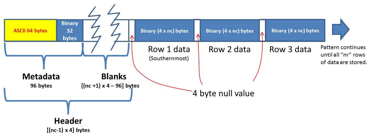
Figure 10-1: Contents of .las/.los format
