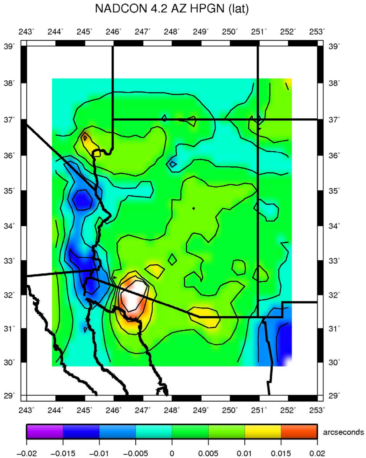
Figure 1-1: The Arizona HPGN latitude grid from NADCON 2.1 (and 4.2)
