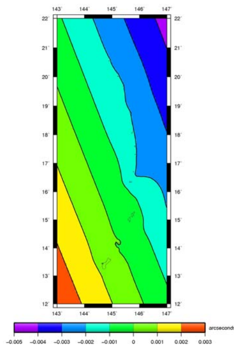
Figure 6-218: Horizontal transformation, latitude (left) and longitude (right) components, in arcseconds for NAD 83(2002)/NAD 83(MA11)/Guam&CNMI.
