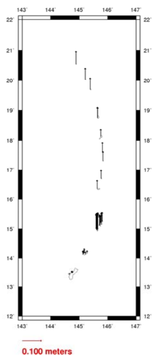
Figure 6-221: All vertical vectors for NAD 83(2002)/NAD 83(MA11)/Guam&CNMI.
