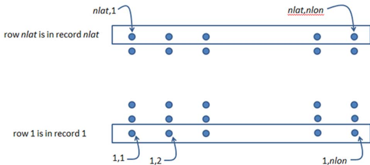
Figure 10-2: Details of data layout for .b format
