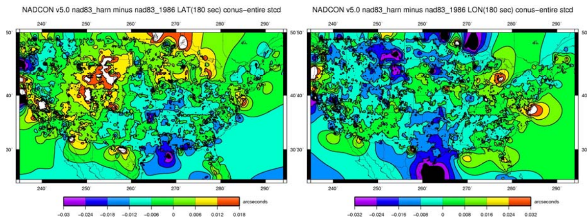
Figure 6-14: Horizontal transformation, latitude (left) and longitude (right) components, in arcseconds for NAD 83(1986)/NAD 83(HARN)/CONUS.
