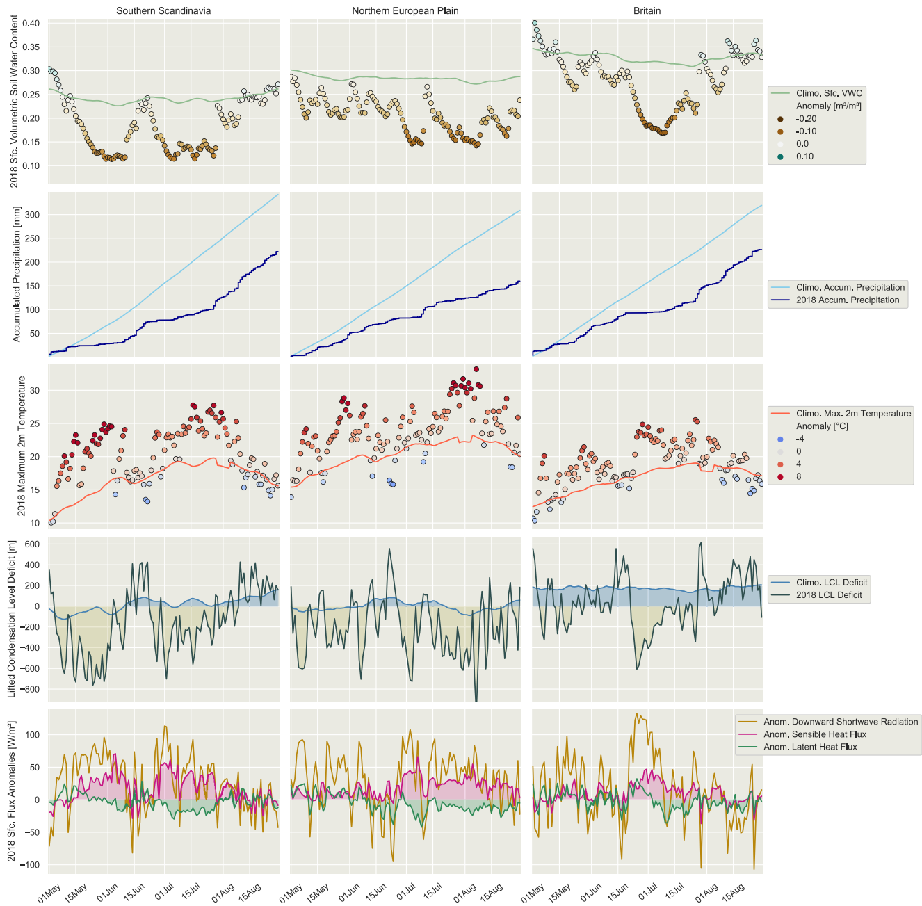
Figure 4. Area averages from ERA5 over land points in the indicated regions for daily surface layer VWC (top row), cumulative precipitation (second row), daily maximum 2 m air temperature (third row), LCL deficit (fourth row), and indicated surface energy balance terms (bottom row). In each panel, climatological values are indicated by a smooth (7-day centered running mean) line except in the bottom row where only anomalies are shown. In the first and third rows, color of dots indicates the magnitude of the anomaly.
