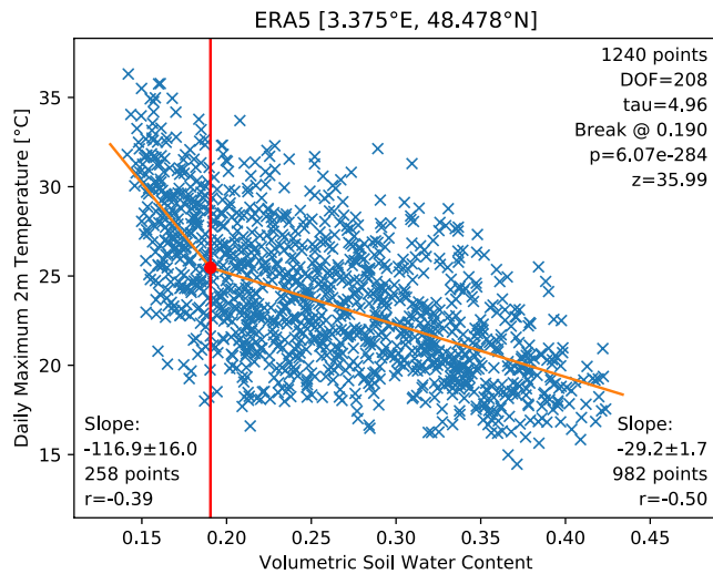
Figure 3. Relationship between daily maximum 2 m air temperature (dependent variable; ordinate) and surface VWC (abscissa) during July for 1979–2018 at a grid cell in France. Values in upper right refer to the total number of days (including VWC memory time scale “tau” in days and reduced degrees of freedom “DOF” due to VWC autocorrelation) and significance of the estimate of the threshold between two best fit linear regressions. Values in the lower corners show the estimated slopes \pm standard error of estimates, number of points, and correlations for each segment—the fits for each segment are significant at the 99% confidence level.
