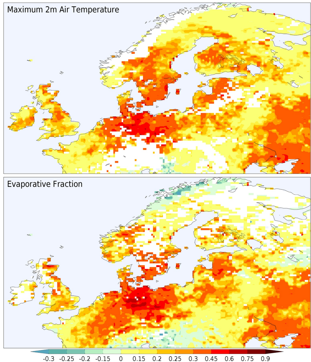
Figure 7. Increase in the fraction of days during May to August 2018 on the dry side of the surface VWC threshold based on ERA5 daily maximum temperature (top) and evaporative fraction (bottom) compared to the 1979–2018 average. Masked areas fail to meet the screening criteria described in Section 3 in all 4 months.
