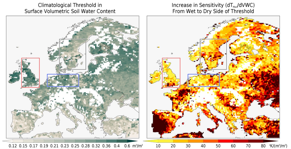
Figure 5. Left: Values of VWC estimated to be at the threshold regarding a significant change in the slope of the regression of daily maximum 2 m air temperature on VWC. Right: Change in the slope of the regression across the threshold. White areas fail to pass at least one of the criteria described in Section 3, with additional criteria that areas of organic (peat) soils are excluded and the estimated value of the maximum temperature at the threshold exceeds 10°C.
