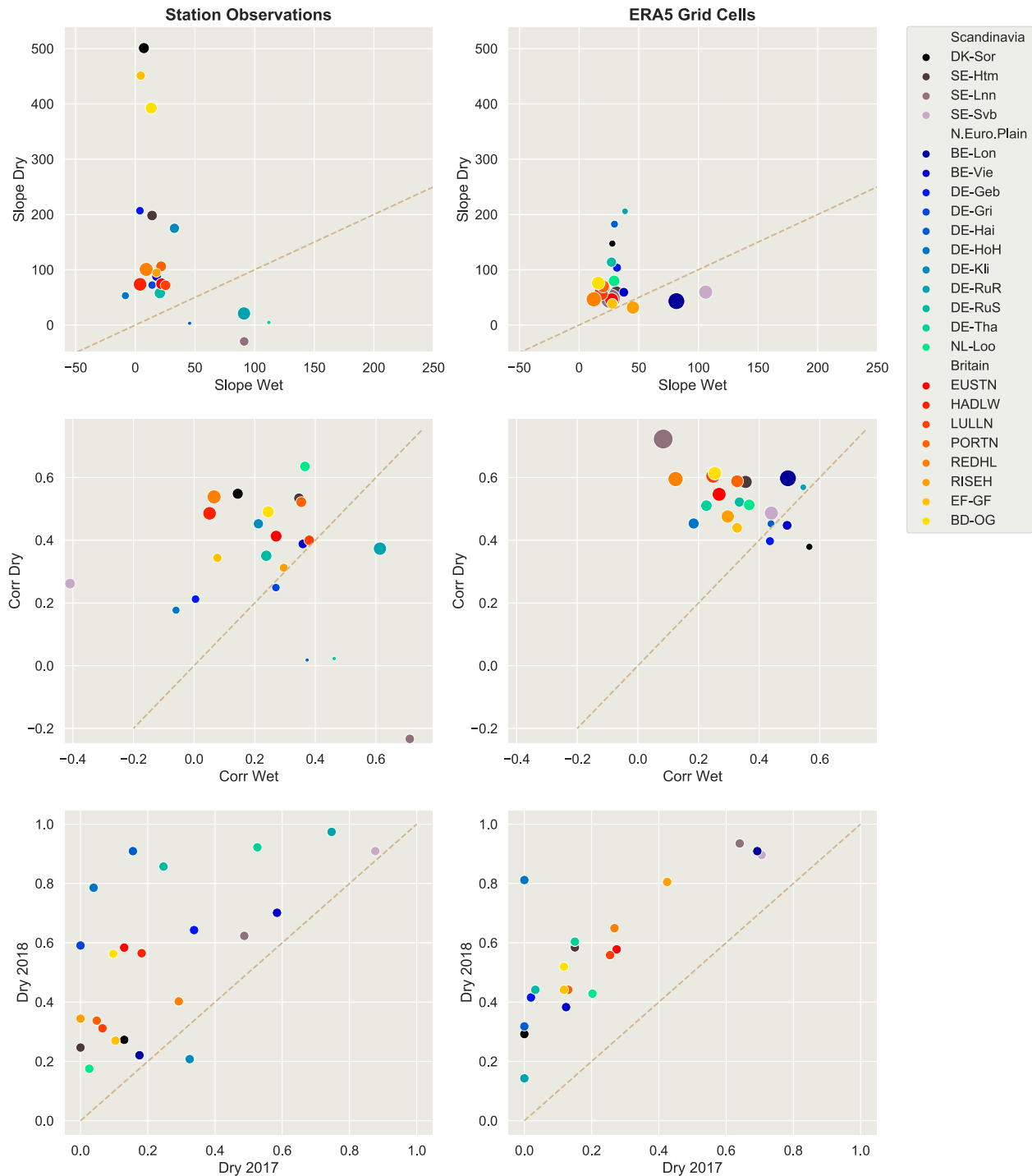
Figure 6. Relationships for in situ stations (left column) and their corresponding ERA5 grid cells (right column) between the sensitivity (slope; K/[m^3m^{-3}] ) dT_{Max}/dSM on the wet and dry sides of the thresholds (top); correlation of the points in the linear regression of T_{Max} on SM on each side of the threshold (middle); Fraction of days during MJJA on the dry side of the threshold during the period 15 May through 15 October in 2018 versus 2017 (bottom). In the first two rows, slopes and correlations are multiplied by -1 for clarity, and the size of the symbol is proportional to the confidence in the dry-side slope defined as the slope divided by the standard error in the estimation of the slope.
