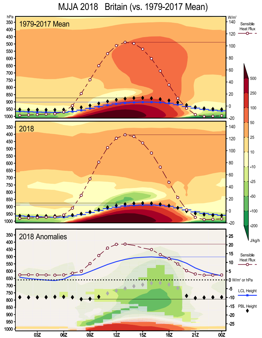
Figure 8. Time-height (model pseudo-pressure coordinate, scale on the left; see Section 2 for details) diagram of hourly heat budget terms averaged over land grid cells of Britain (red box in Figure 1) from ERA5 data. Shading is total diabatic heating per hour—insignificant anomalies for 2018 are grayed out in the bottom panel. Lines and/or symbols show surface sensible heat flux, LCL height, and PBL height as indicated, and thin horizontal lines mark daily extremes tailing to the appropriate scale. In the bottom panel, faint or missing hourly markers indicate lack of significance of the anomaly. All significances are at 95% confidence levels.
