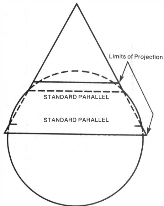
Figure 8.—Sphere and intersecting cone illustrating the Lambert conformal conic projection
