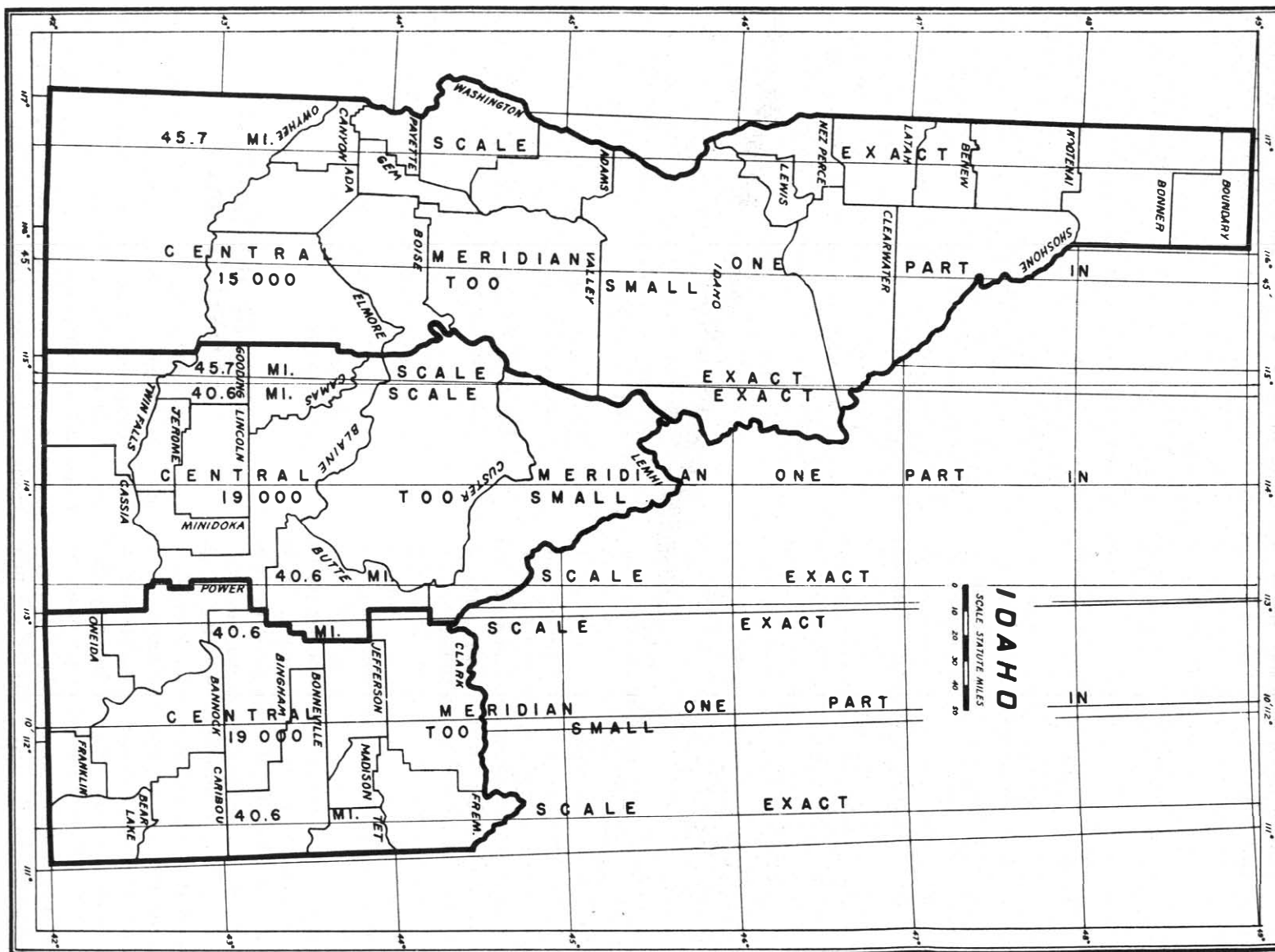
Figure 9.—Use of transverse Mercator projection for plane coordinate zones in Idaho
