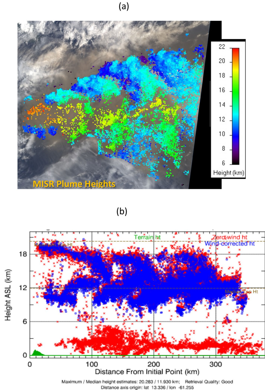
Figure 1. (a) Multi-angle Imaging SpectroRadiometer (MISR) stereo-derived plume-height map showing the La Soufriere eruption plume at \sim 1435 UT on 10 April 2021. (b) Downwind profile plot of the same plume. Red points are derived from the parallax of plume contrast elements in the MISR multi-angle imagery; blue points present the heights corrected for any proper motion of plume elements. The surface elevation is indicated in green.
