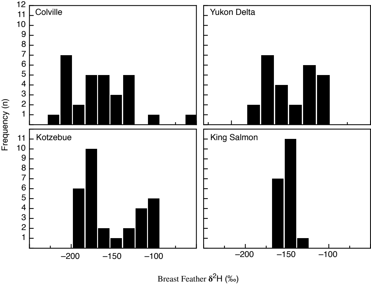
Figure S1. Distributions of individual breast feather δ²H values within breeding areas
