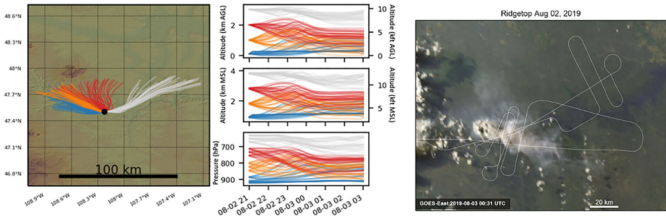
Figure 16. Left: Smoke trajectory ensemble forecast for the Ridgetop fire in Montana for multiple potential smoke injection altitudes in which low-level trajectories depict extensive vertical plume spreading to the north and northwest (blue, orange, and red lines) while high-level trajectories show horizontal plume confinement to the east (gray lines). (Above Ground Level (AGL), Mean Sea Level (MSL)). Right: Satellite image of smoke distribution at the time of aircraft sampling (gray line), showing diffuse low-level smoke transported to the north and high-elevation smoke outflow from pyroconvection transported to the east.
