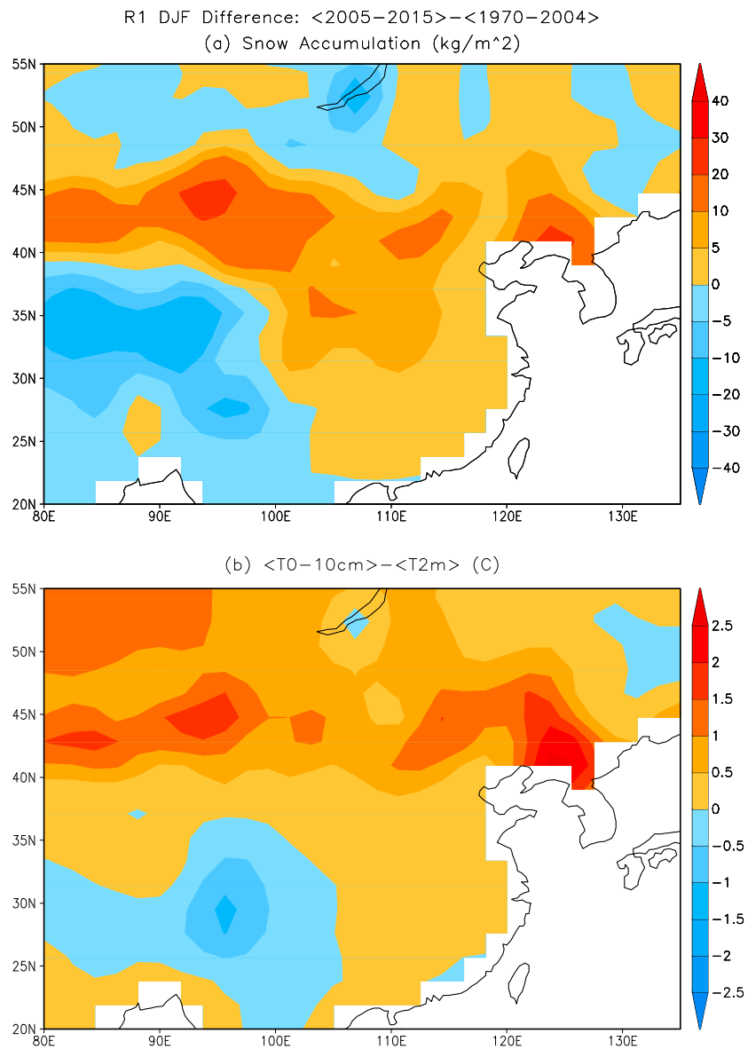
Figure 8. Difference of (a) water equivalent of surface accumulated snow depth (kg/m 2 ) and (b) soil temperature at 0–10 cm minus air temperature at 2 m (°C) between 1970–2004 and 2005–2015 in NCEP/NCAR reanalysis data.
