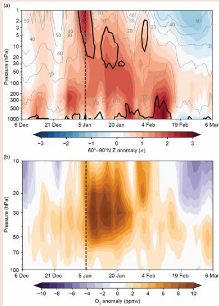
Fig. SB5.3. The vertical coupling for 30 days before to 60 days after the 5 January 2021 SSW, shown as pressure–time cross-sections of daily-mean (a) 60°–90°N geopotential height anomalies (std. dev.; shading) and 60°N zonal-mean zonal winds ( \text{m s}^{-1} ; gray contours, with the zero wind line in black) from the ERA5 reanalysis, and (b) 65°–90°N ozone anomalies (ppmv) from the MERRA2 reanalysis. All anomalies are created with respect to the daily climate over 1991–2020. The geopotential height anomalies are additionally normalized at each pressure level by the standard deviation of all days in the 90-day window shown during 1991–2020. The dashed black vertical line indicates the date of the SSW.
