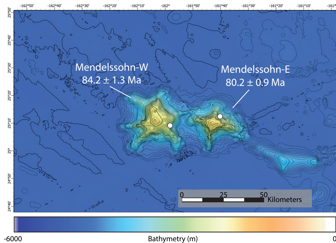
Figure 5. A bathymetric map shows the Mendelssohn Seamounts, which are composed of the Mendelssohn East and Mendelssohn West seamounts. The locations of two dredges are shown with white circles, and the corresponding ^{40}\text{Ar}/^{39}\text{Ar} ages are shown (Sager and Pringle, 1987).
