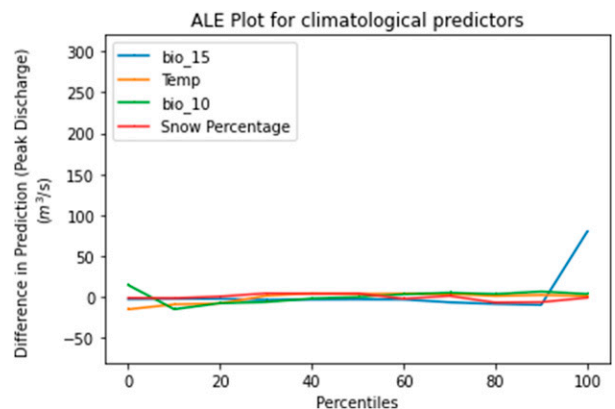
FIG. 9. ALE analysis for climatological predictors.
