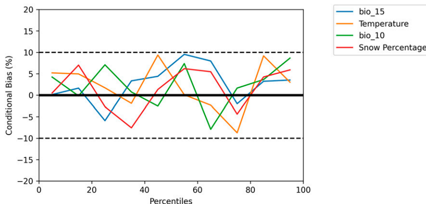
FIG. 6. Conditional bias for climatological predictors.
