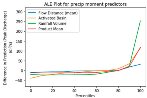
FIG. 8. ALE analysis for precipitation spatiotemporal variability predictors.
