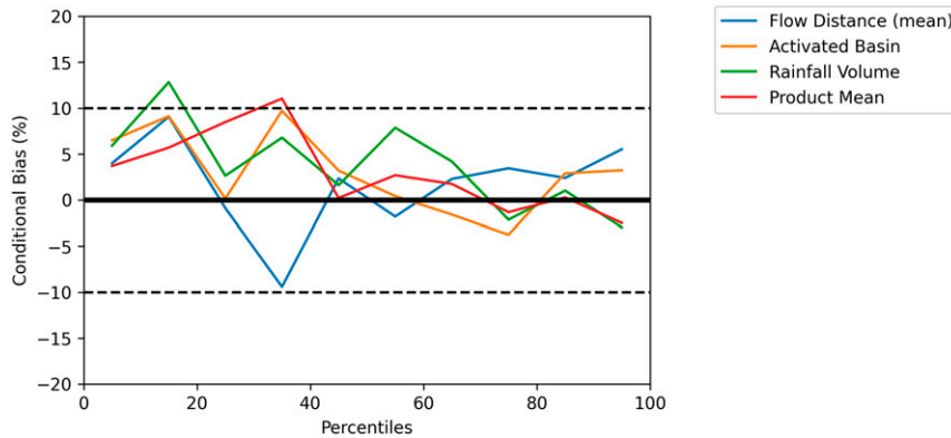
FIG. 5. Conditional bias for precipitation spatiotemporal variability predictors.
