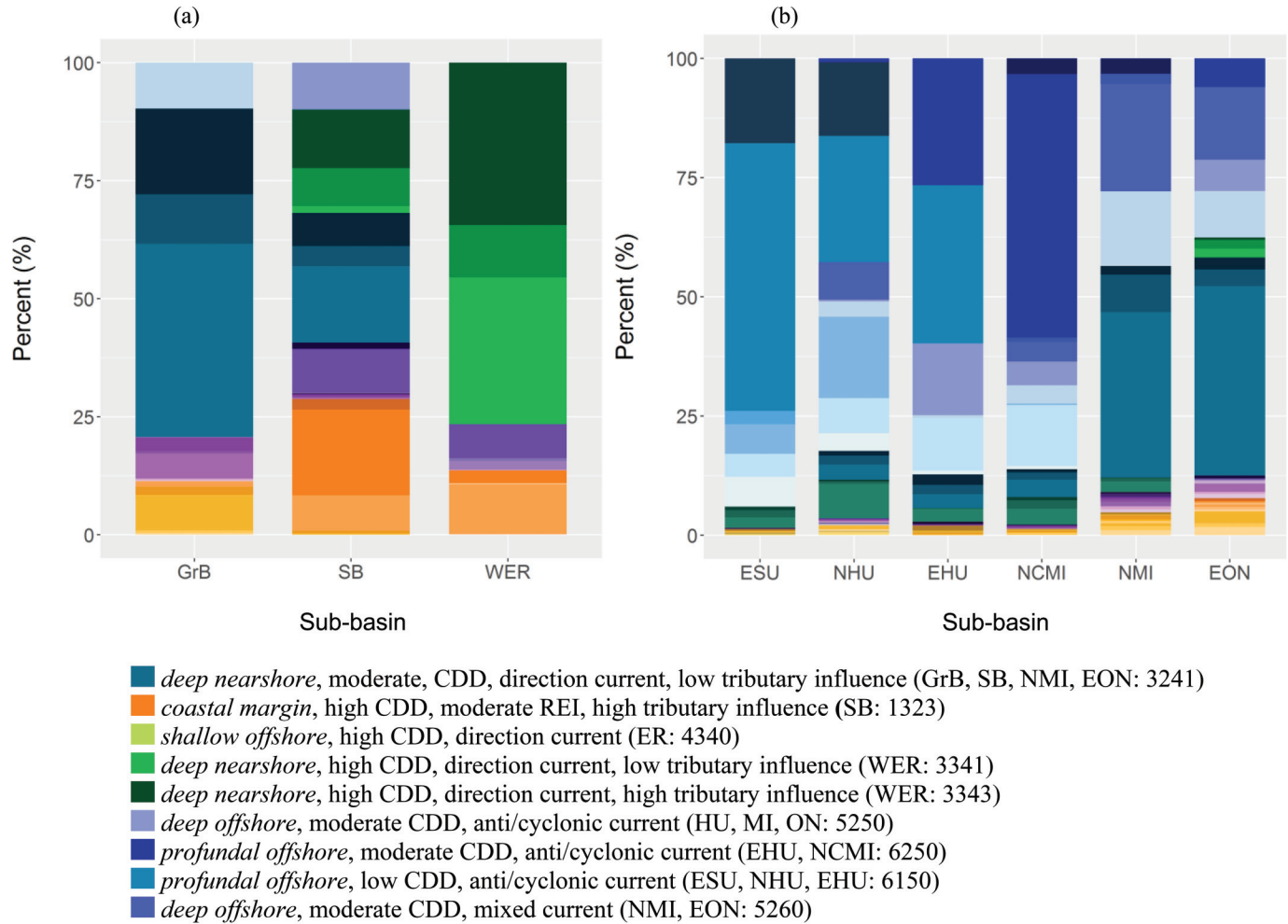
Fig. 6. Bar graphs illustrating the proportion of different aquatic ecological units (AEUs) across five focal areas mapped in Fig. 5; the color codes match the codes for the AEUs in Fig. 3. (a) Comparison of Green Bay (GrB, Lake Michigan), Saginaw Bay (SB, Lake Huron), and western sub-basin of Lake Erie (WER). (b) Comparison of the eastern sub-basin of Lake Superior (ESU), northern and eastern sub-basins of Lake Huron (NHU, EHU), north-central and north sub-basins of Lake Michigan (NCMI, NMI), and eastern Lake Ontario with Bay of Quinte (EON). Lake codes are in Fig. 1. The color codes match the codes for AEU types in Fig. 3. For reference, the dominant AEU types in this figure are listed in the figure legend.
