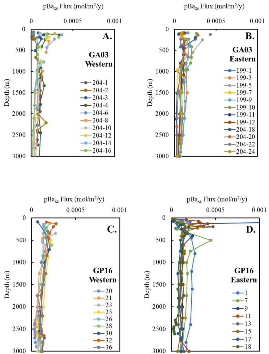
Figure 3. ^{230}\text{Th} -normalized \text{pBa}_{\text{xs}} flux in the water column in the western (a) and eastern (b) basins of GA03. Corresponding ^{230}\text{Th} -normalized \text{Ba}_{\text{xs}} flux at stations in the western (c) and eastern (d) basins of GP16 (the maximum flux at station 9, 0.0025 \text{ mol m}^{-2} \text{ year}^{-1} , is off scale).
