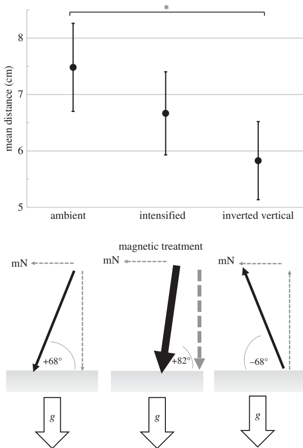
Figure 1. Mean height of fish movement ( y -axis) under different magnetic conditions. Error bars indicate the 95% confidence interval of the mean. Significant differences between treatments are indicated by an asterisk (Mann–Whitney U -test, U = 29871 , p = 0.0036 ). Beneath the graph is a schematic of the magnetic conditions experienced by fish. The geomagnetic vector is shown by a black arrow; the horizontal and vertical components of the field are grey dashed arrows (arrow thickness shows relative intensity). Magnetic north is designated by 'mN'. The gravity vector is shown as a white arrow, 'g'.
