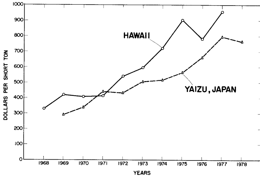
Figure 5.--Ex-vessel value of skipjack tuna landed in Yaizu, Japan, 1969-78, and in Hawaii, 1968-77. (Data from [U.S.] National Marine Fisheries Service 1969-1978 and Hawaii Division of Fish and Game see text footnote 1.)
