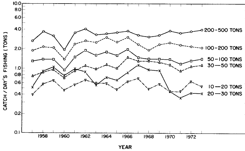
Figure 6.--Catch per day's fishing by vessel size classes in the Japanese skipjack tuna pole-and-line fishery. (From Ishida 1975.)
