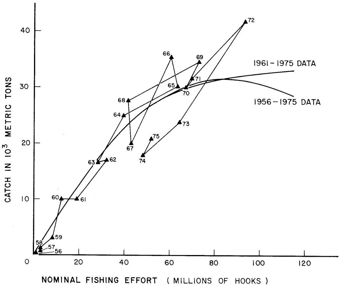
Figure 5. Production model results for south Atlantic albacore.
