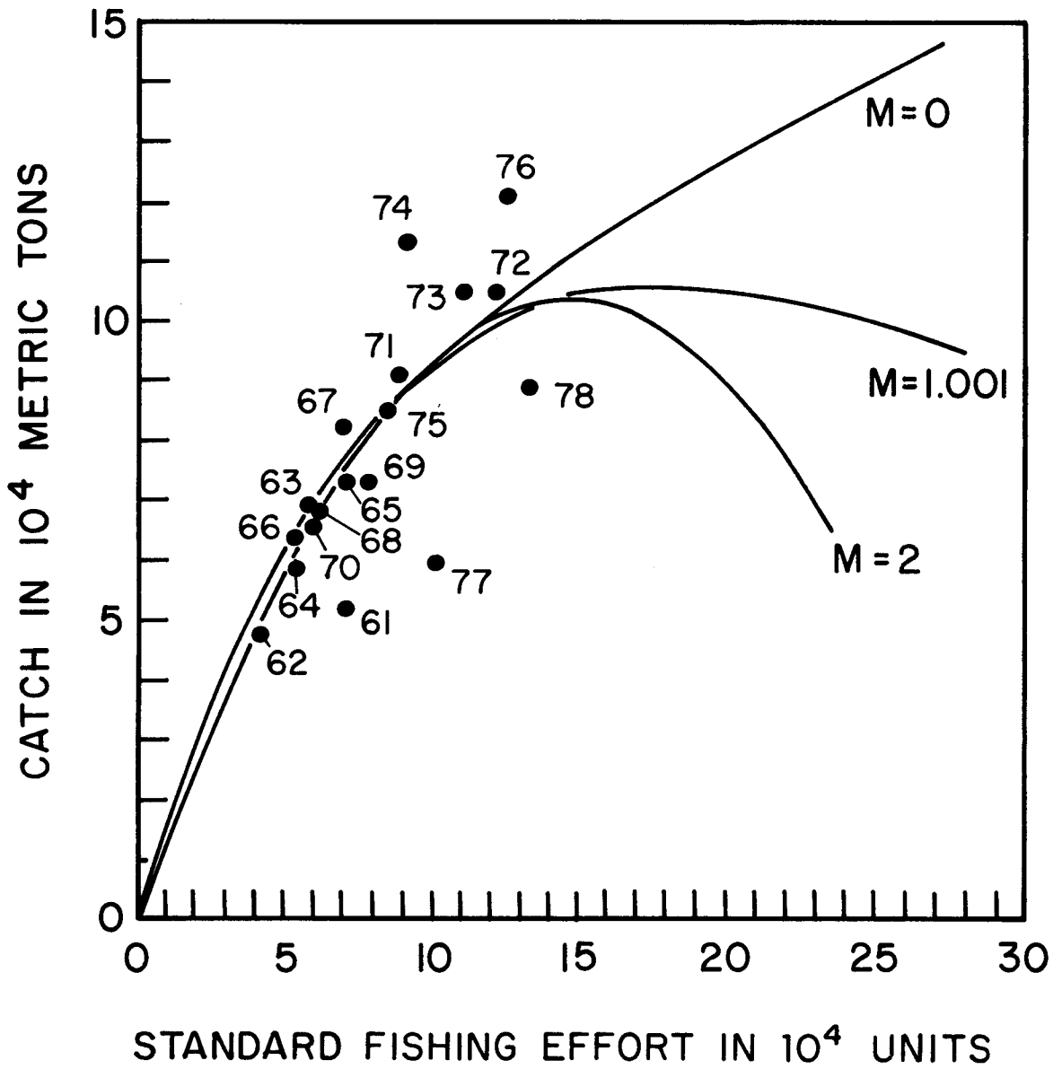
Figure 5. Equilibrium yield curves and observed data for North Pacific albacore, years 1961 to 1978.
