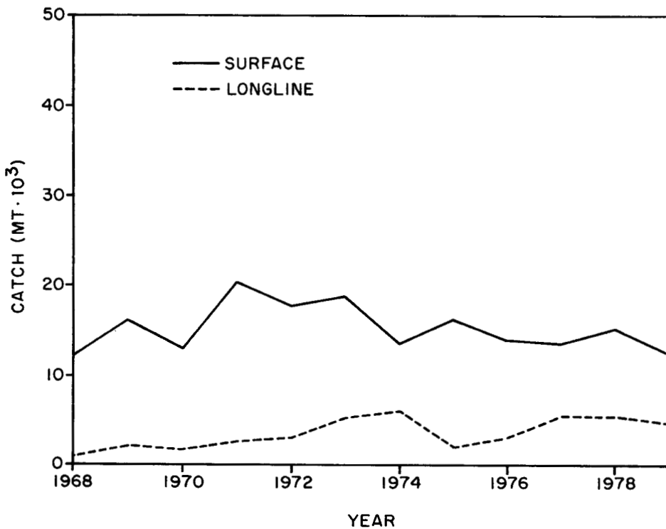
Figure 3. a) Total catch of bigeye tuna from surface and longline gears fishing in the northern Atlantic, 1968 to 1979. b) Total catch of bigeye tuna from surface and longline gears fishing in the southern Atlantic, 1968 to 1979.
