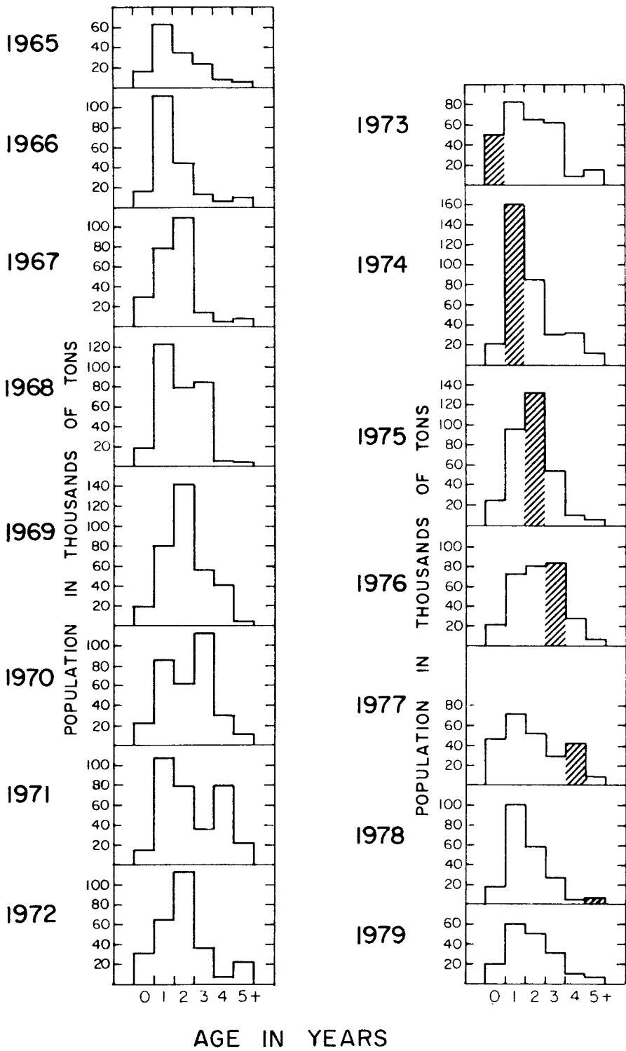
Figure 8. Annual biomass estimates of yellowfin in the CYRA by age groups, 1965 to 1979.
