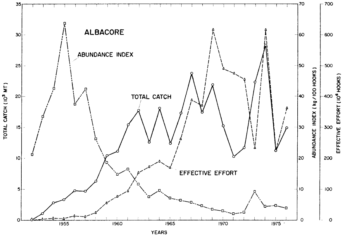
Figure 7. Estimated total catch ( 10^3 MT), relative abundance (kg/100 hooks), and effective effort ( 10^6 hooks) for Indian Ocean albacore.
