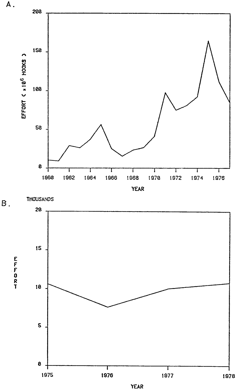
Figure 4. a) Fishing effort in hooks for the longline fishery in the northern Atlantic, 1960 to 1977. b) Effort in days at sea for the Canary Island bait-boat fleet, 1975 to 1978.
