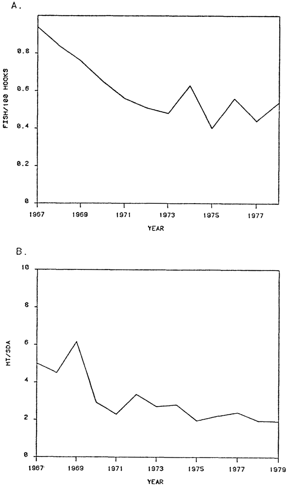
Figure 7. a) Catch-per-unit-effort (number of fish/100 hooks) from the Atlantic longline fishery for yellowfin tuna, 1967 to 1978. b) Catch-per-unit-effort (metric tons/standard purse seine days absence) from the eastern Atlantic surface fishery for yellowfin tuna, 1967 to 1979.
