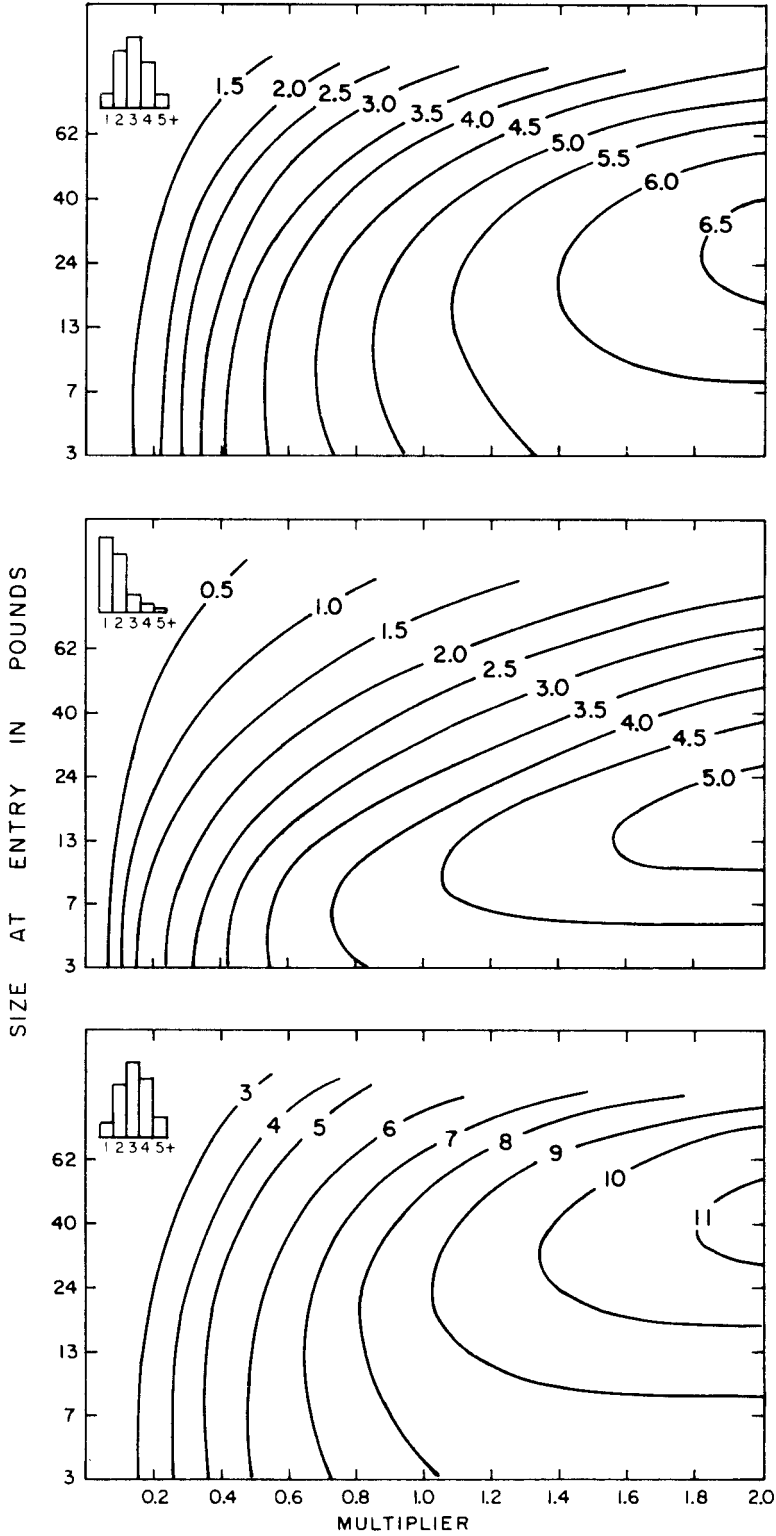
Figure 7. Yield-per-recruit isopleths for yellow-fin tuna inside the CYRA; a) based on the age structure of the catch during the period 1968 to 1972 and natural mortality rate M=0.8 , b) based on the age structure during the period 1973 to 1978 and M=0.8 , c) based on the age structure during the period 1968 to 1972 and M=0.6 .
