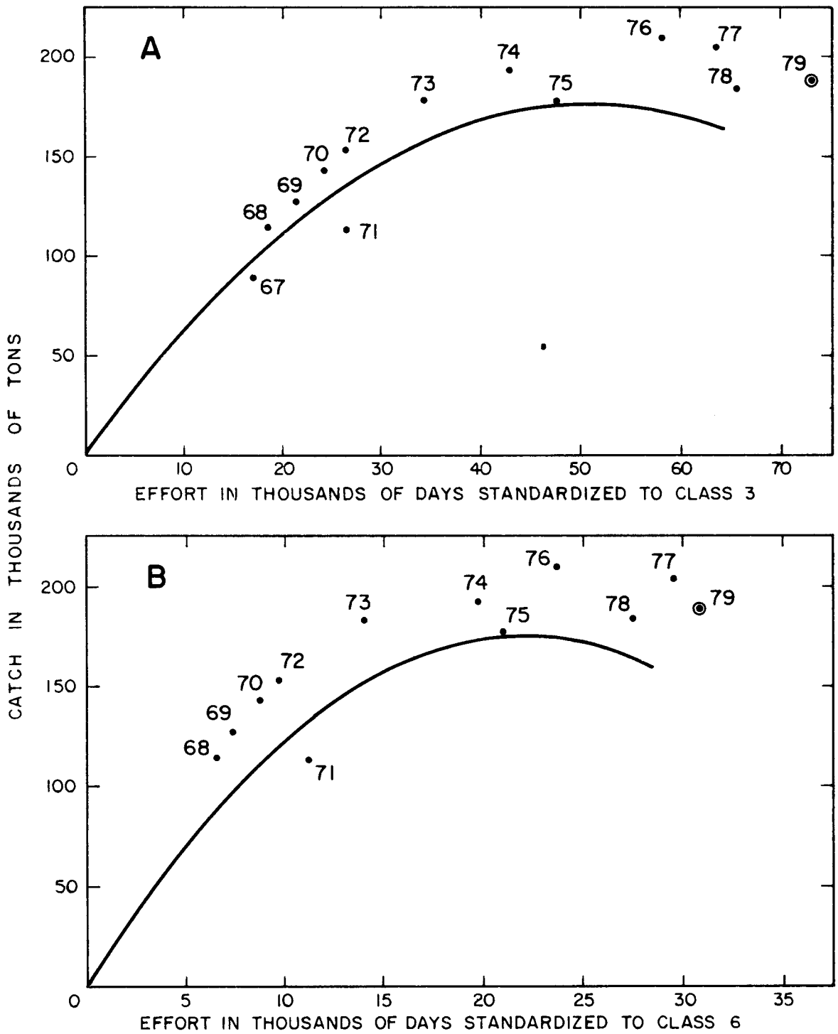
Figure 5. a) Equilibrium catch curve for the yellowfin tuna fishery inside the CYRA, 1967 to 1979. Effort in days fishing is standardized to Class 3 purse seiners. b) Equilibrium catch curve for the yellowfin tuna fishery inside the CYRA, 1968 to 1979. Effort in days fishing is standardized to Class-6 purse seiners.
