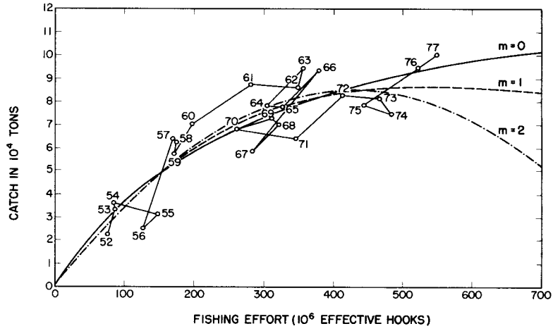
Figure 6.--Catch and effort plots with curves fitted to the model for m = 0, 1, \text{ and } 2 ( k = 3 ), respectively, for yellowfin tuna caught in the Pacific-wide longline fishery, 1952-77. (From FAO in press.)
