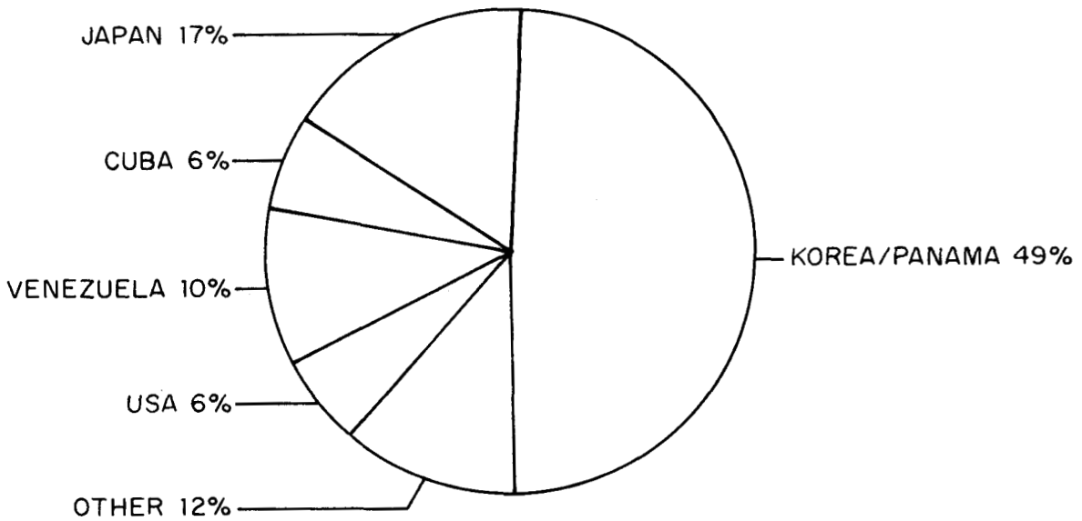
Figure 2. a) Major participants in the eastern Atlantic surface and long-line fishery for yellowfin tuna, 1975 to 1979.
