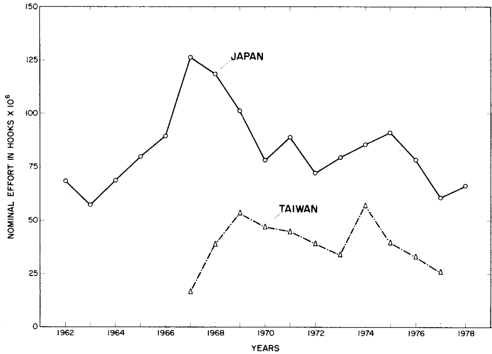
Figure 6. Nominal effort in 10^6 hooks by Japanese and Taiwan longline vessels in the Indian Ocean. (Japanese data from Fisheries Agency of Japan, Research Department 1980 and Taiwan data courtesy of R. T. Yang, National Taiwan University, Taiwan, Republic of China.)
