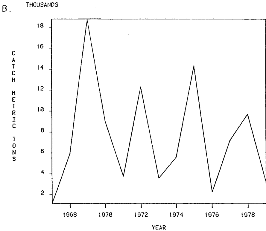
Figure 6. a) Total fishing effort in number of U.S. vessels fishing in the Atlantic Ocean, 1967 to 1979. b) Total catch of yellowfin tuna for U.S. vessels fishing in the Atlantic Ocean, 1967 to 1979.
