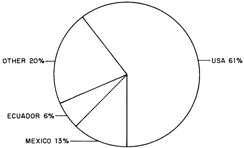
Figure 2. Major participants in the eastern tropical Pacific Ocean yellowfin tuna fishery based upon percent of total catch in 1979.
