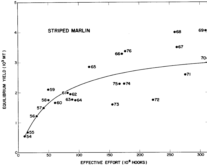
Figure 9.--Predicted relationship between equilibrium yield (10 3 MT) and effective effort (10 6 hooks) for Indian Ocean striped marlin, based on production model analysis. (From Wetherall et al. see text footnote 1.)
