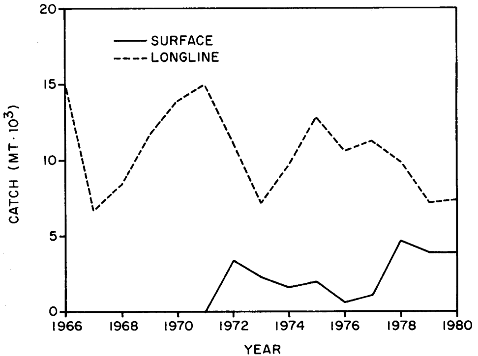
Figure 3. a) Total catch of yellowfin tuna using surface and longline fishing gear in the eastern Atlantic, 1966 to 1980. b) Total catch of yellowfin tuna using surface and longline fishing gear in the western Atlantic, 1966 to 1980.
