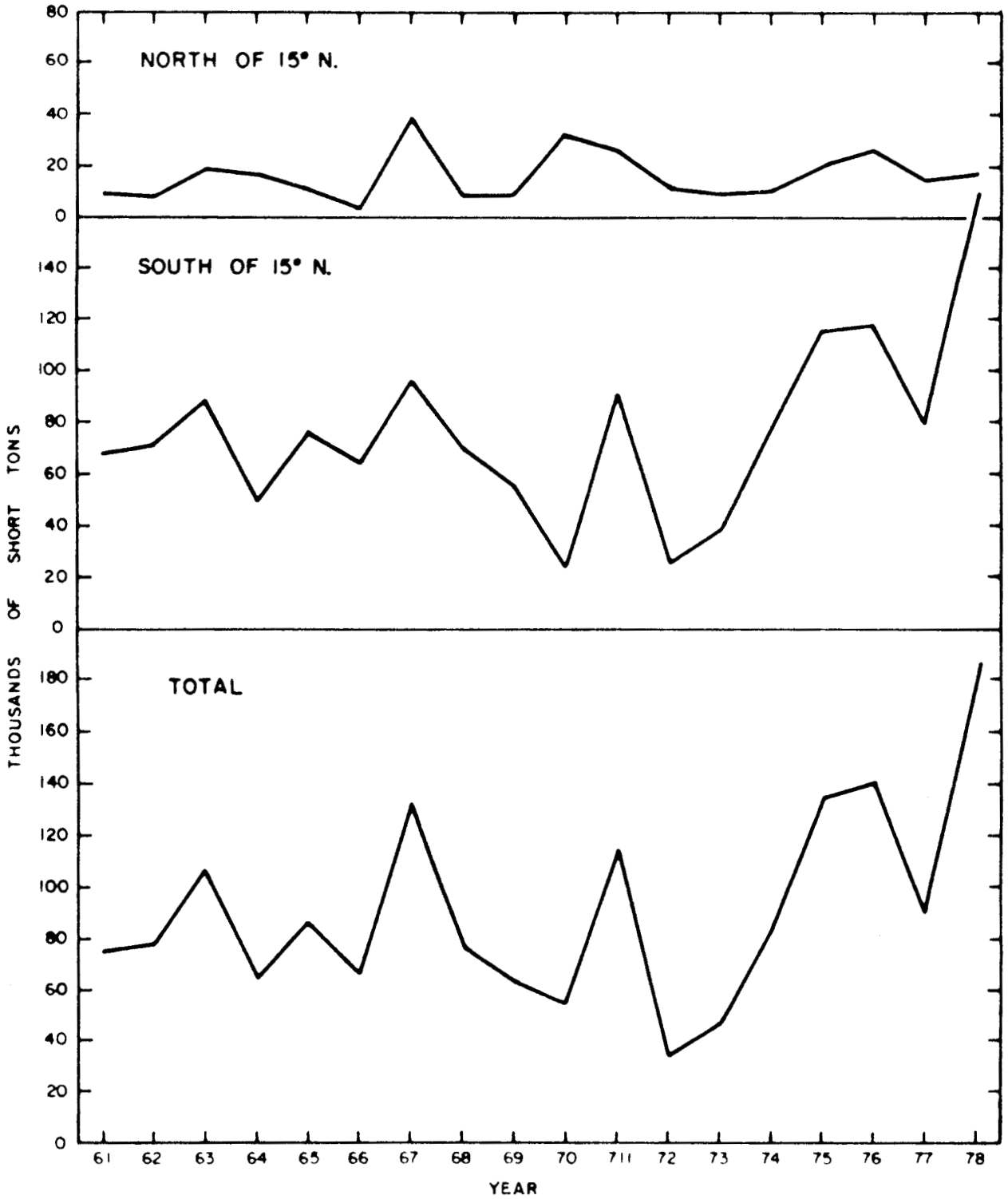
Figure 4. Estimated CYRA catches of skipjack north and south of 15° N, 1961-1978.
