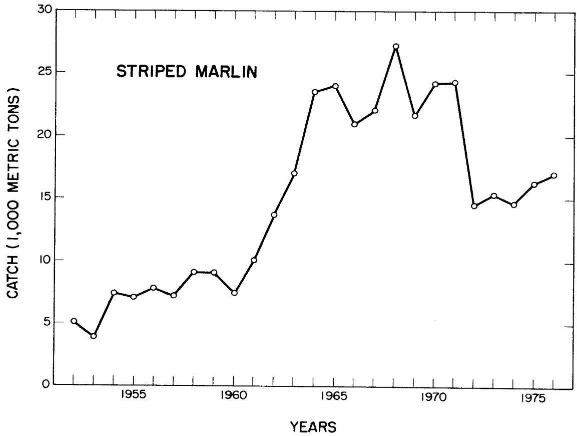
Figure 7.--Pacific catch of striped marlin, 1952-76. (Data from Table 2.)
