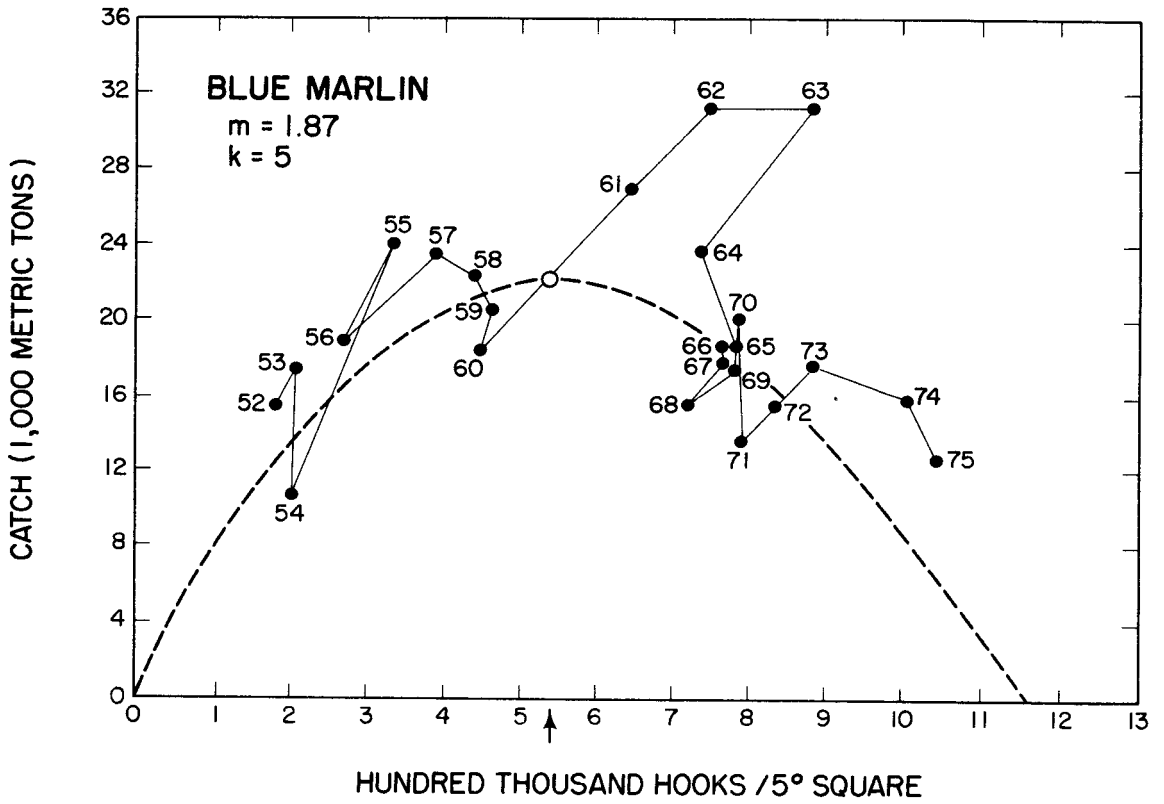
Figure 11.--Relation between catch of blue marlin and effective fishing effort. The equilibrium yield curve is based on the production model. (From Shomura 1980.)
