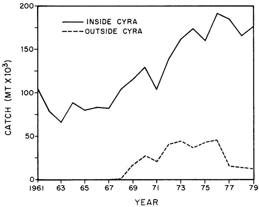
Figure 3. Catches of yellowfin tuna from inside the CYRA and outside the CYRA in the eastern tropical Pacific Ocean.
