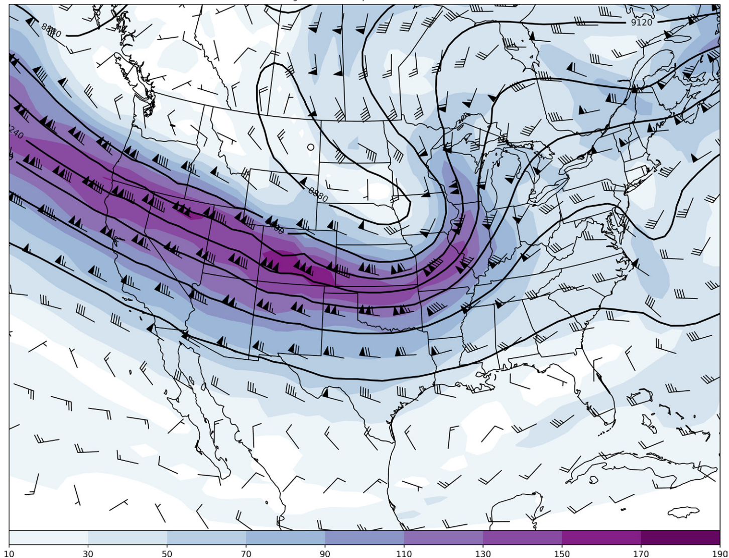
Fig. 5. Geopotential heights (contoured; m), wind speed (filled contours; kt), and wind barbs (kt) from Global Forecast System output valid at 1200 UTC 31 Oct 2010. Example analysis produced using MetPy's declarative plotting syntax demonstrated in Fig. 4.
