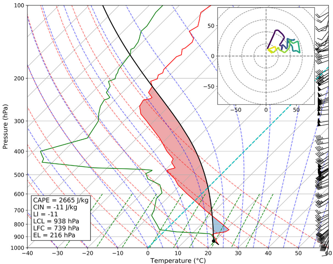
Fig. 1. Vertical profile of the atmosphere, valid 1200 UTC 22 May 2011 from Topeka (TOP), presented on a skew T - \log p diagram. Shown are observed temperature (red line), dewpoint temperature (green line), calculated parcel profile trace (black line), 0°C isotherm (cyan line, dashed), and wind barbs (right axis; kt; 1 kt \approx 0.51 m s -1 ), with shaded areas for CIN (blue shaded) and CAPE (red shaded). Calculated indices are inset at the bottom left, and a hodograph is presented in the top right, colored by altitude.
