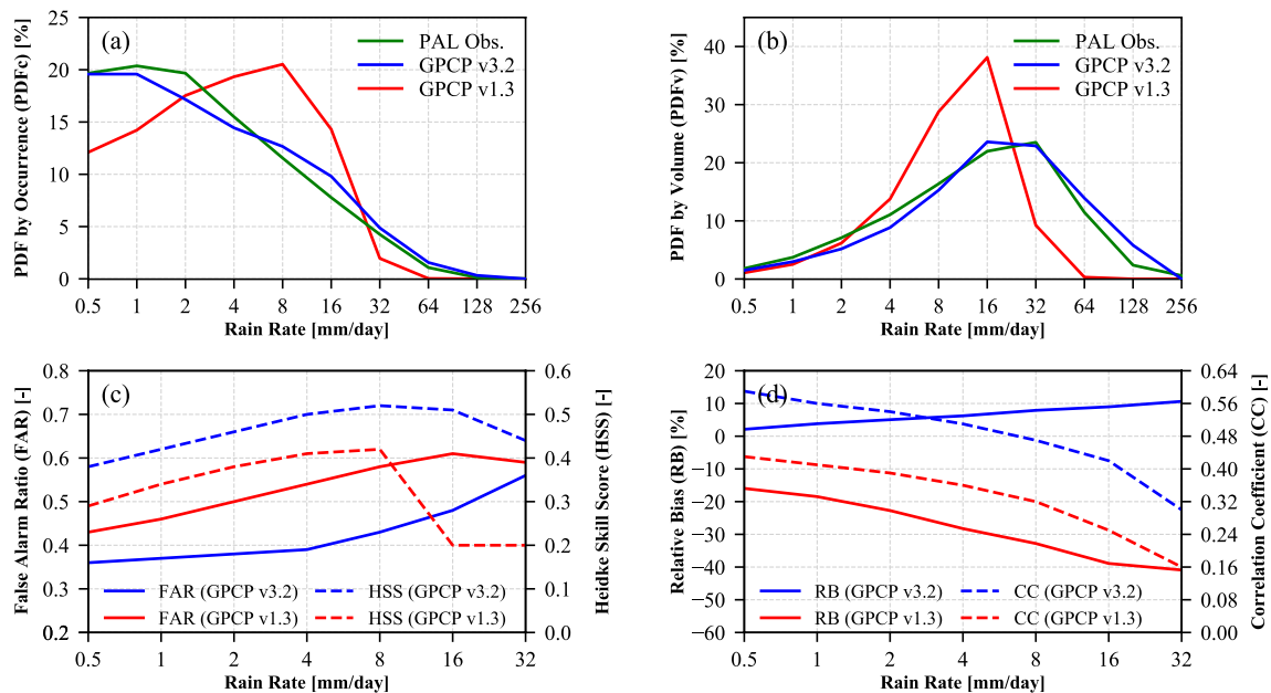
Figure 5. Comparison of (a) probability distribution function by occurrence (PDFc), (b) probability distribution function by volume (PDFv), (c) rainfall detection skills (false alarm ratio and Heidke skill score), and (d) estimation metrics (relative bias and correlation coefficient) as a function of daily rainfall intensity for Global Precipitation Climatology Project products.
