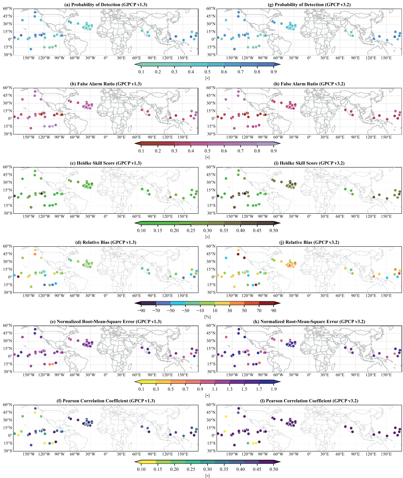
Figure 4. Spatial maps of (a, g) probability of detection, (b, h) false alarm ratio, (c, i) Heidke skill score; and conditional (d, j) relative bias, (e, k) normalized root-mean-square error, and (f, l) Pearson's correlation coefficient for daily Global Precipitation Climatology Project (GPCP) v1.3 (left panels) and GPCP v3.2 (right panels) estimates against Passive Aquatic Listeners (PALs). The circles represent the drifting end location of PALs, and rain detection threshold is 0.5 mm/day.
