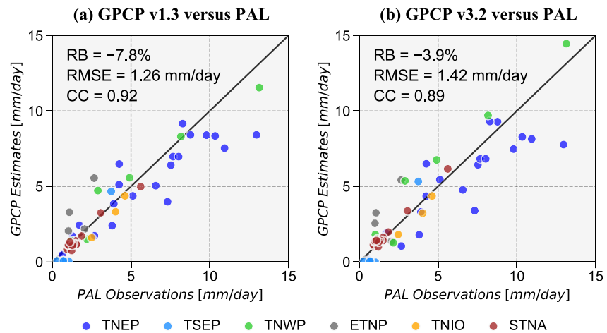
Figure 2. Scatterplots comparing the multi-year mean rain rates (mm/day) estimated by (a) Global Precipitation Climatology Project (GPCP) v1.3 and (b) GPCP v3.2 against Passive Aquatic Listener (PAL) observations. Each data point corresponds to one PAL, and the color indicates its group by region.
