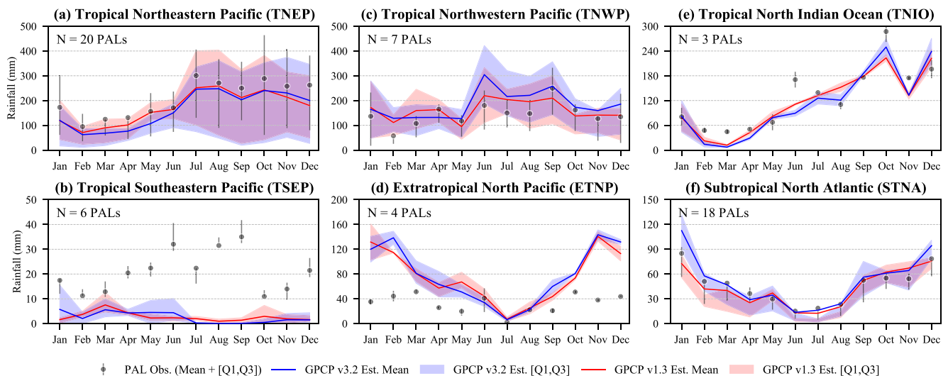
Figure 3. Intra-annual distributions of monthly rainfall estimated from Global Precipitation Climatology Project (GPCP) v1.3, GPCP v3.2 and Passive Aquatic Listener (PAL) over different regions (as shown in Figure 1). The comparison includes the mean, and interquartile range (IQR, i.e., the difference between 25% and 75% quantile, [Q1, Q3]) estimates of monthly rainfall, which are calculated from N PALs within each region. Here, N represents the number of PALs.
