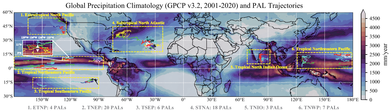
Figure 1. The trajectories of 58 Passive Aquatic Listeners (PALs) used in this study, on the global precipitation climatology map derived from Global Precipitation Climatology Project v3.2 (2001–2020). Different colors are used for individual PALs to enhance visibility. The two white triangles in the zoomed-in inset show the fixed locations of PALs (on buoy moorings) that were deployed in the tropical Eastern Pacific during SPURS-2.
