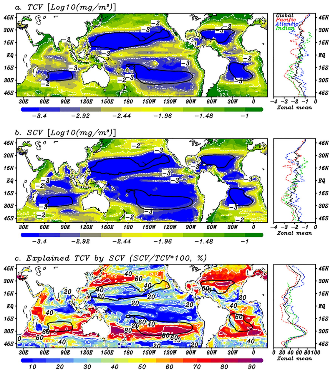
Figure 1. Seasonal cycle controls first order total chlorophyll variance (TCV) in the mid latitude. (a) Log 10 -transformed TCV from September 1997 to August 2021 (Equation 1), (b) Log 10 -transformed seasonal cycle (SCV) from September 1997 to August 2021 (Equation 3). TCV and SCV are calculated in original scale of chlorophyll (mg/m 3 ) and then transformed to log 10 to represent in global as shown in figures. (c) Explained TCV by seasonal cycle (SCV/TCV*100), which is calculated based on original scale of chlorophyll (mg/m 3 ). Black contour line denotes the edge of oligotrophic waters defined as below 0.07 mg/m 3 of mean annual chlorophyll.
