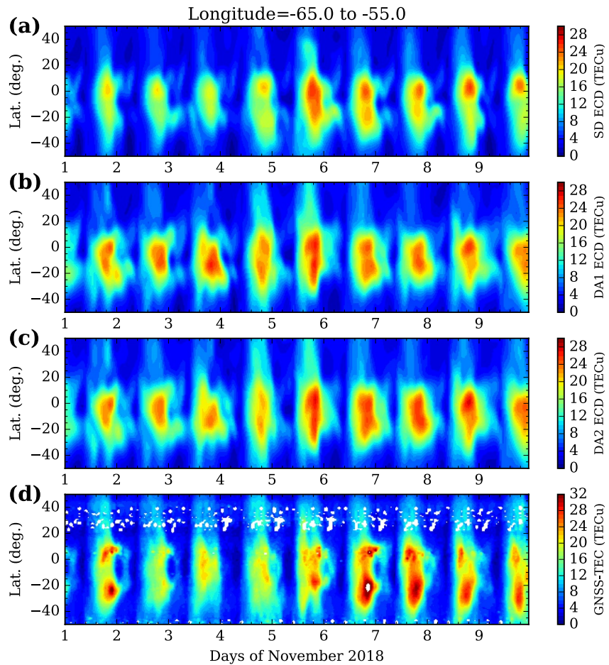
Figure 6. Latitude and day-to-day variability of SD electron column density (ECD) (a), DA1 ECD (b), DA2 ECD (c), and global navigation satellite system total electron content (d) averaged over 55°W to 65°W longitude.
