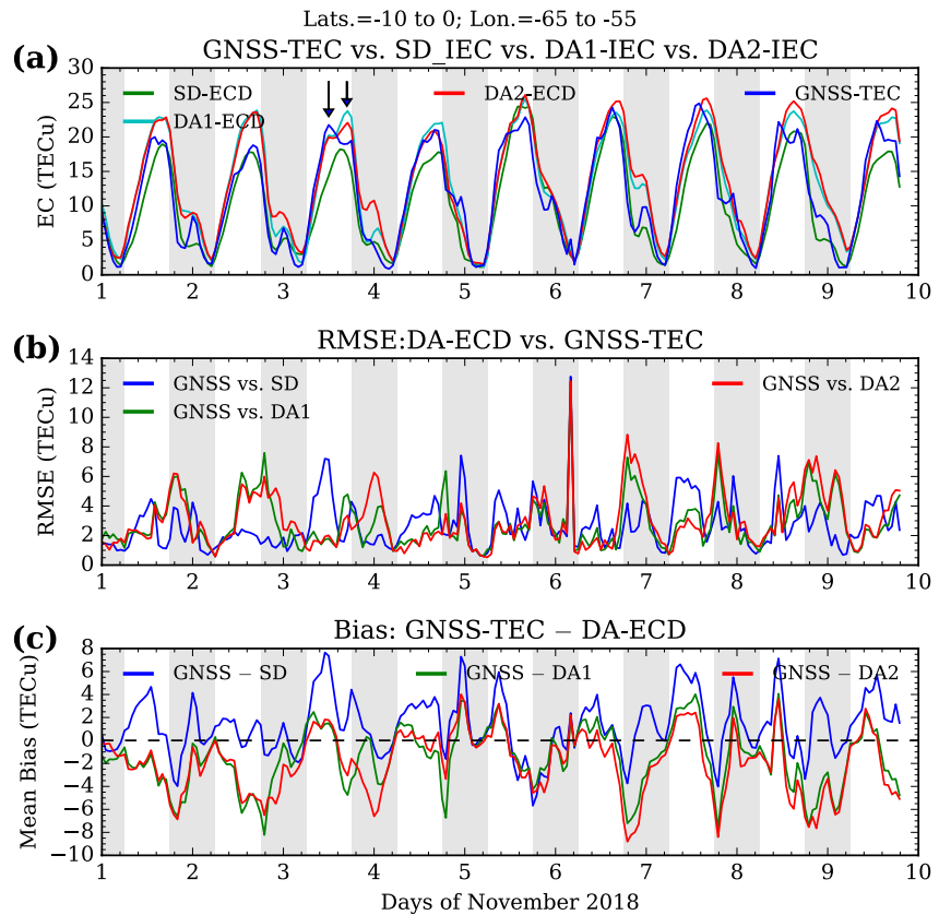
Figure 7. (a) Comparison of the SD electron column density (ECD) (green), DA1 ECD (cyan), DA2 ECD (red), and Global Navigation Satellite System Total Electron Content (GNSS-TEC) (blue) which are averaged over 10°S to 0°N and 55°W to 65°W. (b) RMSEs in GNSS-TEC versus SD ECD (blue), GNSS-TEC versus DA1 ECD (green), and GNSS-TEC versus DA2 ECD (red). (c) Mean bias in GNSS-TEC versus SD ECD (blue), GNSS-TEC versus DA1 ECD (green), and GNSS-TEC versus DA2 ECD (red) are shown. Two dashed arrows in (a) indicate example two-peak structure. The shaded regions represent nighttime, when Global-Scale Observations of Limb and Disk data are not assimilated.
