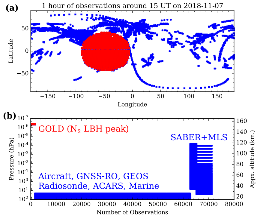
Figure 1. (a) Geo-locations, (b) altitude or pressure and number of observations that are assimilated successfully during a representative hour on a particular day are shown. The red points show the Global-scale Observations of Limb and Disk observations and blue points are the rest of the observations, which we term as lower atmosphere observations including SABER and MLS. MLS, Microwave Limb Sounder; SABER, Sounding of the Atmosphere using Broadband Emission Radiometry.
