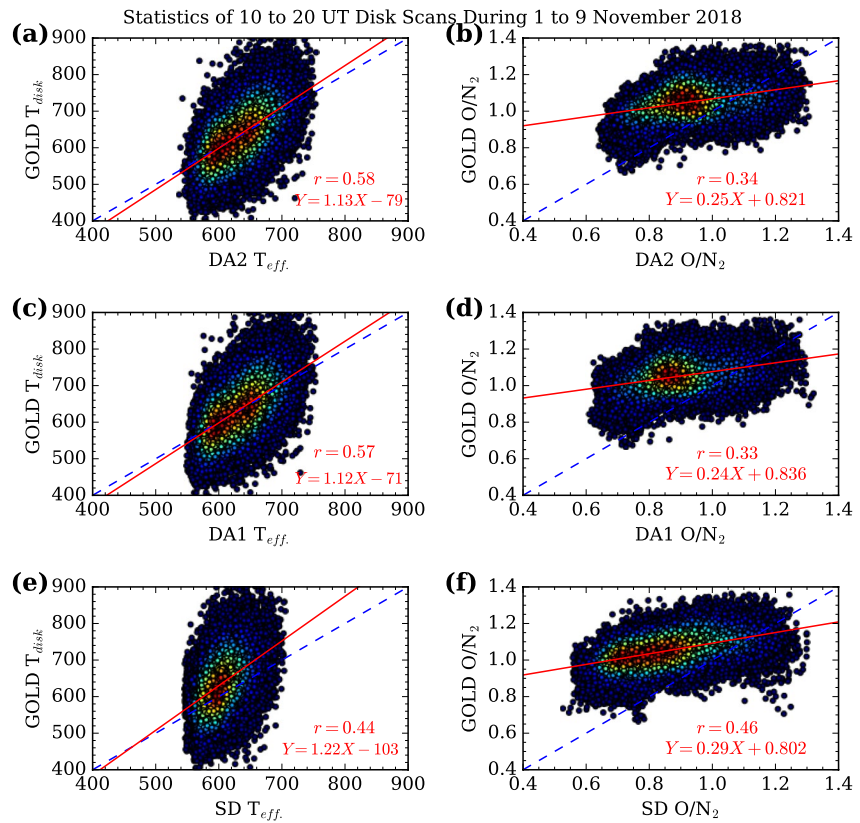
Figure 5. Scatter diagram of the Global-scale Observations of Limb and Disk (GOLD) T_{\text{disk}} and O/N_2 compared to their DA2, DA1, and SD equivalents are shown. For this analysis all the disk scans between 10 and 20 UT during 1–9 November 2018 are used. The red regions in the scatter diagram represents highest density points. For the GOLD versus DA2 the highest density points distribute around the one-to-one line (dashed), particularly for the temperature. The comparisons with respect to SD for both temperature and O/N_2 , on the other hand, are not as good.
