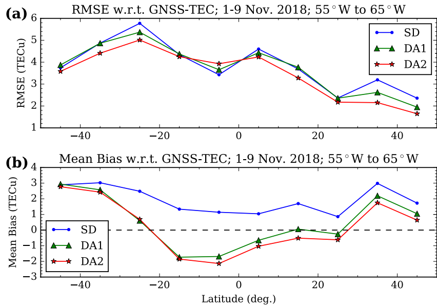
Figure 8. (a) Latitudinal variability of root mean square error (RMSE) and (b) mean bias for SD (blue), DA1 (green), and DA2 (red) with respect to Global Navigation Satellite System Total Electron Content during 1–9 November 2018 are shown. Clearly, for the DA2 the RMSE is smaller compared to other two cases and bias is closer to zero.
