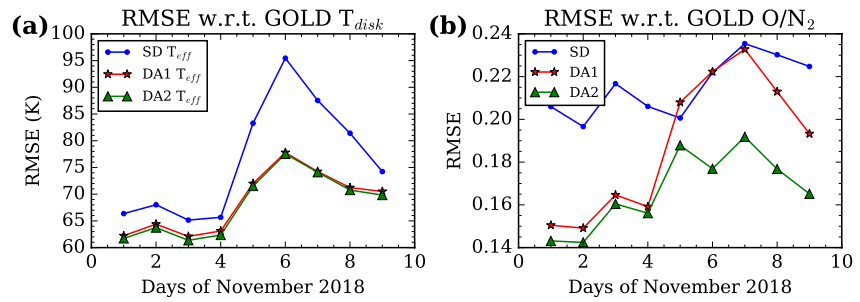
Figure 4. The root mean square error (RMSEs) in DA1 T_{\text{eff}} and DA2 T_{\text{eff}} with respect to Global-scale Observations of Limb and Disk T_{\text{disk}} are shown in (a) and similar RMSEs in O/N_2 are shown in (b). Note that the temperature RMSEs in the two DA runs, are clearly smaller than the SD. Also, the average O/N_2 RMSEs are better for the two assimilation runs compared to the SD, and DA2 has the best RMSE.
