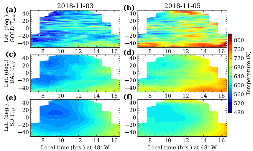
Figure 2. Local time and latitude variation of the Global-scale Observations of Limb and Disk T_{\text{disk}} compared with T_{\text{eff}} from DA1 (DA1 T_{\text{eff}} ) and specified dynamics-Whole Atmosphere Community Climate Model with thermosphere-ionosphere extension (SD T_{\text{eff}} ).
