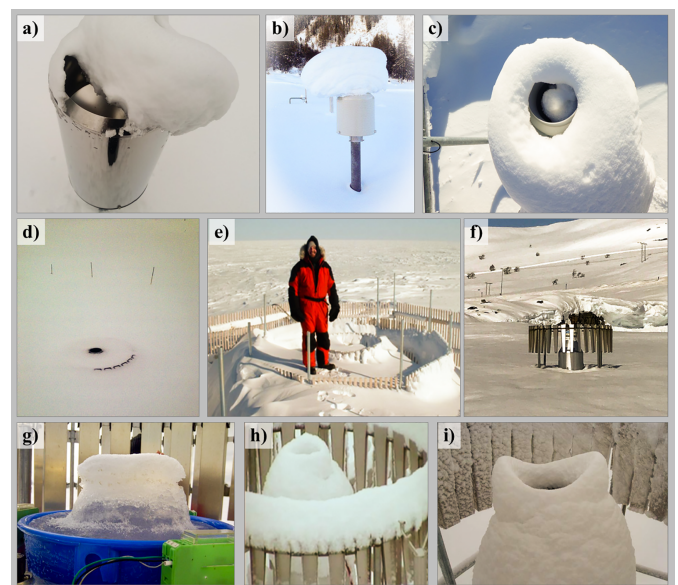
Fig. 6. Photos of common solid precipitation measurement issues, such as (a),(b),(c),(h),(i) fully or partially capped gauges; (d),(f) buried gauges; (e) shields that have accumulated drifting snow; (g) gauges with frozen bucket contents; and (h),(i) shields that have accumulated snow.
