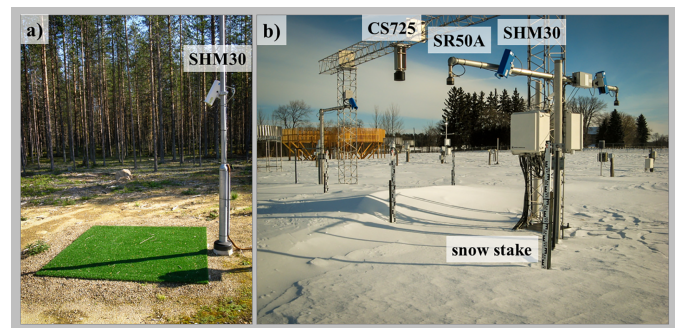
Fig. 8. Photos of snow depth sensor installations under assessment during SPICE: (a) an optical sensor (Lufft/Jenoptik SHM30) at Sodankylä prior to snow accumulation on a surface target constructed from artificial turf; (b) optical (Lufft/Jenoptik SHM30) and ultrasonic (Campbell Scientific SR50A) snow depth sensors concurrently measuring the same target area at CARE alongside manually observed graduated snow stakes used as the reference, and a Campbell Scientific CS725 passive gamma snow water equivalent sensor.
