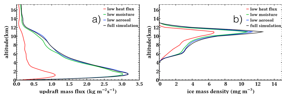
Figure 14. Profiles from four pyroCb model simulations showing the averaged vertical distributions of the (a) spatiotemporally averaged updraft mass fluxes and (b) ice mass densities. See text for descriptions of the four simulations.
