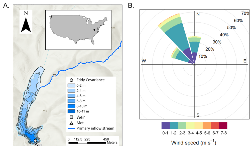
Figure 1. (a) Map of Falling Creek Reservoir located in Vinton, Virginia, USA (map inset) showing location of the eddy covariance system, the weir located on the primary freshwater inflow, and the meteorological station located on the dam. (b) Wind rose showing the dominant wind direction and wind speed ( \text{m s}^{-1} ) of greenhouse gas fluxes retained for analysis. The cumulative footprint distribution for the study period is shown in Supporting Information S1 (Figure S2).
