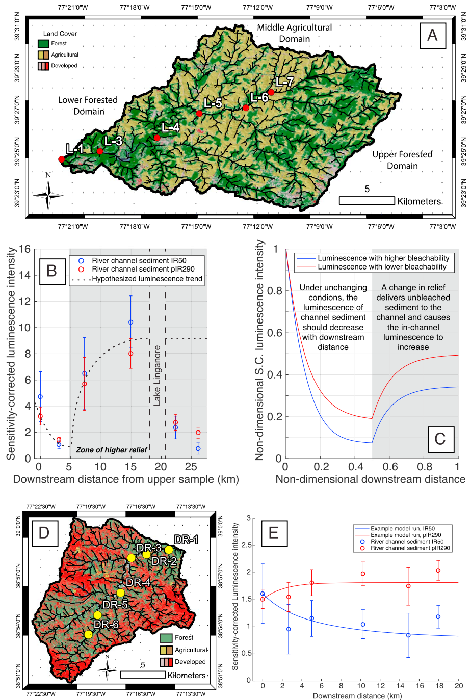
Figure 2. (a) Map of the Linganore Creek, MD, catchment showing land cover and drainage network. (b) Measurements of the in-channel sensitivity-corrected luminescence for Linganore Creek. Circles show the average sensitivity-corrected luminescence intensity taken from large aliquots; bars indicate the standard error. Gray zone shows area of higher-relief forested land cover. The black dashed line shows hypothesis of luminescence trend based on panel c. (c) Hypothesized behavior of luminescence at Linganore Creek. (d) Map of Difficult Run, VA, showing land cover, sample locations, and drainage network. Note high concentration of developed land use. (e) Field data results. The data show little to no change with downstream distance. We interpret this as an indication that human activity on sediment transport can obscure the natural signal by channel modification and construction/development runoff. Lines show example of possible model fits.
