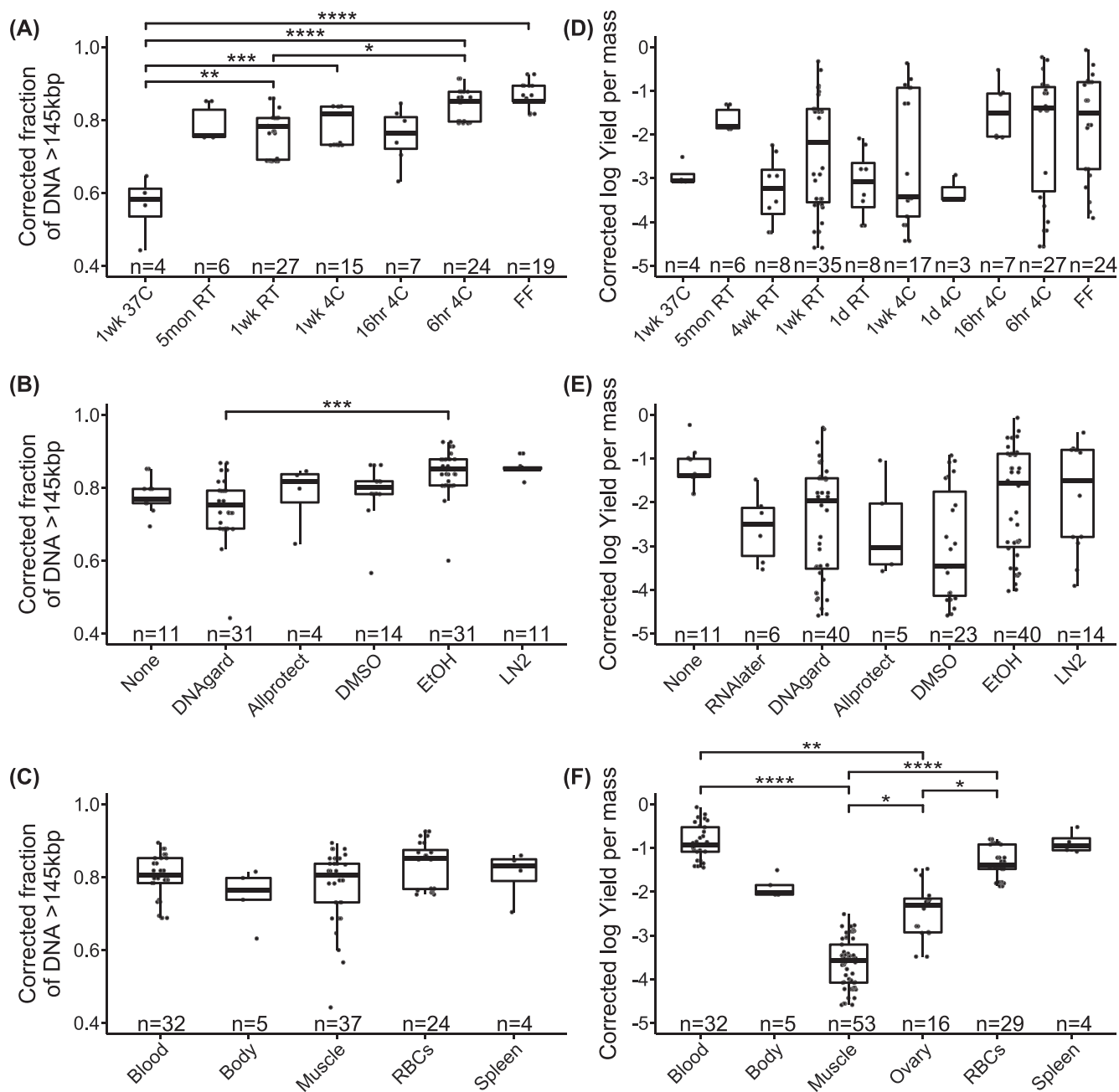
Figure 3: Testing the effect on two measures of uHMW DNA quality. Distributions of sample groups are overlaid with results of linear modeling of fragment length ( n = 102 , A–C) and DNA yield ( n = 139 , D–F). Shown are univariate scatterplots overlaid with box plots indicating the median, quartiles, and full range of individual observations. Fragment length was quantified here as the proportion of pulsed-field gel electrophoresis (PFGE) signal above 145 kb and was modeled in a generalized linear model with temperature (A), preservative (B), and tissue type (C) as predictors. DNA yield per input mass was log-transformed and modeled with temperature (D), preservative (E), tissue type (F), and vertebrate group as predictors. Significant relationships from post hoc comparisons are shown as connecting bars with significance levels: **** P < 0.0001 , *** P < 0.001 , ** P < 0.01 , * P < 0.05 . Sample sizes for each factor are given along the x-axis.
