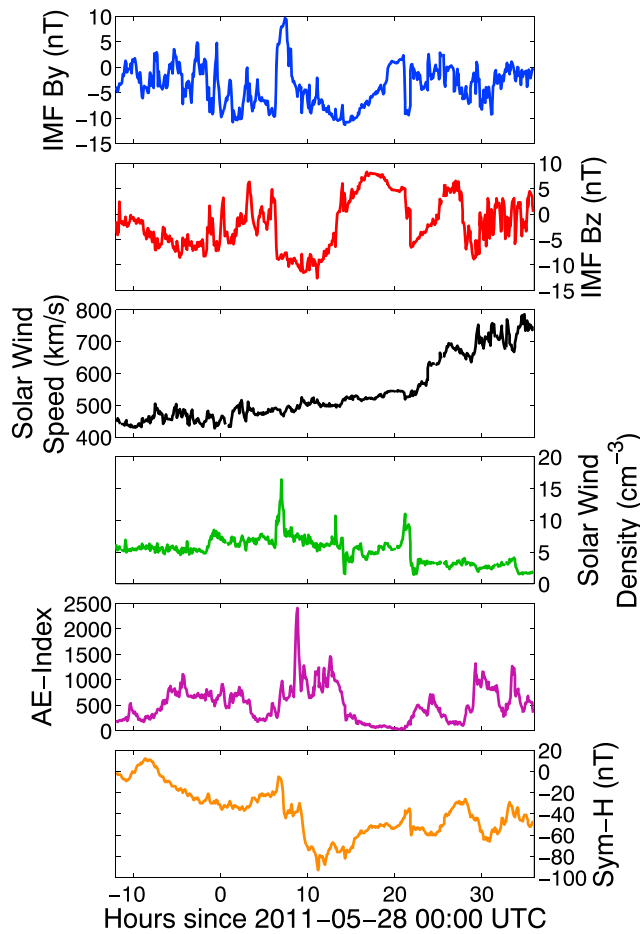
Figure 12. Interplanetary magnetic field (IMF), solar wind, AE index, and SYM-H around 28 May 2011 measured by satellites and magnetometers. Data are downloaded from OMNIWeb ( http://omniweb.gsfc.nasa.gov/form/omni_min.html ).
