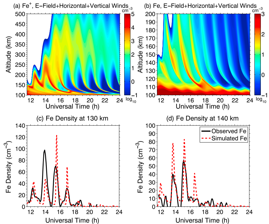
Figure 15. The same as Figure 13 except that the energy influx to the GLOW model is increased to 30 erg/s/cm 2 for this simulation.
