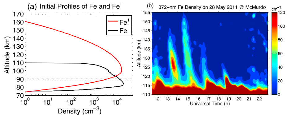
Figure 3. (a) Initial density profiles of Fe (black line) and Fe + (red line) used in the simulations of the thermospheric Fe layer event on 28 May 2011 at McMurdo, Antarctica. (b) Contour of thermospheric Fe densities from 110 to 155 km observed by lidar at McMurdo on 28 May 2011. Figure 3b is reproduced from Chu et al. [2011] for comparison to the TIFe model simulations.
