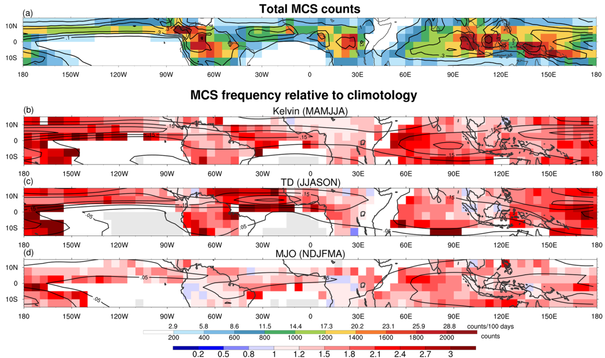
Figure 1. (a) MCS counts binned in 5^\circ \times 5^\circ grid boxes from 2001 to 2019. Each MCS is binned by its average lifetime location. Annual mean precipitation is contoured at 0.1 \text{ mm hr}^{-1} . (b–d) Frequency ratio ( R_{freq} , colors) of MCS occurrence relative to climatology when the calculation is conditioned on (b) Kelvin waves in MAMJJA, (c) TDs in JJASON, and (d) the MJO in NDJFMA. The mean standard deviation of wave-filtered rainfall in the respective months is contoured every 0.05 \text{ mm hr}^{-1} with zero lines omitted.
