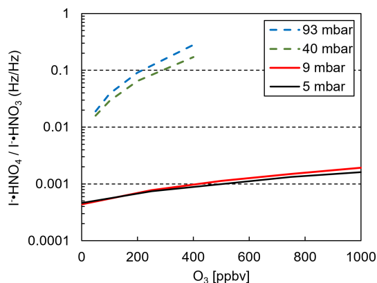
Figure 5. Ratio of I - •HNO 4 and I - •HNO 3 as a function of ozone mixing ratio of the sample gas. Solid lines: instrument described in this work operating at pressures indicated in the legend. Dashed lines: data from a standard I - -CIMS instrument operated at pressures indicated in the legend (40 and 93 mbar).
