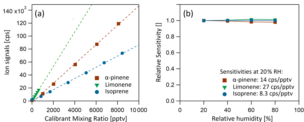
Figure 6. Calibrations in benzene mode. (a) Instrument response to selected biogenic calibrants (isoprene, C 5 H 8 ; α-pinene, C 10 H 16 ; limonene, C 10 H 16 ). (b) Sample humidity dependency of the calibrants.
