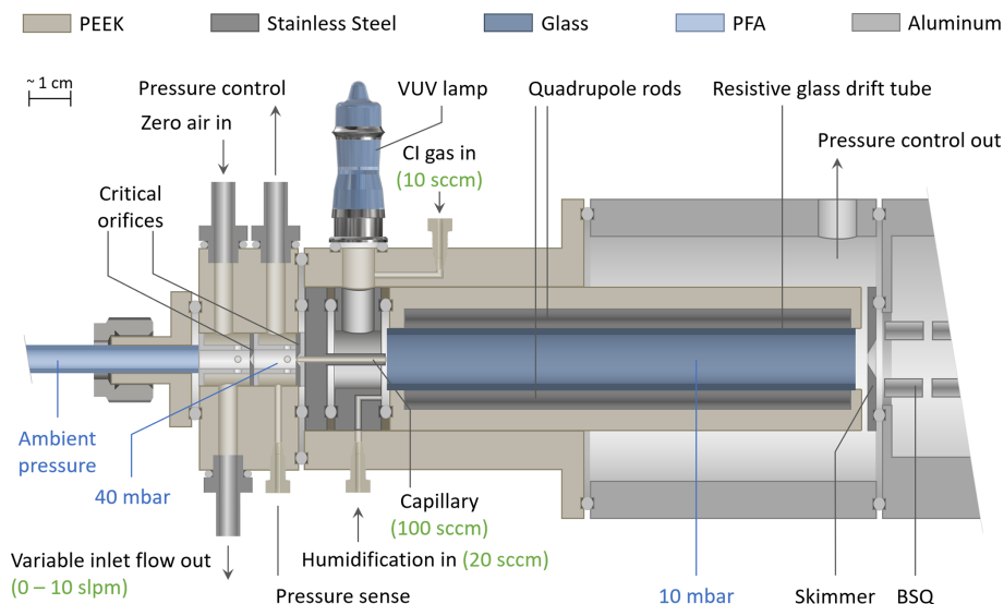
Figure 1. The VUV ion source coupled to the Vocus PTR-ToF-MS instrument. Note that only one VUV lamp is shown. Green numbers represent approximate typical flow rates.
