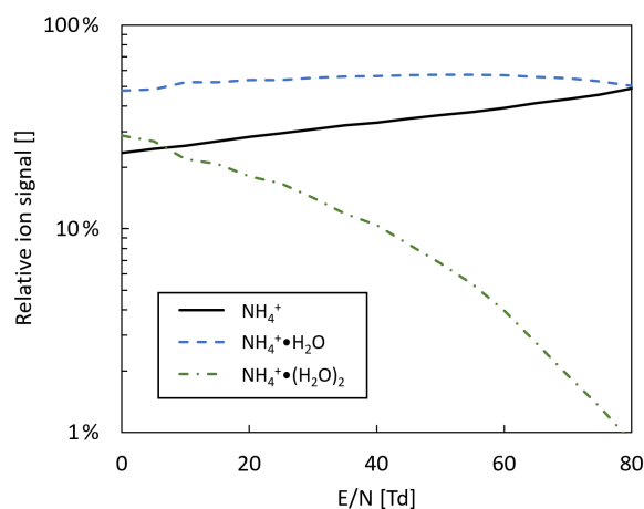
Figure 7. Reagent ion cluster distribution in ammonia mode as a function of reduced electric field ( E/N ). Drift tube pressure: 2 mbar; drift tube temperature: 60 °C.
