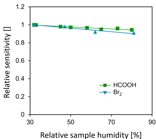
Figure 4. Relative sensitivities of formic acid (HCOOH) and bromine (Br 2 ) as a function of sample relative humidity (RH; T_{\text{ambient}} = 22\text{ }^{\circ}\text{C} , added H 2 O flow: 18 sccm). Sensitivities are normalized to the driest conditions (RH = 30 %).
