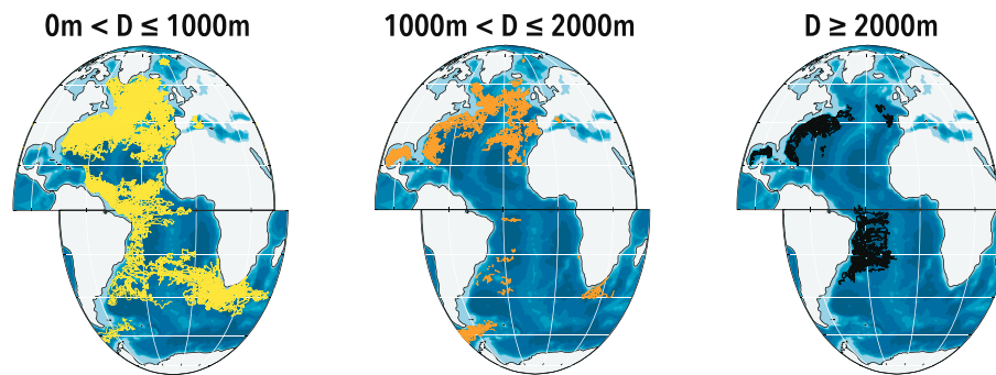
Figure 12. Subsurface float trajectories binned by depth, from left to right: 0–1,000 m; 1,000–2,000m; and 2,000m and deeper. Data source is the AOML PhOD subsurface drifter database, which currently houses all subsurface data collected through end of 2015 (Ramsey et al., 2018; https://www.aoml.noaa.gov/phod/float_traj/ ).
