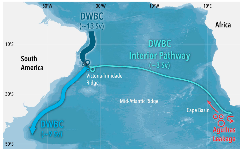
Figure 11. Schematic of North Atlantic Deep Water pathways in the South Atlantic as described by van Sebille et al. (2012) and Garzoli et al. (2015). The lower limb of the Atlantic Meridional Overturning Circulation (i.e. North Atlantic Deep Water) is shown in shades of blue, and some relevant pathways of the upper-limb Atlantic Meridional Overturning Circulation are shown in red. Bottom topography is shaded at 1,000-m intervals.
