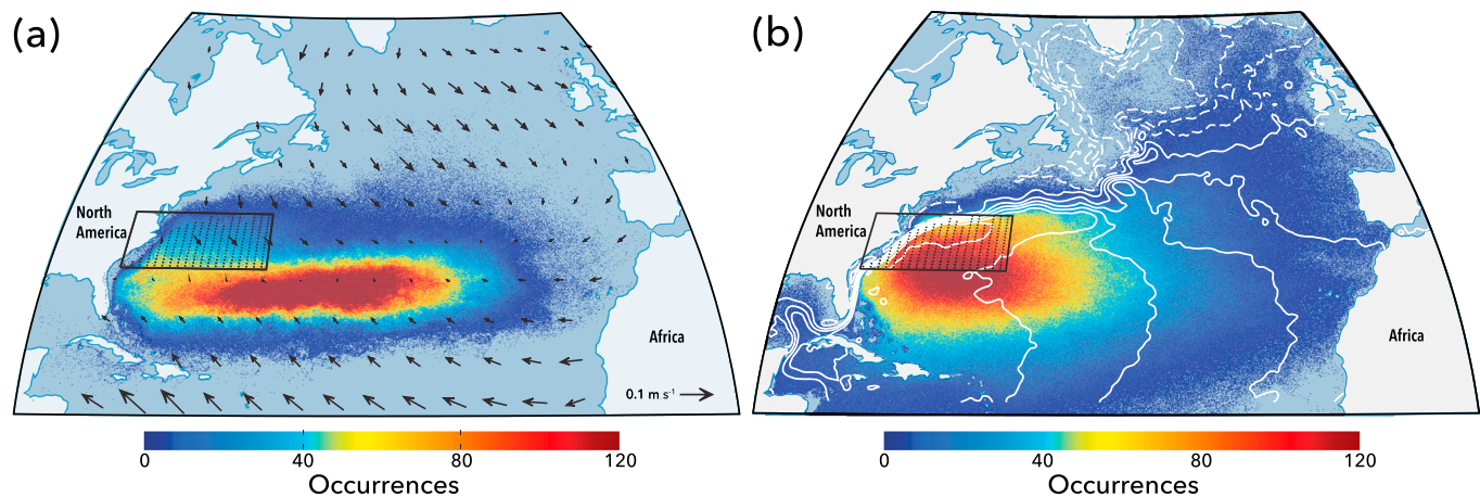
Figure 5. Distribution of modeled Gulf Stream waters. Fluid particle trajectories are initialized at the surface in the black box and integrated for 5 years in the 1/12^\circ FLAME model through either the (a) two-dimensional surface velocity field or (b) three-dimensional flow field. The colors refer to the number of times a particle passed through a given location over the 15-year model run. Less than 0.01% of the trajectories reach the subpolar gyre when restricted to the surface velocity field (a) and only 2.51% reach the subpolar gyre when allowed to follow the three-dimensional flow field (b) after 5 years. These results demonstrate the lack of a direct connection between the surface Gulf Stream and the subpolar gyre. Arrows in (a) indicate the time-averaged Ekman velocities over the North Atlantic, showing a convergence zone at 30^\circ\text{N} . Contours in (b) indicate the time-averaged SSH field over the North Atlantic, with positive values in solid contours and negative values in dashed contours. Figure adapted from Foukal and Lozier (2016).
