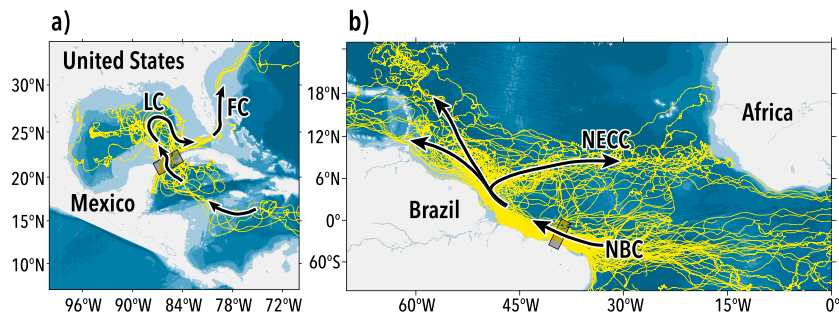
Figure 3. Select surface trajectories from the Global Drifter Program (GDP). The selection is for those drifters that pass through a given box (marked on each map), out of a block of 5,000 trajectories (data file for IDs 10001-15000 as distributed by the GDP). (a) Trajectories passing through a box in Yucatan Channel. The inflow from the east through the Caribbean and into the Channel, the Loop Current (LC), and finally the Florida Current (FC) are highlighted by arrows. (b) Trajectories in the North Brazil Current (NBC). The arrows show the inflow from the South Equatorial Current into the NBC, from where successive paths lead directly into the Caribbean, northward but east of the Caribbean, or retroflect into the North Equatorial Countercurrent (NECC). Flow from the North Equatorial Current is not shown. Bottom topography is shaded in 1,000-m intervals.
