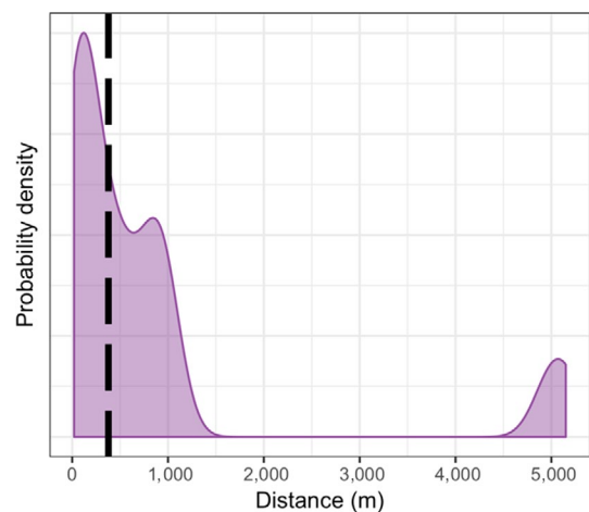
FIGURE 3 Estimates of distances between ploidy levels. Shaded region shows distributions of minimum distances; dashed vertical line indicates median [Colour figure can be viewed at wileyonlinelibrary.com ]
