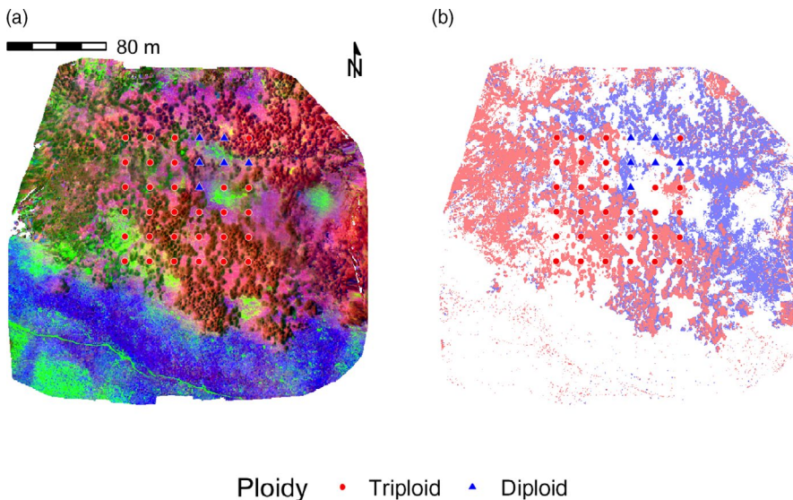
FIGURE 7 Example prediction of ploidy level from multispectral imagery for the Ben-Itha site. (a) False colour representation shaded according to scores from a principal component analysis (for visualization only) of all five spectral bands. (b) Spatial predictions of an ensemble of random forest classifiers, with canopy pixels shaded light red (triploids) or light blue (diploids). In both panels, georeferenced genetic samples are shown as red circles (triploids) or blue triangles (diploids) [Colour figure can be viewed at wileyonlinelibrary.com ]
