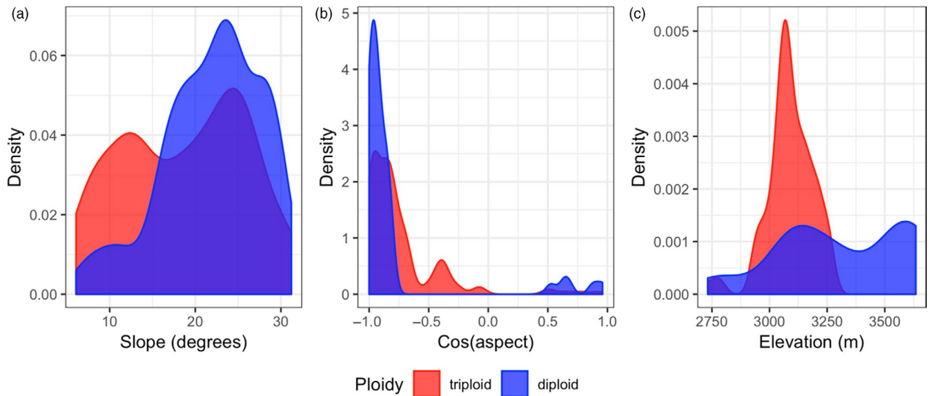
FIGURE 2 Distribution of ploidy levels across topographical gradients of (a) slope, (b) cosine aspect ( -1 = south-facing, 1 = north-facing) and (c) elevation [Colour figure can be viewed at wileyonlinelibrary.com ]
