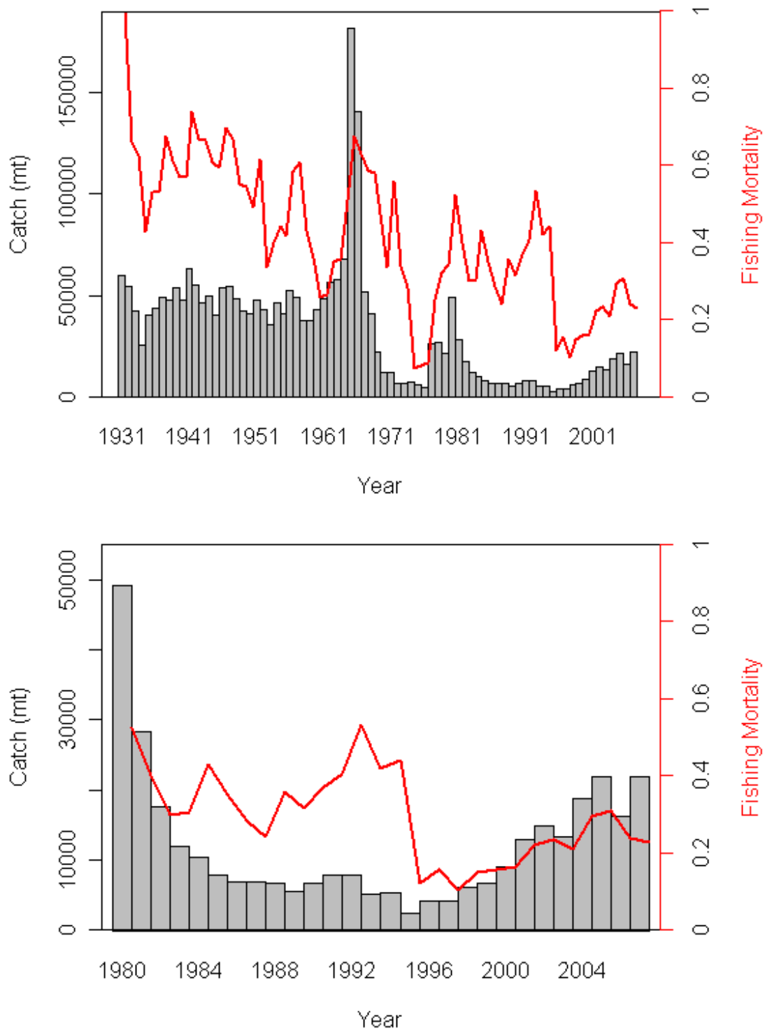
Figure B9. Total catch (mt) and VPA estimates of average fishing mortality on ages 5-7 for Georges Bank haddock.
