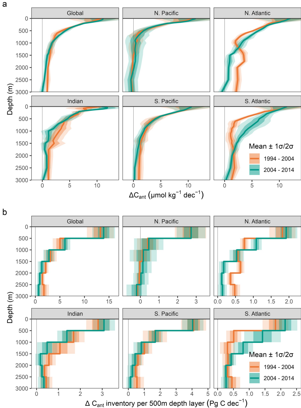
Figure 4. Mean vertical distribution of the decadal changes in anthropogenic carbon ( \Delta C_{ant} ) for the global ocean and both hemispheres of the main ocean basins: (a) mean content profiles and (b) 500-m-depth layer inventories of \Delta C_{ant} . Colors distinguish the decades 1994–2004 and 2004–2014. Thick lines represent the standard case reconstruction of \Delta C_{ant} and ribbons indicate the 1\sigma - and 2\sigma -uncertainty ranges.
