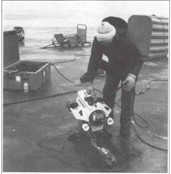
Figure 9. Remotely operated vehicle (ROV) used in cooperative GLERL/U.S. Fish and Wildlife pilot studies of under-ice ecology. The large lakes winter ecology program provides increased knowledge of climate variability and global change.
