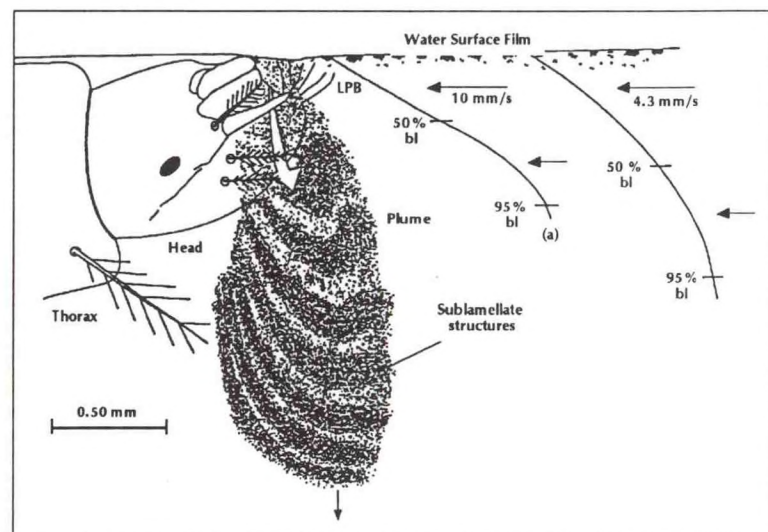
Figure 6. Lateral view of interfacial feeding Anopheles larva with India ink particles in the surface microlayers. Results of high-speed movies like these show that the food is selected in a microlayer below the surface film, concentrated in the mouth, and the "filtered" water is pushed below the animal. The plume with distinct lamellae demonstrate that the flow is laminar.
