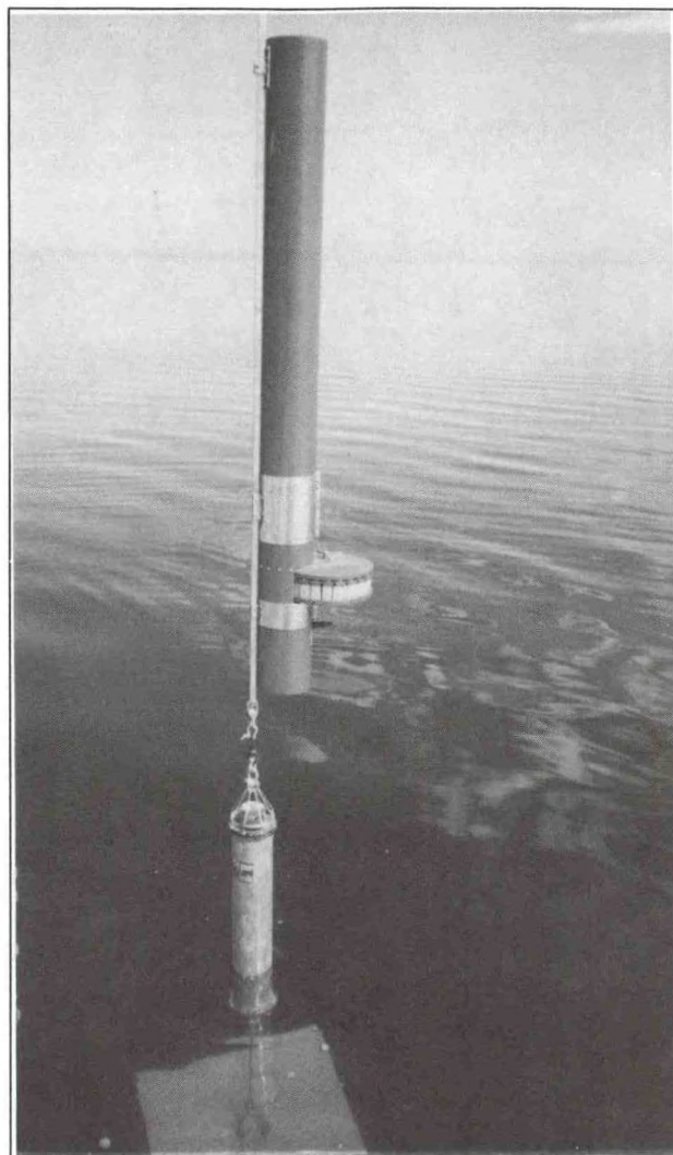
Figure 18. The GLERL-designed sequential sediment trap ready for deployment in Lake Michigan.
