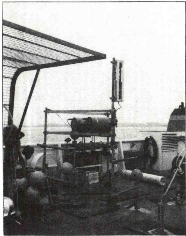
Figure 17. An instrument tripod for monitoring sediment resuspension. Water transparency is measured by the two transmissometers - one is in the cage on the vertical pipe and the other is suspended below the tripod. Current velocity is measured by the two current meters attached to the tripod legs. The two pressure cases contain the data acquisition system and the power supply.
