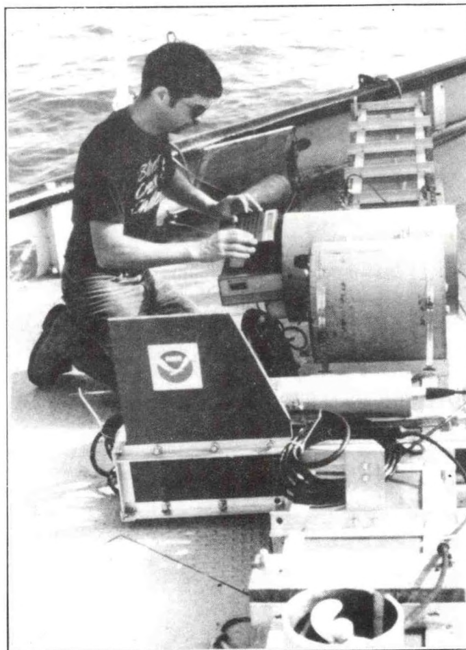
Figure 9. A bottom-resting flume used to determine the velocity required to initiate sediment resuspension. Water is pulled through the flume by the propeller located at the bottom of the picture. The small cylinder just behind the sail contains the electronics for a small electromagnetic current meter used to measure the current velocity in the flume. The sail is attached to a cage which protects the transmissometer. This instrument, which is mounted in the side walls of the flume, measures the amount of sediment in suspension. The shorter pressure case contains the power supply while the longer one contains the data acquisition system. The sail is used to orient the flume perpendicularly to the ambient flow.
