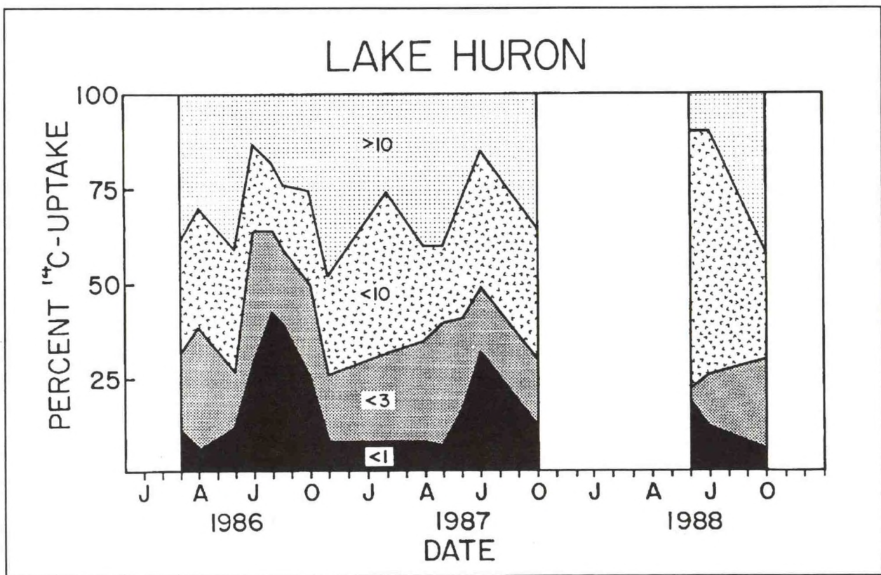
Figure 12. Seasonal variation of 14 C fixation by percent contribution of various size classes of phytoplankton in Lake Huron determined by filter fractionation.
