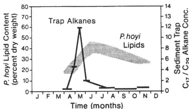
Figure 13. Seasonal total lipid content of P. hoyi averaged over 2 years of collection (data taken from Gardner et al. 1985; Landrum 1988; Gauvin 1989). Also shown is the ratio of the planktonic n-alkane C_{17} to the terrestrial n-alkane C_{29} . The April-June peak is a clear signal of autochthonous carbon input. The sediment value for this ratio is 0.2.
