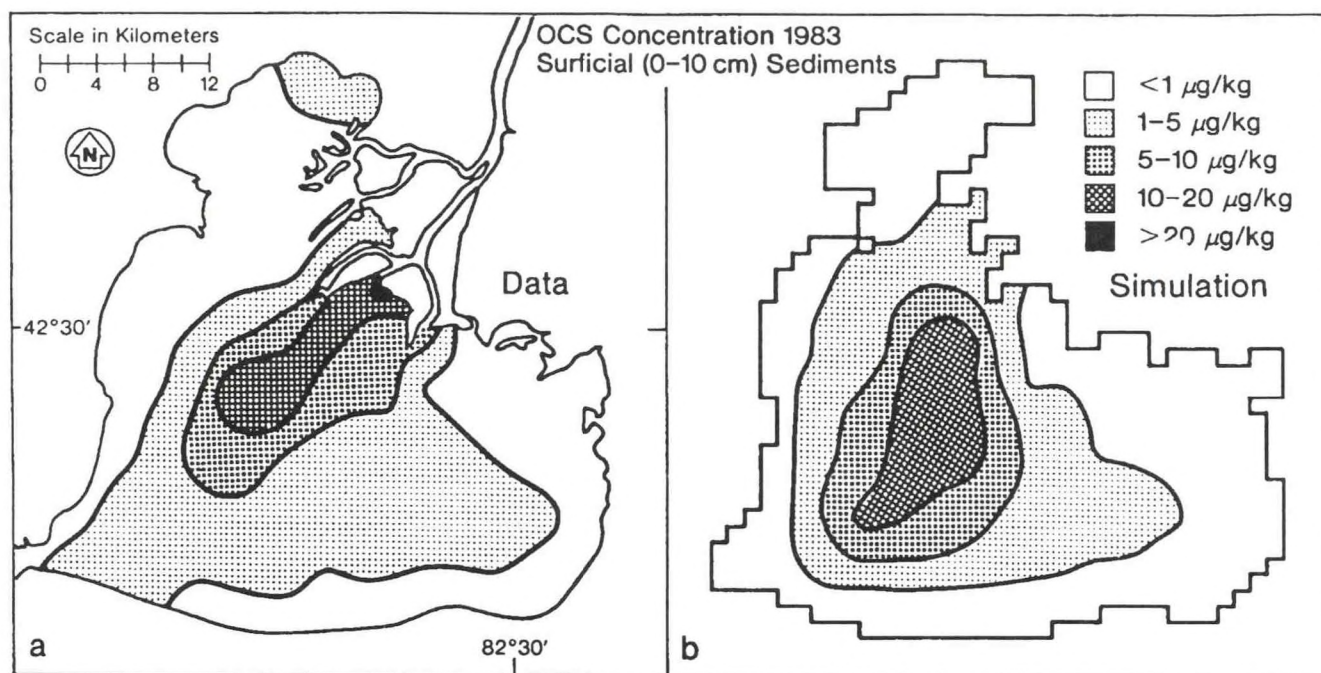
Figure 18. Comparison of observed (a) and model-simulated (b) concentrations of octachlorostyrene (OCS) in surface (0-10 cm) sediments of Lake St. Clair in 1983. Units in \mu\text{g kg}^{-1} . Model results indicate that from 1971-83, 3.8 MT of OCS entered the system, 2.8 MT were flushed from the lake through the Detroit River, 0.8 MT were lost due to biological degradation and volatilization, and 0.2 MT were deposited in the lake's sediments.
