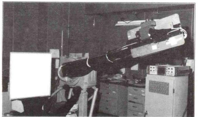
Figure 20. Barium sulfate panel mounted on five-axis positioner. The rotating boom, on which the detector is mounted, is shown at an angle approximately +20^\circ from normal to the panel.
