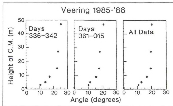
Figure 12. Currents veer counter-clockwise as the lake bottom is approached through an Ekman layer. The veering shown in this figure was observed during two high speed current outbreaks that lasted for durations of 7 and 20 days. These measurements are compared with the average veering observed for a six-month-long current meter (C.M.) deployment in the winter of 1985-1986.
