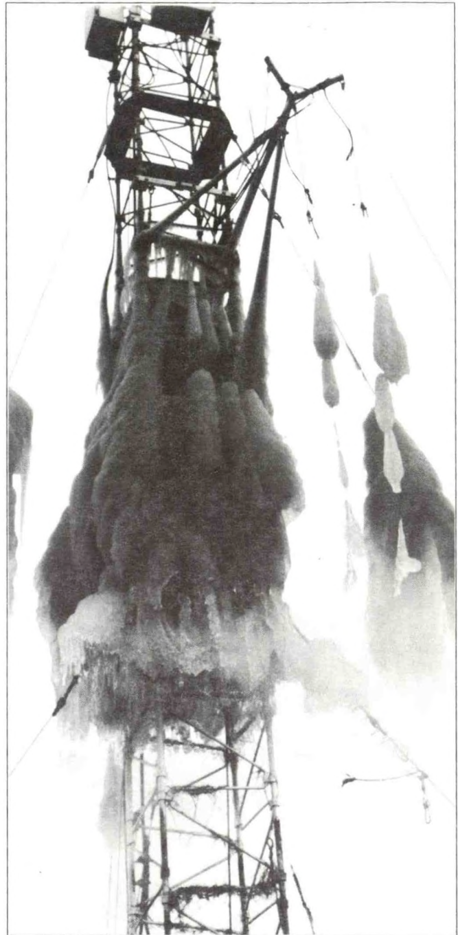
Figure 19. A wave tower used on Lake St. Clair during the GLERL–NWRI study on wave processes. Ice formed on the tower before it was retrieved December 1986.
