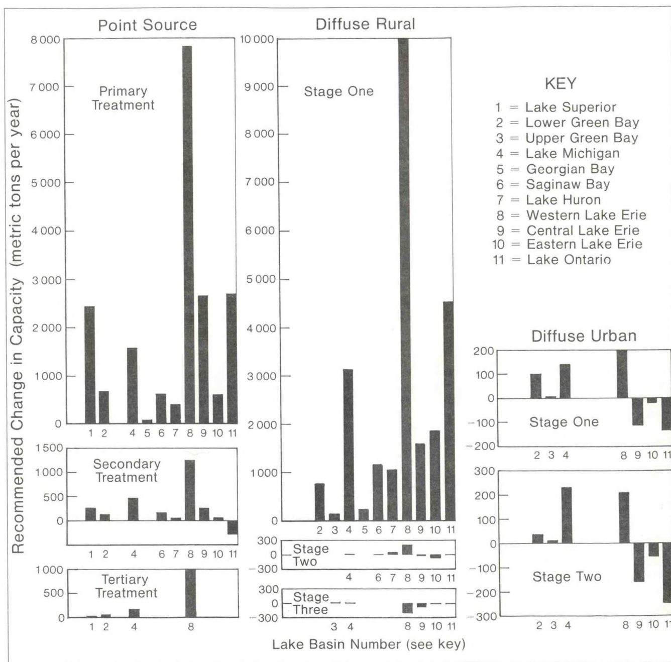
Figure 33. Recommended changes in treatment capacities in order to achieve a 100 percent probability of attaining desired phosphorus concentrations in the 11 basins. Changes recommended are relative to those capacities suggested in the 1978 IJC agreement.
