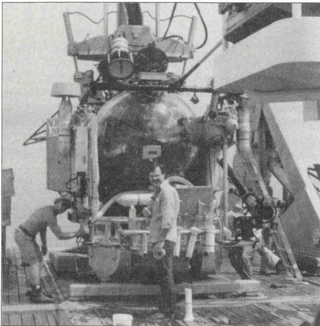
Figure 18. The Johnson Sea-Link was used during 1985 for a NOAA-sponsored exploration of Lake Superior using a research submersible. This marked the first time man has explored the greatest depths of Lake Superior first hand.
