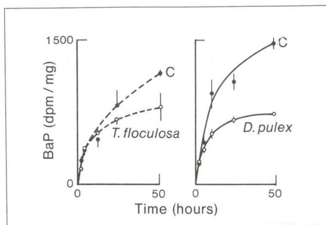
Figure 5. Uptake by Mysis relicta of BaP from contaminated water (line C) and two food-water combinations. The food sources used were the algae Tabellaria flocculosa (left) and the zooplankton Daphnia pulex (right).
