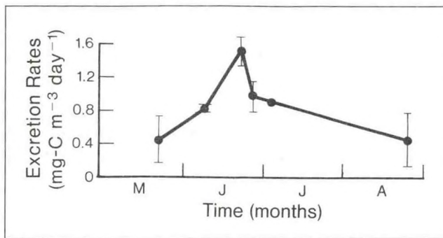
Figure 10. Release of dissolved organic carbon by algae in 1984 as measured by accumulation of ^{14}\text{C} in 0.22- \mu\text{m} filtrate after short-term incubations.
