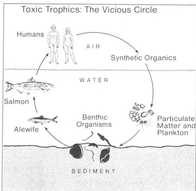
Figure 1. A conceptual representation of the cycling of trace contaminants in the Great Lakes and the closed-loop relationship to human beings.
