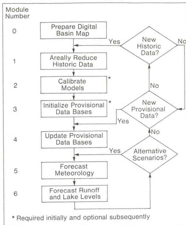
Figure 22. Conceptual logic flow chart for making water supply outlooks for a large lake. Typically, modules 0, 1, 2, and 3 are performed only infrequently on a large computer in order to prepare the models, data, and data bases for use with modules 4, 5, and 6 on other, perhaps smaller, computers in the forecast office. Modules 1–3 may be repeated as new historic data becomes available every 2 to 3 years; module 4 is repeated as new provisional data becomes available from the field in near-real-time every day or week; and modules 5 and 6 are repeated as new water supply outlooks are desired.
