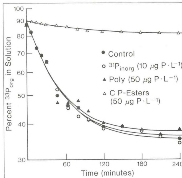
Figure 14. Results of a multiple substrate addition experiment showing that phosphorus-containing radiolabeled organic compounds ( ^{33}\text{P}_{\text{org}} ) produced by algae are rapidly taken up by heterotrophic bacteria in Lake Michigan. Uptake of ^{33}\text{P}_{\text{org}} is unaffected by additions of inorganic phosphate ( ^{31}\text{P}_{\text{inorg}} ) and condensed inorganic polyphosphate (Poly) but is severely reduced when phosphorus-containing carbohydrate esters (C-P-Esters) are added. This shows that bacteria utilize the organic rather than the inorganic dissolved phosphorus pool.
