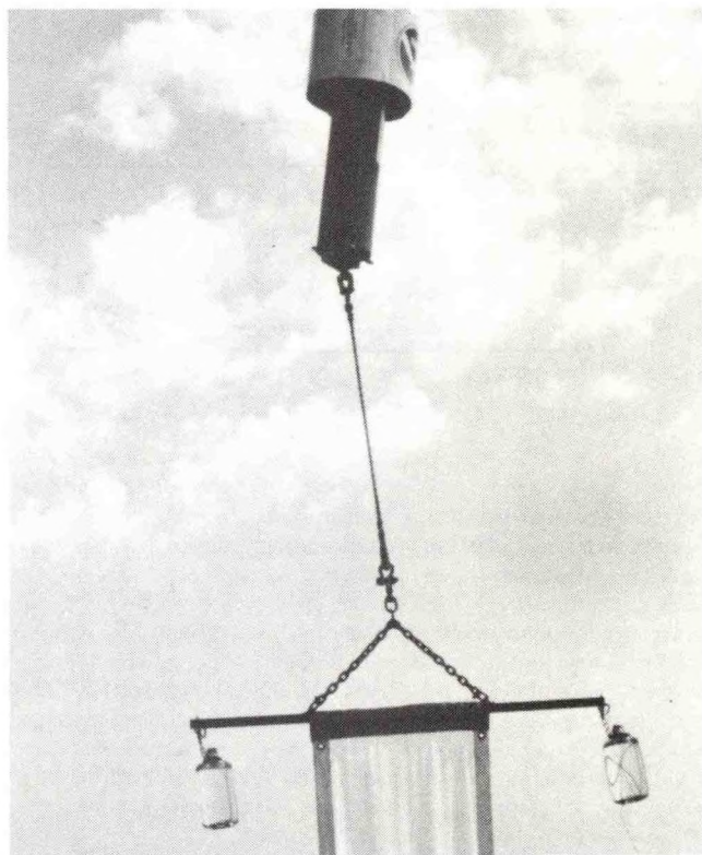
Satellite-tracked drifter buoy with attached window-shade drogue and bottles containing phytoplankton and lake water samples. This instrumentation was used to gather data for the phytoplankton growth part of the Lake Michigan Ecosystem Experiment.
