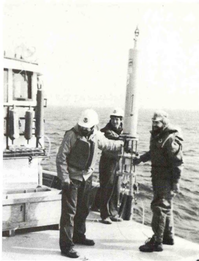
Vector averaging current meter. The marine instrumentation laboratory deployed 36 current meters this past year, including 4 in the St. Clair and Detroit Rivers and this one in Lake Michigan. The work done by this group in maintaining and calibrating current meters and other instruments is vital to the success of field experiments.
