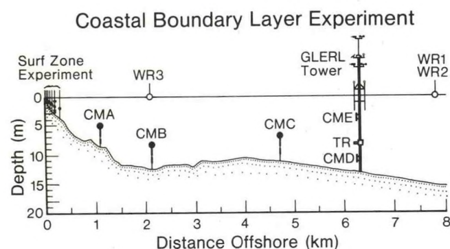
Cross section of the Coastal Boundary Layer Experiment instrument array. CMA-E represent the five vector averaging current meters, WR1-3 are Waverider buoys, and TR is a transmissometer, an instrument for measuring water transparency. In addition, there were four Zwartz wave gauges mounted on the solar-powered tower to record directional wave information and mean water level and meteorological instruments to measure wind velocity and direction.
