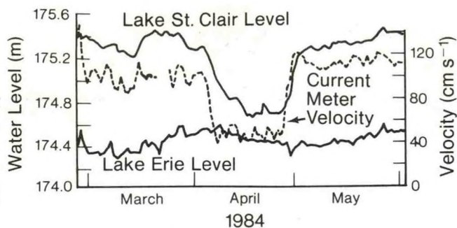
Lake St. Clair and Lake Erie water levels (in meters) and current-meter velocities (in centimeters per second) for March through May 1984. Note the low water levels in Lake St. Clair in April 1984 due to the ice jam in the St. Clair River.
