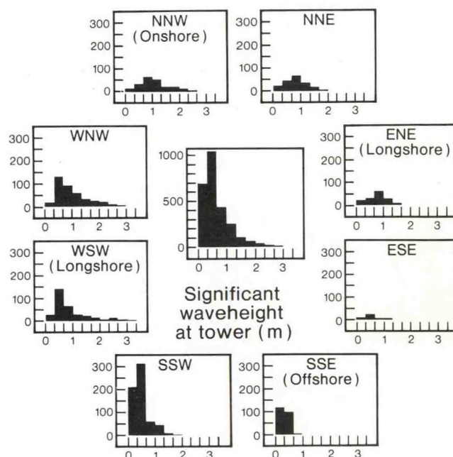
Histograms for significant wave height (in meters) for various wind directions at the GLERL tower deployed in Lake Erie during July-October 1981. These data were collected as part of the Lake Erie Coastal Boundary Layer Experiment. Data from that experiment have been used to examine the probability distributions for both deep and shallow water waves.
