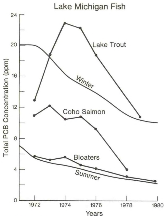
PCB's in Lake Michigan fish. The smooth lines are model output using maximum pollutant removal rates (summer) and minimum rates (winter). Fish data through 1978 are from the International Joint Commission; 1979 and 1980 data are from W. A. Wilford (personal communication, U.S. Fish and Wildlife Service, Ann Arbor).
