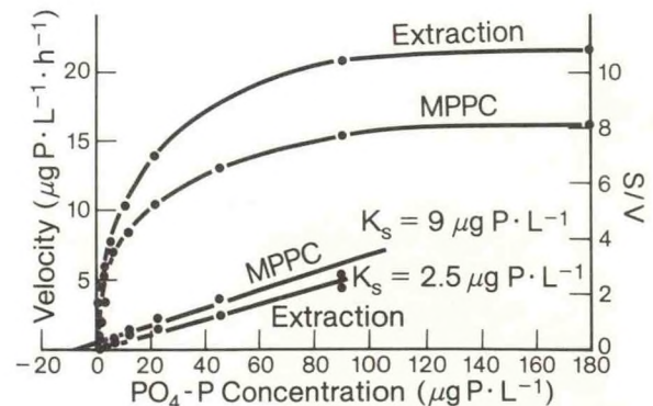
The kinetics of phosphate-phosphorus uptake by a mixed microbial population in Lake Michigan based on two estimates of ambient phosphate-phosphorus concentrations: chemical (extraction) and radioassay estimates of maximum possible phosphate-phosphorus concentrations (MPPC). The curved lines are the result of plotting the velocity of phosphorus uptake versus phosphate-phosphorus concentration. K_s (the affinity of microorganisms for phosphate-phosphorus) is obtained by linear transformation, that is, plotting the phosphate-phosphorus concentration divided by the velocity ( S/V ) versus the phosphate-phosphorus concentration and extrapolating through the negative y axis. The negative sign is dropped by convention.
