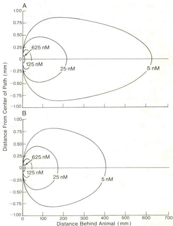
Contour diagrams for the steady-state plume of phosphorus, in nanomoles per liter, (A) behind a swimming Daphnia pulex and (B) with algal uptake of phosphorus included.
