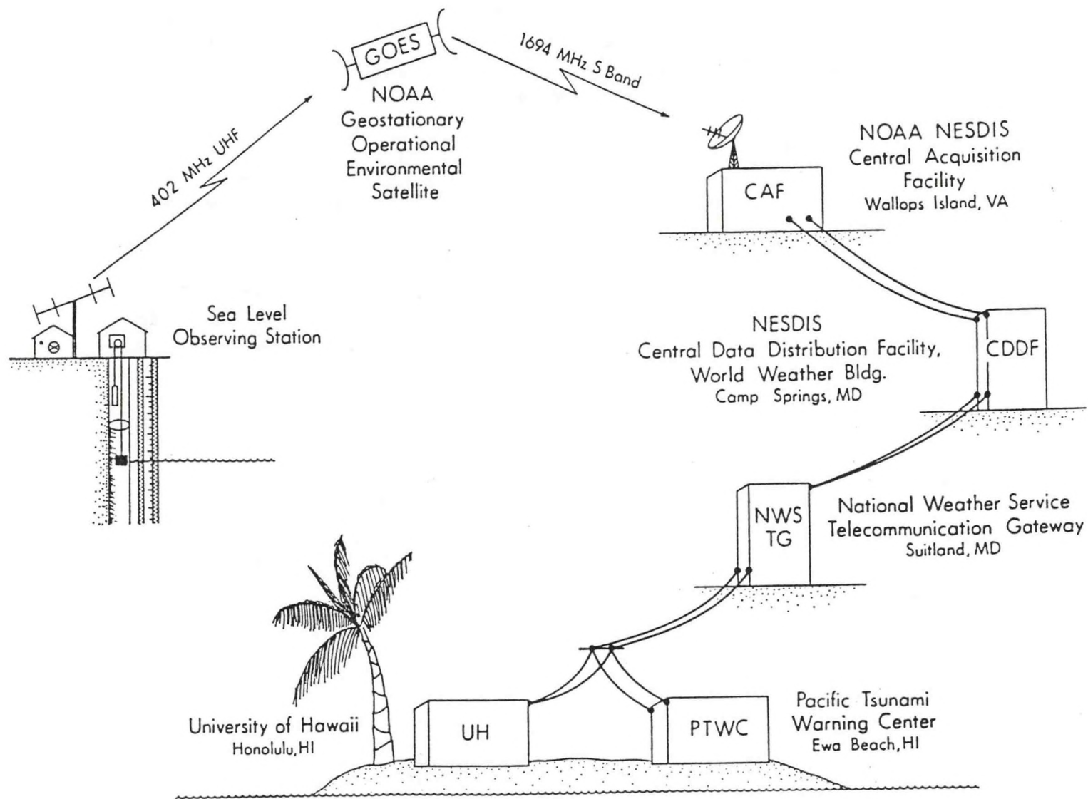
Satellite data transmission pathway for stations within the Pacific Sea Level Network.
