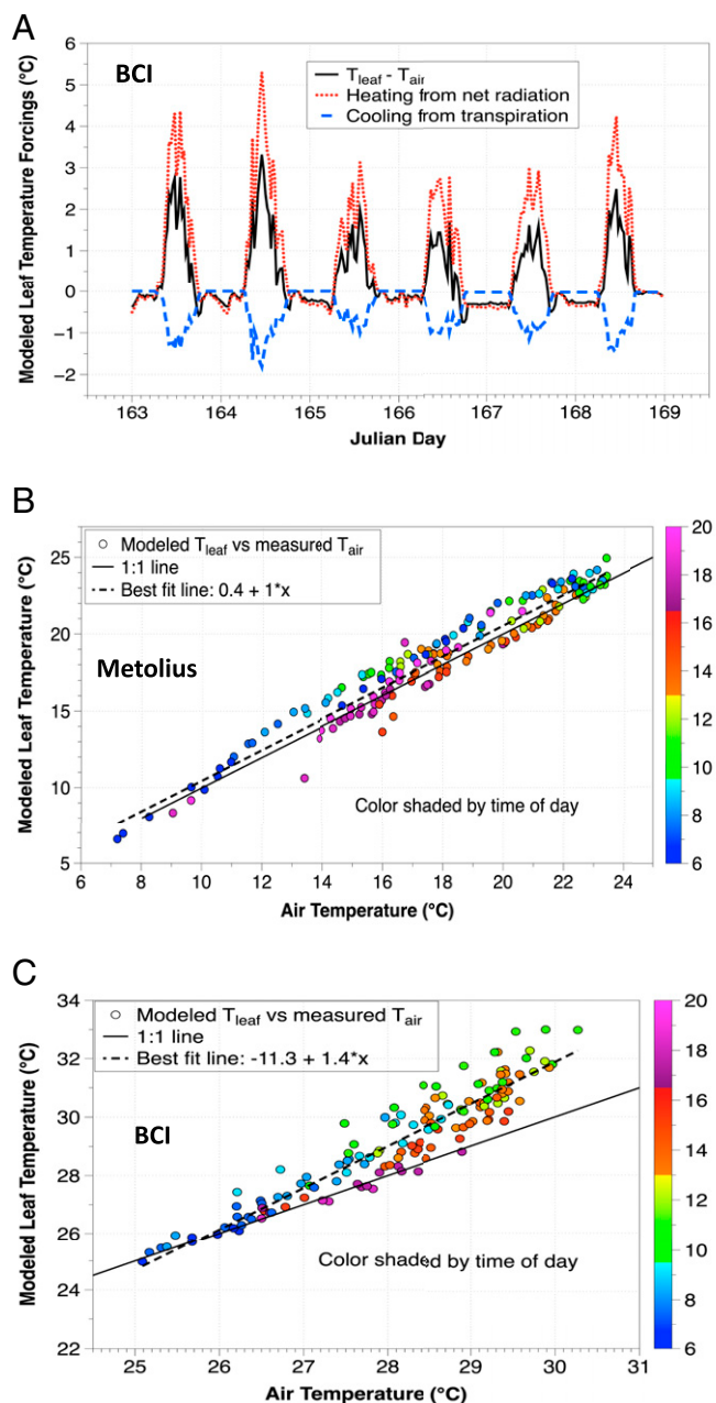
Fig. 5. Modeled T_{leaf} - T_{air} (black solid line), leaf heating from R_{net} ( W m^{-2} , red dotted line), and leaf cooling from transpiration (blue dashed line) at BCI (in °C) shown in (A). A typical example of a 6-d summer period for modeled T_{leaf} versus measured T_{air} (both °C) at Metolius (B) and BCI (C) for representative rain-free periods (May 25–June 1, 2015 and June 12–18, 2015, respectively). Color shading is by hour of day.
