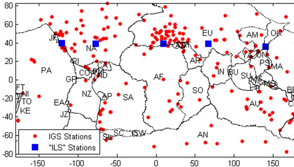
Fig. 3 Circles and squares depict the 231 core stations defining the IGS08 geodetic frame. The closest IGS stations to the old ILS astronomical observatories are represented by squares
