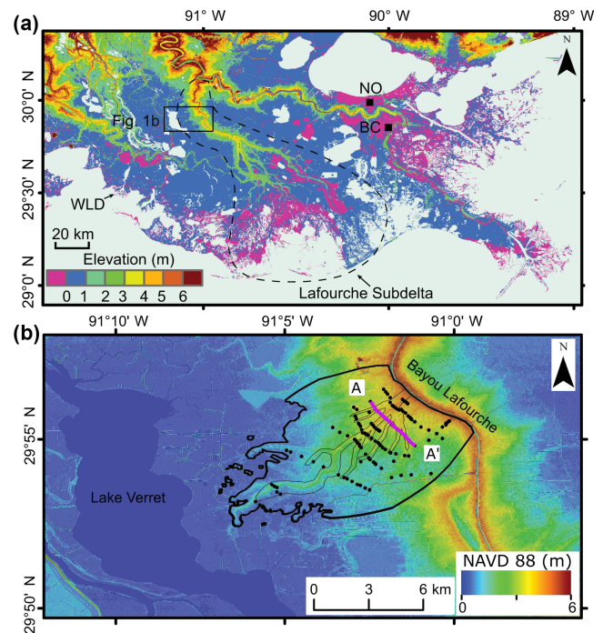
Figure 1. Digital elevation models (DEMs) of the study area. (a) Mississippi Delta, Louisiana, USA. Regional data are derived from the 1/3 arcsec DEM of the US Geological Survey ( http://viewer.nationalmap.gov/basic/#startUp ), accessed in September 2015. (b) The Attakapas Crevasse Splay at Napoleonville, Louisiana. Black dots mark core locations. The surface expression of the silty splay deposit used in the 3-D model is marked by the thick black line. Thin black lines show alluvial ridges associated with splay channels. The local DEM is derived from light detection and ranging data available from Atlas: The Louisiana State GIS ( http://atlas.lsu.edu ). NO – New Orleans; BC – Belle Chasse; WLD – Wax Lake delta; NAVD 88 – North American Vertical Datum of 1988.
