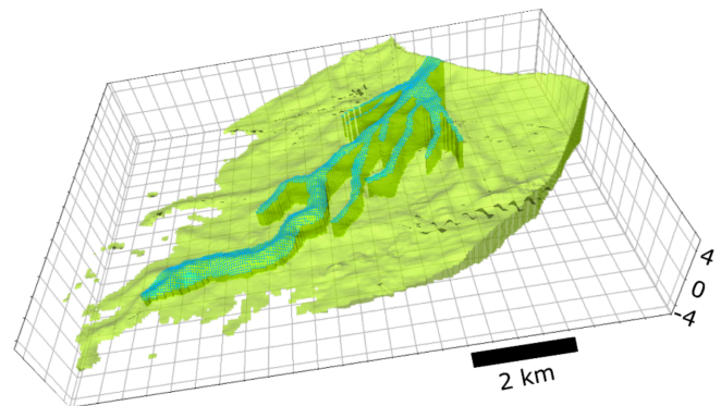
Figure 3. 3-D geometry of the Attakapas Crevasse Splay. Vertical axis is in meters relative to NAVD 88. The relatively sandy channel deposits are shown in blue green; light green refers to the silt-dominated portion of the splay. Channel deposits make up 16% of the total volume, and non-channel deposits compose the remaining 84%. The transparent top bounding surface is the lidar-derived modern land surface, and the base is the clay to silt transition shown in Fig. 4. Wherever possible, the lateral boundary is chosen to be the intersection of the top and basal bounding surfaces. On the lateral edges, where the deposit does not pinch out and these two surfaces do not meet, the boundary was chosen manually.
