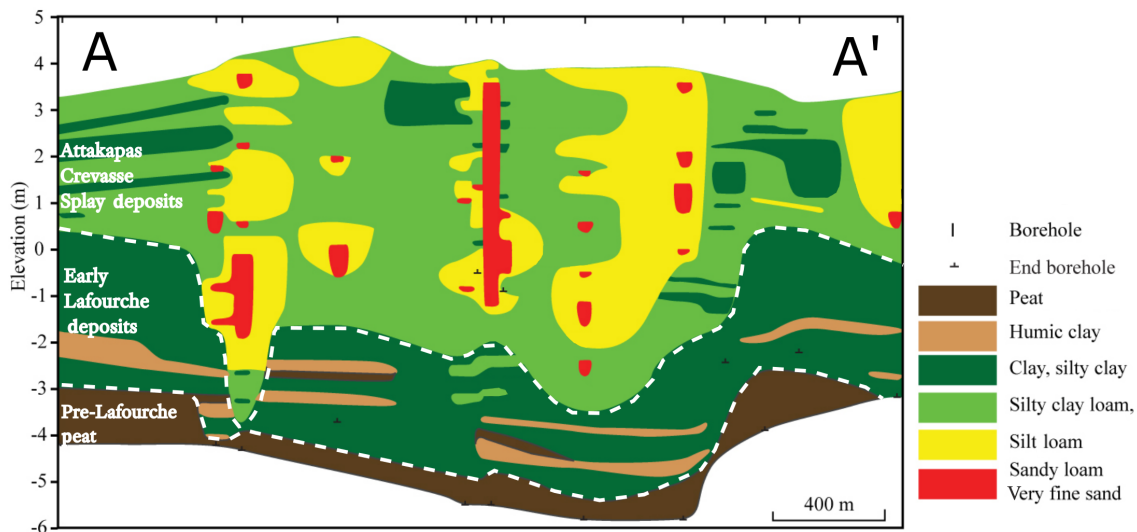
Figure 4. Stratigraphic cross section along transect A to A' (see Fig. 1b for location), adapted from Shen et al. (2015). Our 3-D model (Fig. 3) considers only sediments preserved above the clay to silty clay loam transition. Channel bodies can be seen as deposits of coarser material, often corresponding to alluvial ridges.
