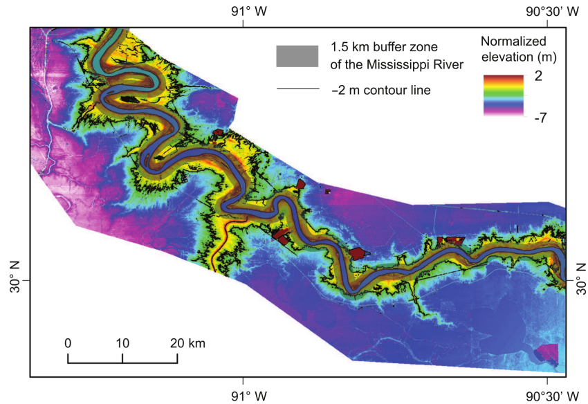
Figure 2. Normalized DEM of the LMR between Baton Rouge and the Bonnet Carre Spillway and the adjacent portion of the delta plain for crevasse splay identification. The DEM was obtained by subtracting a planar surface that best fits the Mississippi River natural levee long profile from the DEM of the studied reach. A -2 m contour of the normalized DEM and a 1.5 km buffer zone around the centreline of the MR are used to identify crevasse splays. The area where the -2 m contour lies outside the buffer zone is identified as formed by a crevasse splay (see Shen et al., 2015, for further explanation), which accounts for \sim 75\% of the bank length in the studied reach. Note the reduction in the extent of crevasse splays downstream of the avulsion site; this is likely due to the fact that the duration of channel activity upstream of this point was considerably longer than in the downstream reach.
