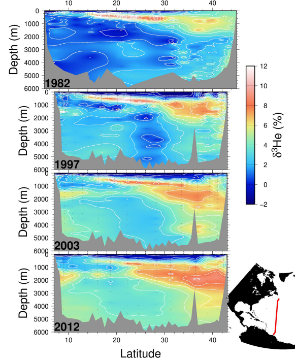
Figure 6. Four meridional \delta^3\text{He} sections along roughly 52^\circ W in the North Atlantic taken in 1982, 1997, 2003, and 2012. Contour intervals are 1 %, and measurement uncertainties are 0.15 %. Due to differences in cruise tracks, the topography for the 1982 occupation differs from the others.
