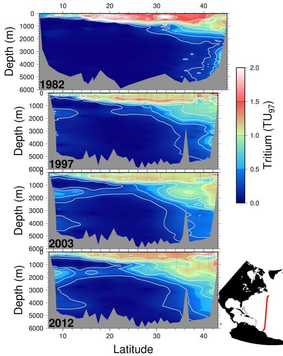
Figure 5. Four meridional tritium sections along roughly 52^\circ W in the North Atlantic taken in 1982, 1997, 2003, and 2012. The tritium concentrations have been decay-corrected to a common time (1 January 1997) for comparison. Contour intervals are 0.2 \text{ TU}_{97} , and measurement uncertainties are of order 0.01 \text{ TU}_{97} or better. Due to differences in cruise tracks, the topography for the 1982 occupation differs from the others.
