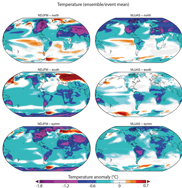
Figure 2. CESM spatial composite of surface temperature anomaly ( ^{\circ}\text{C} ) for (top row) ASYMM NH , (middle row) ASYMM SH , and (bottom row) SYMM events, each in (left column) NDJFM and (right column) MJJAS. Stippling indicates statistical significance using a two-sided Student's t test ( p < 0.05 ).
